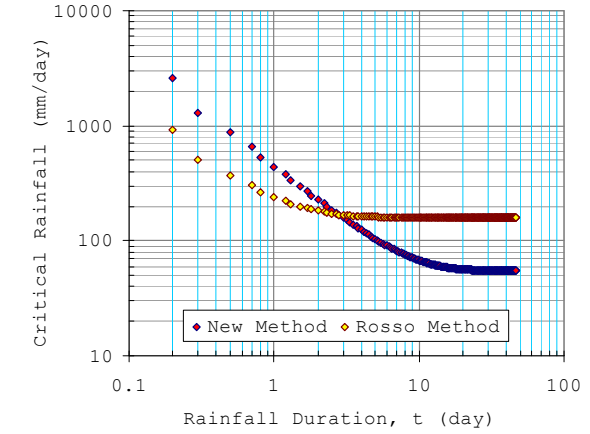
Fig. 5 The comparisons of predicted rainfall threshold for different rainfall duration role computed by the new method and the original approach.
