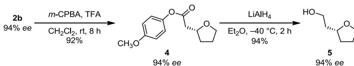
Scheme 1. Transformation of 2b .
