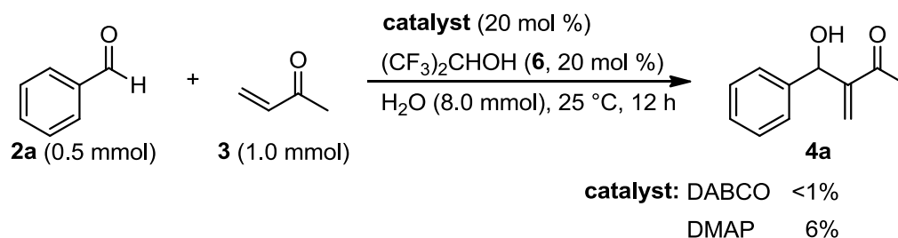
Scheme 3. MBH Reaction between Benzaldehyde ( 2a ) and Methyl Vinyl Ketone ( 3 ) Using DABCO and DMAP in the Presence of Water.
