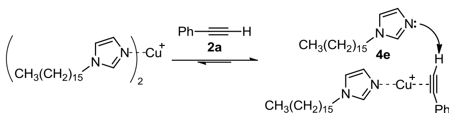
Scheme 3. Proposed Pathway of the Acceleration by 4e .
