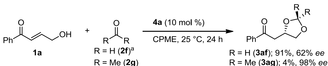
Scheme 4. Formal [3+2] Cycloaddition with Formaldehyde ( 2f ) and Acetone ( 2g ).
