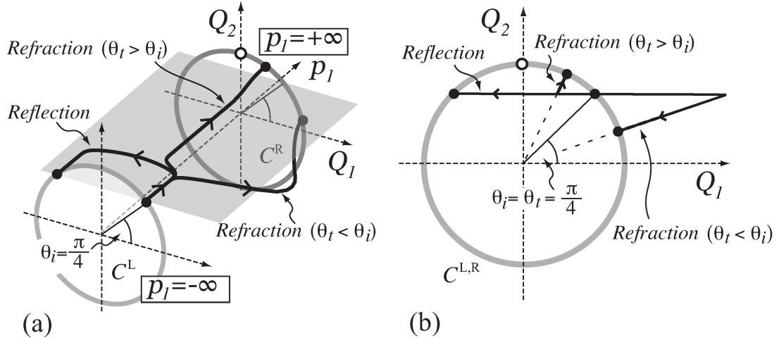
Figure 8. (a) Schematic picture of orbit flows in three-dimensions of (p_1, Q_1, Q_2) . The solid circles C^{L,R} show the invariant circles of TS solutions at p_1 = \mp\infty , respectively. The solid curves indicate the orbit flows starting from \theta_i = \pi/4 for the reflection of \hat{\epsilon} = 70 and refraction for 35 and -350 , respectively. The white disk on C^R indicates the traveling spot solution moving parallel to the jump line, corresponding to \theta_t = \pi/2 . It plays a role of scatter for the transition between reflection and refraction behaviors. (b) The projection of orbit flows onto the (Q_1, Q_2) -plane. The refraction behaviors initially move on the plane where Q_2 is conserved, indicated by the gray plane in (a), and then they gradually depart from that into the final destination of TS on C^R along its stable manifold in the direction of e(\theta_t) .
