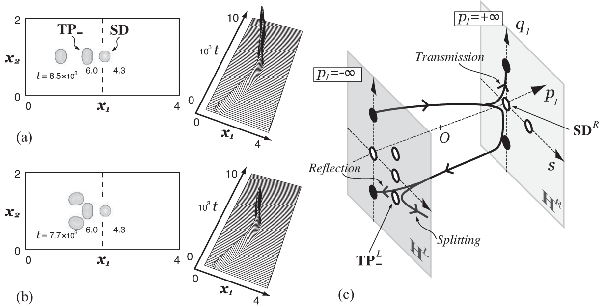
Figure 10. (a) Response of the traveling spot coming from the left when it meets the heterogeneity. We set to (f_1^L, \epsilon) \approx (0.06046, 7.2817 \times 10^{-4}) . The left two figures show the behaviors when the spots turn back and cross the jump line for the second time. The left upper figure first shows the initiation of splitting, but it recovers the original shape afterwards. As \epsilon is decreased slightly, the transition from reflection to splitting occurs as shown in the left lower figure (b). The middle figures show the associated time evolutions of the cross section at x_2 = 1 along the x_1 -axis. In both cases there appear quasi-steady traveling peanuts (TPs) that persist for a certain time before settling down to each final state. (c) Schematic picture of orbit flows in the three-dimensions of (p_1, q_1, s) near triple junction point of Fig.9(a). The orbits starting from TS_+^L are sorted out along the heteroclinic connection between SD^R and TP_-^L .
