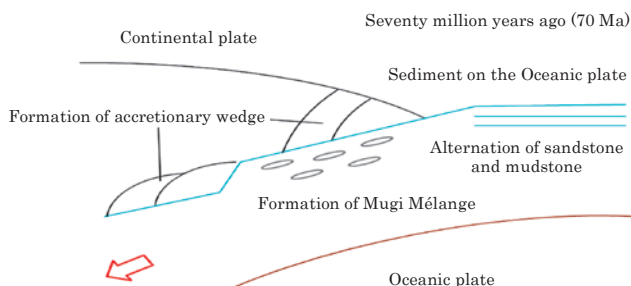
Fig.1. Schematic diagram of the accretionary wedge.
