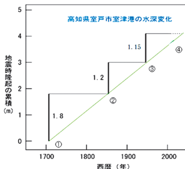
Fig.9. Time-predictable model (1, 4).
