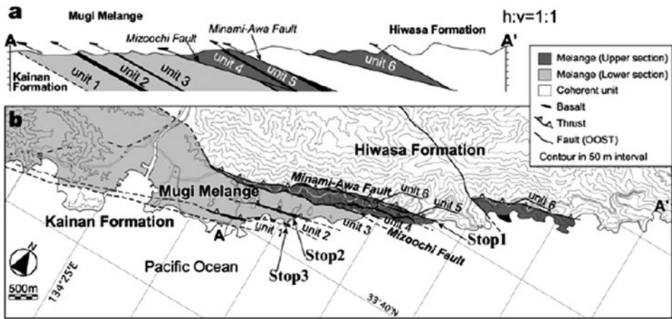
Fig.6. A geological map of the Mugi Mélange (3).
