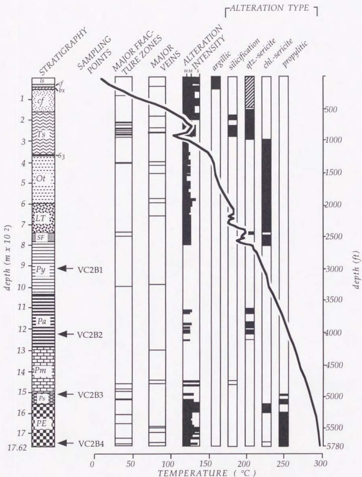
Fig.2 Summarized geologic log for VC-2B core hole and sampling points (modified from Hulen and Gardner, 1989).
