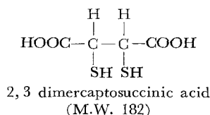
Fig. 1. Chemical structure of DMSA.
