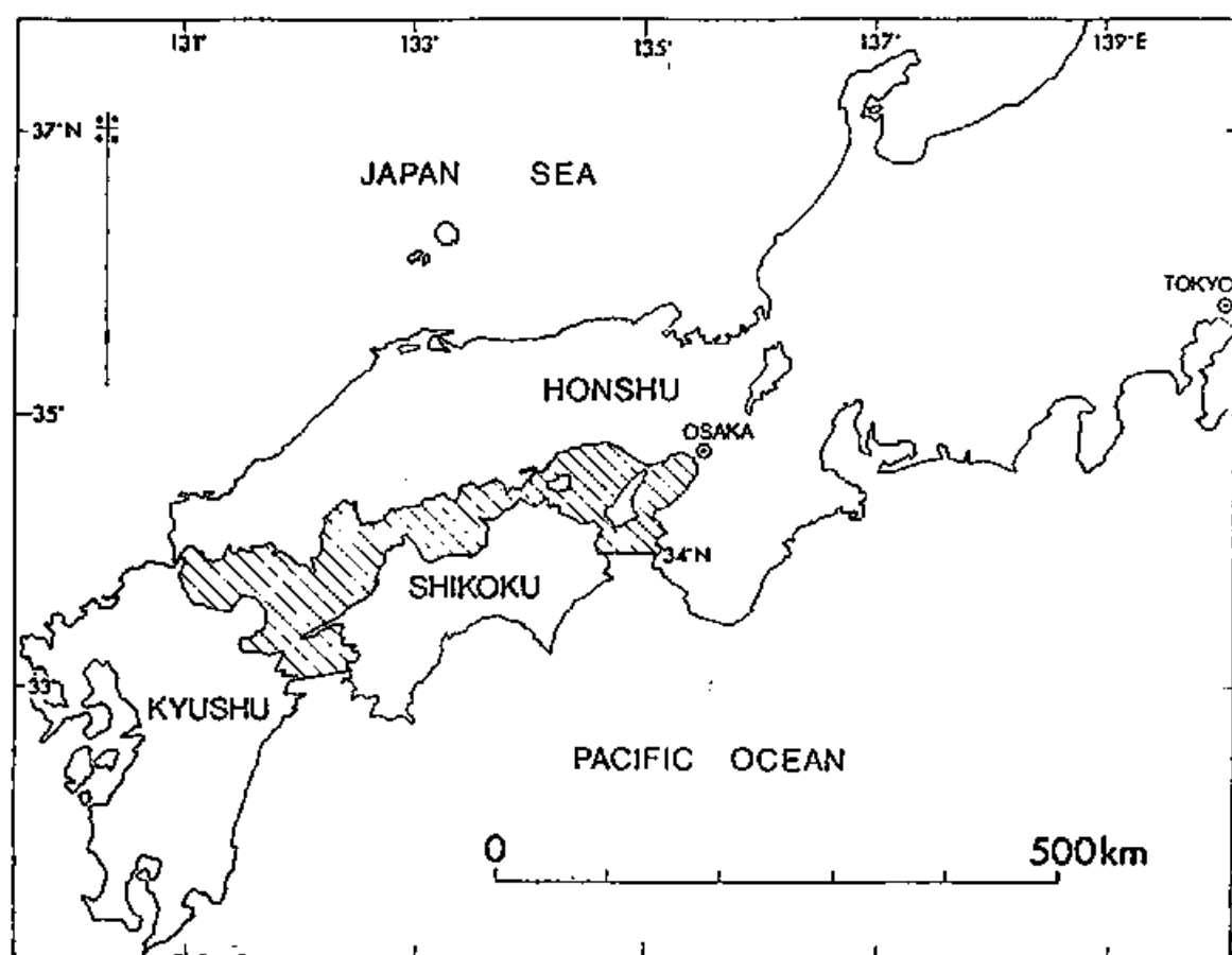
Fig. 1 Index map of the study area.
