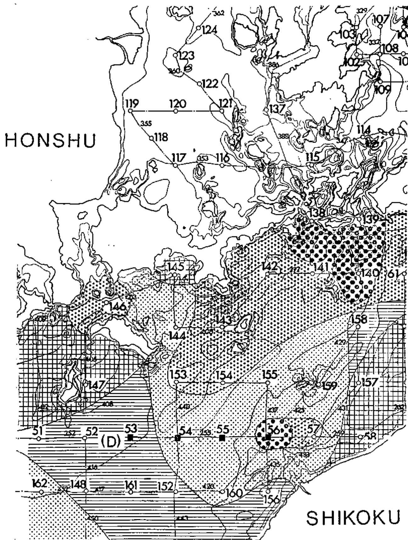
Fig. 11-5 Detailed distribution map of surface sediments in Mzô. Eastern part of Iyo Nada.
