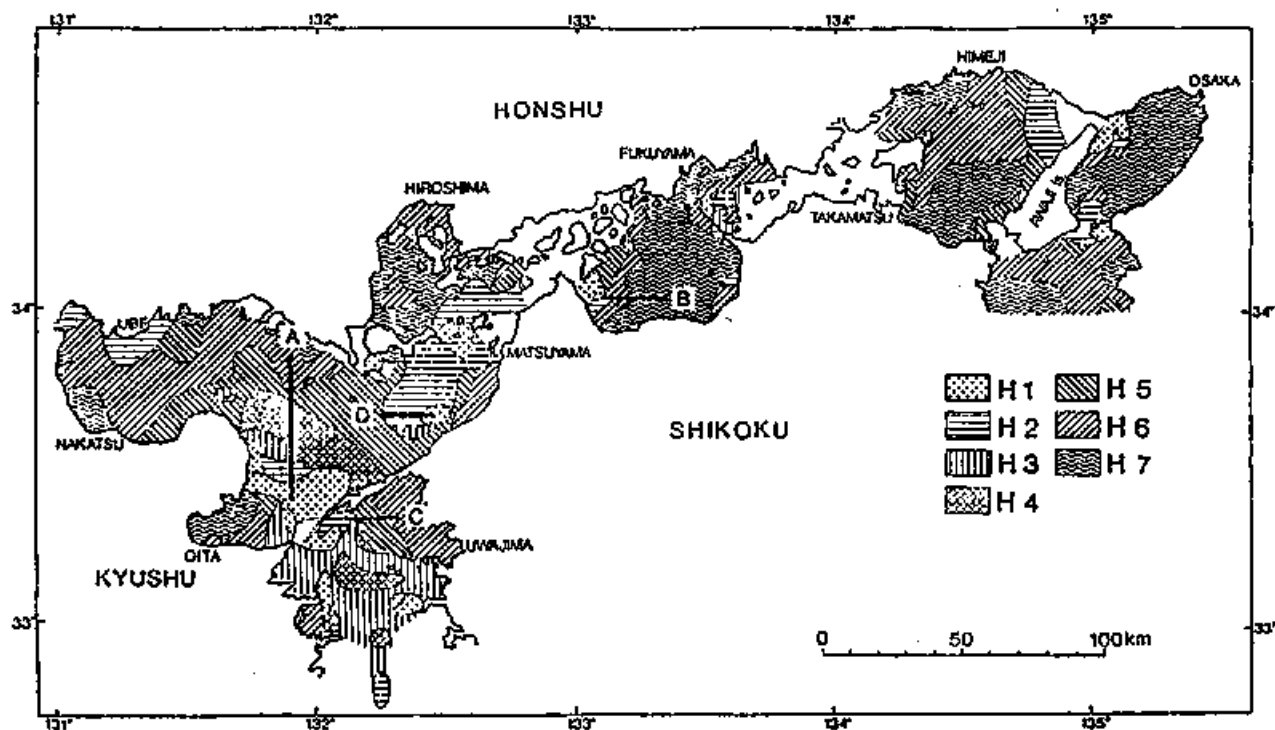
Fig. 14 Distribution map of sediment types.
