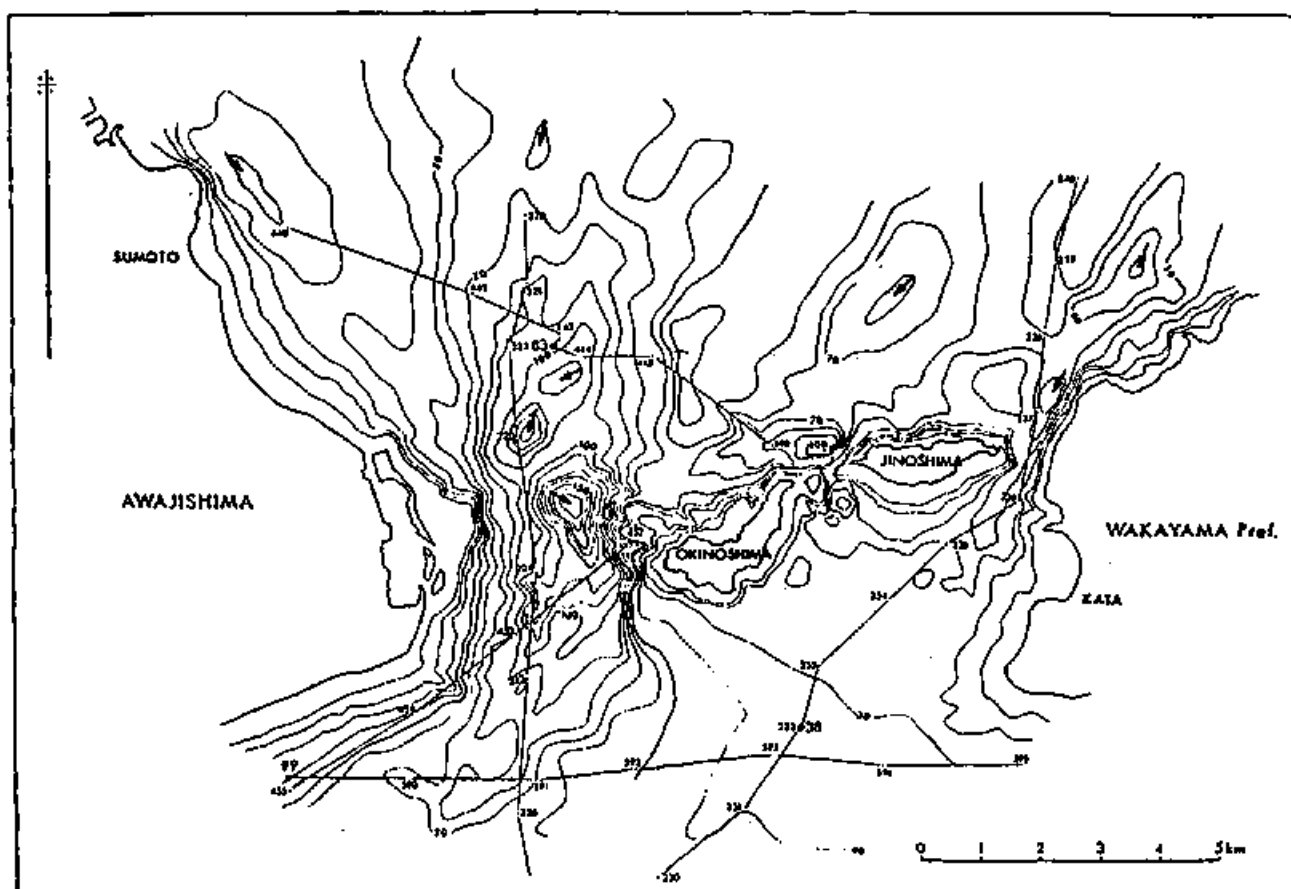
Fig. 5 Bottom topography of Tomogashima Strait. ( Single-type caldron ) Depth in meter. Lines show tracks for seismic profiles.
