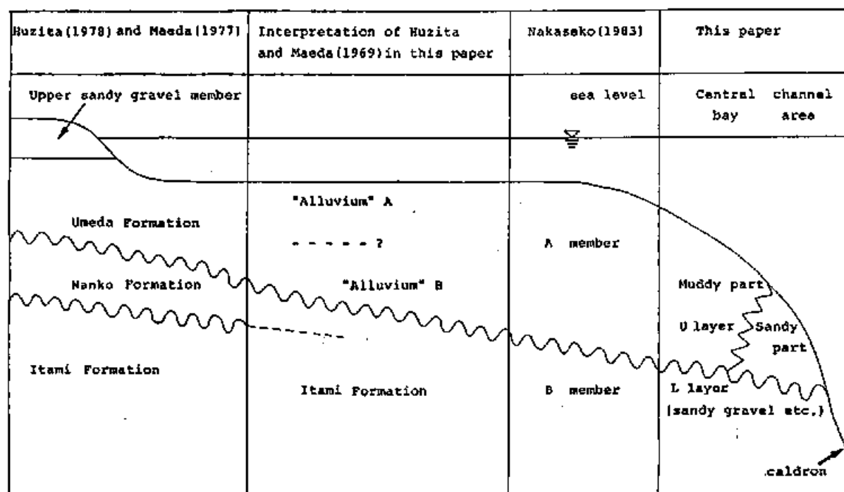
Fig. 23 Holocene stratigraphy in Osaka Bay.
