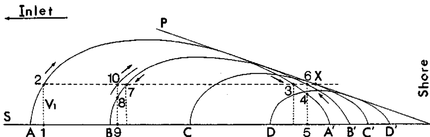
Fig. 21 Settling lag effect (From Straaten and Kuenen, 1958)
