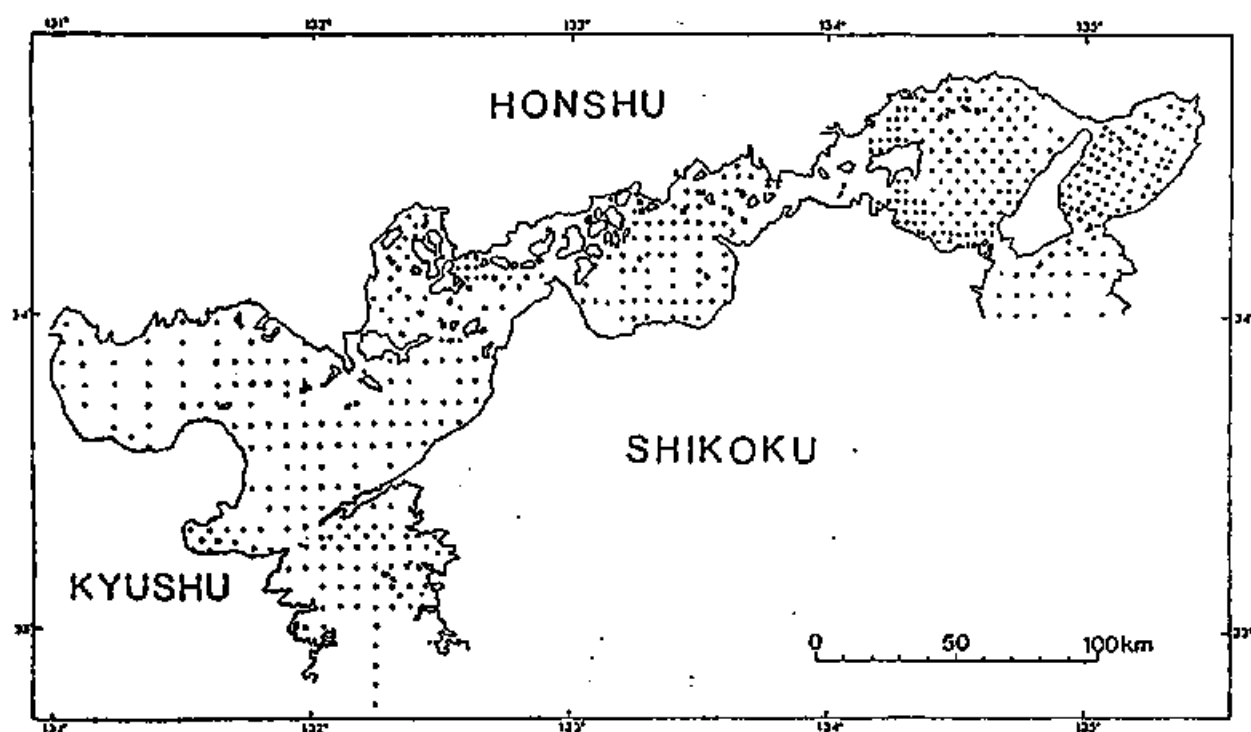
Fig. 2 Sampling locations in the Seto Inland Sea.
