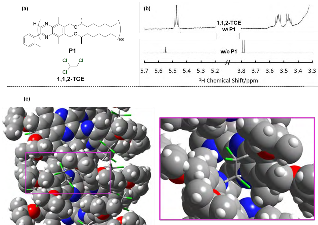
Figure. (a) Structure of P1 and 1,1,2-TCE. (b) 1 H-NMR trace of 1,1,2-TCE with or without P1 in cyclohexane-d 12 . (c) Calculated structure of P1 /1,1,2-TCE complex.
