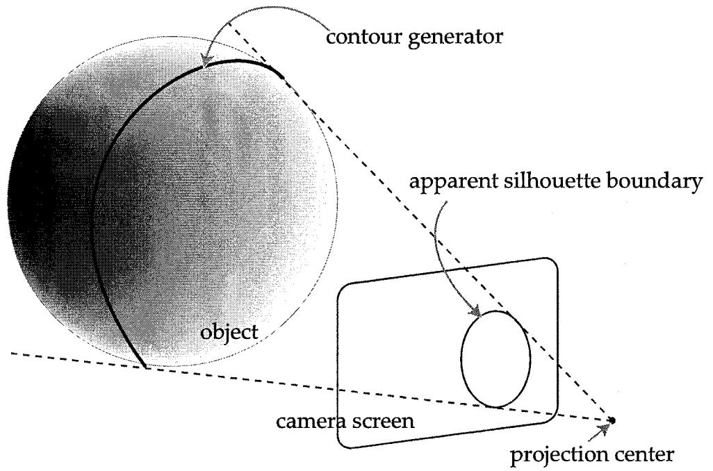
Figure 2.5: Contour generator
