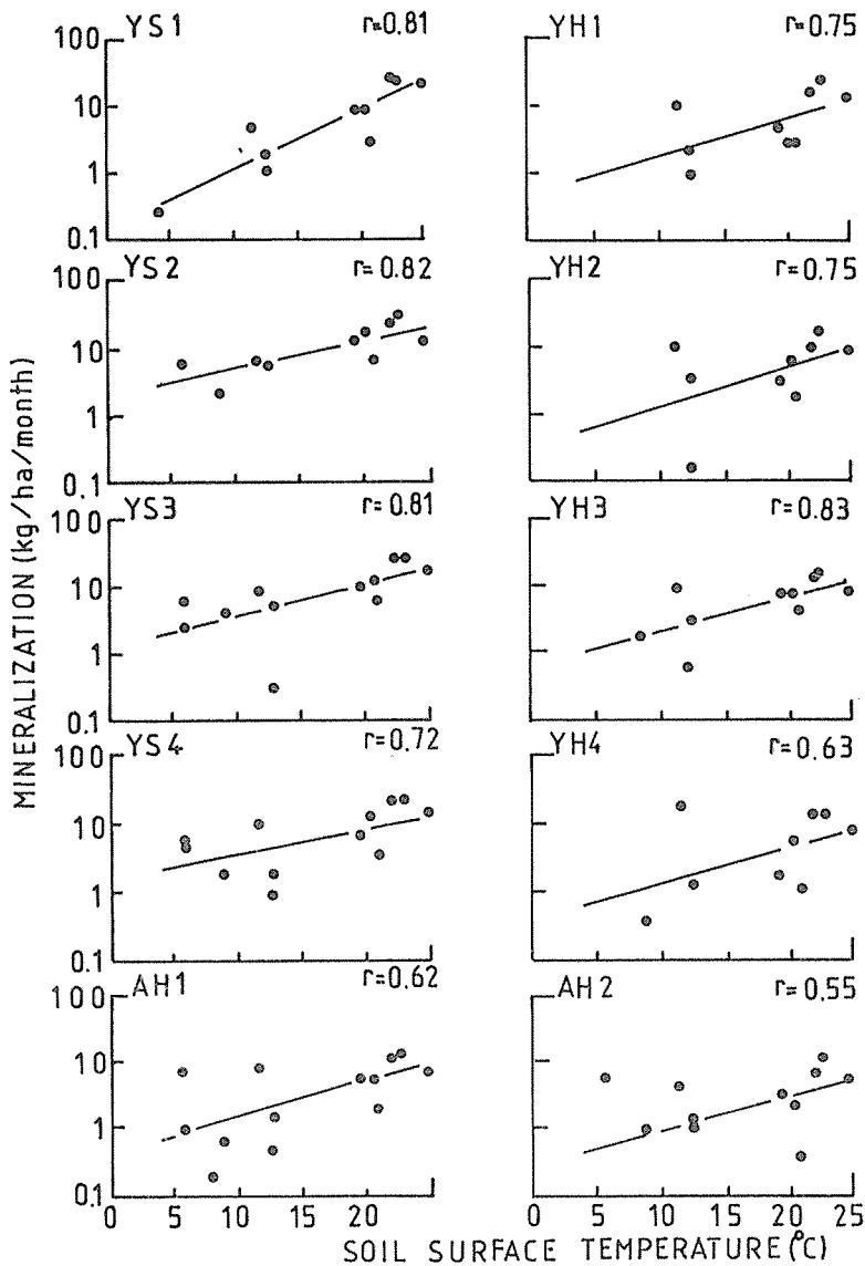
図3 土壌表層の温度と無機化速度の関係 Relationships between mineralization rates and soil surface temperature over a two year period
