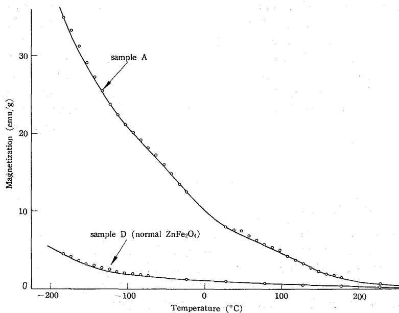
Fig. 4. Magnetization vs. temperature curves of normal \text{ZnFe}_2\text{O}_4 and sample A, measured in the magnetic field of 9600 Oe.
