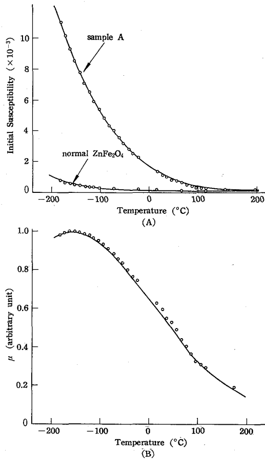
Fig. 7. (A) Initial susceptibility vs. temperature curves of normal \text{ZnFe}_2\text{O}_4 and sample A, measured at 900 Oe.
