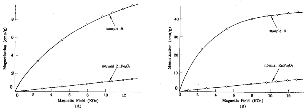
Fig. 5. Magnetization vs. magnetic field curves of normal \text{ZnFe}_2\text{O}_4 and sample A, measured at 20°C (A) and -190°C (B).
