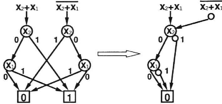
Figure 3.2: Output Inverters
