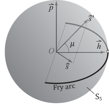
Figure 4: Schematic illustrations of Fry arcs (thick lines) on S_5 . The orthogonal projection of \vec{s} onto the plane spanned by \vec{h} and \vec{p} is denoted by \vec{s}' . The line through the ends of the arc is depicted by a dotted line. Open circle indicates the center of the arc denoted by \vec{h} . Shear stress on the fault corresponding to the arc has the maximum value when \vec{s} indicate this point.
