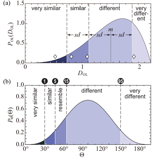
Figure 12: The probability density functions of D_{OL} (a) and \Theta (b) for randomly chosen tensors. Boldface letters indicate the dissimilarity classes of reduced stress tensors of (Orife and Lisle, 2003) (a) and this study (b). The mean and standard deviation of P_{OL}(D_{OL}) are denoted by m and sd in (a). Diamonds indicate the D_{OL} values corresponding to the class boundaries in (b), where the dissimilarity classes with the boundaries at the 1, 5, 15 and 95 percentile points.
