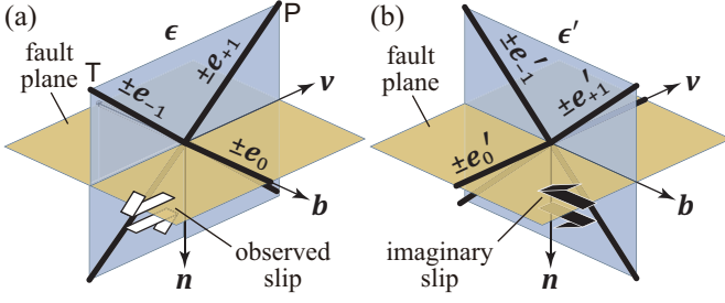
Figure 3: A fault-slip datum, \mathbf{n} , \mathbf{v} and \mathbf{b} = \mathbf{n} \times \mathbf{v} (Fig. 1), and the principal orientations (bold lines) of the corresponding strain tensors, \epsilon and \epsilon' , both of which have the eigenvalues, +1, 0 and -1. The orientations parallel to the eigenvectors of \epsilon are denoted by \mathbf{e}_{+1} , \mathbf{e}_0 and \mathbf{e}_{-1} , where the subscripts indicate the corresponding eigenvalues. Likewise, those of \epsilon' are indicated by \mathbf{e}'_{+1} , \mathbf{e}'_0 and \mathbf{e}'_{-1} . The imaginary slip along \mathbf{b} direction, which brings about the imaginary strain \epsilon' , is shown in (b).
