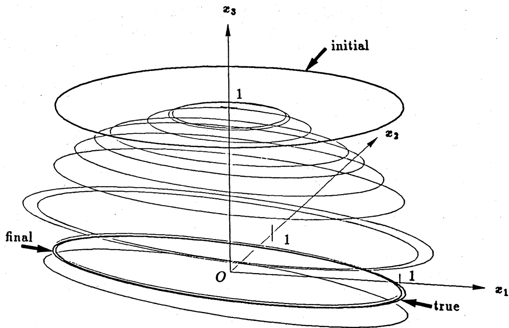
Fig. 2 Mode of convergence in 3D crack determination analysis in time domain.
