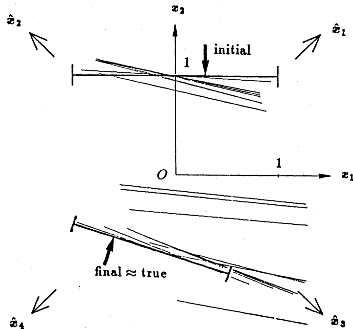
Fig. 1 Mode of convergence in 2D crack determination analysis in time domain.
