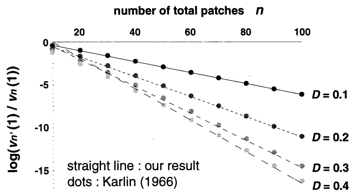
Fig.2 Rapid Decrease of Expected Time to Extinction by Habitat Destruction ( r = 2, c = 1 )
