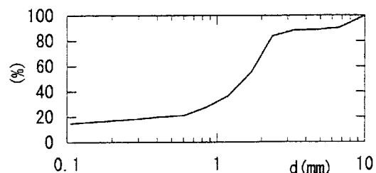
Fig.2 Grain-size distribution of the sand used in experiments
