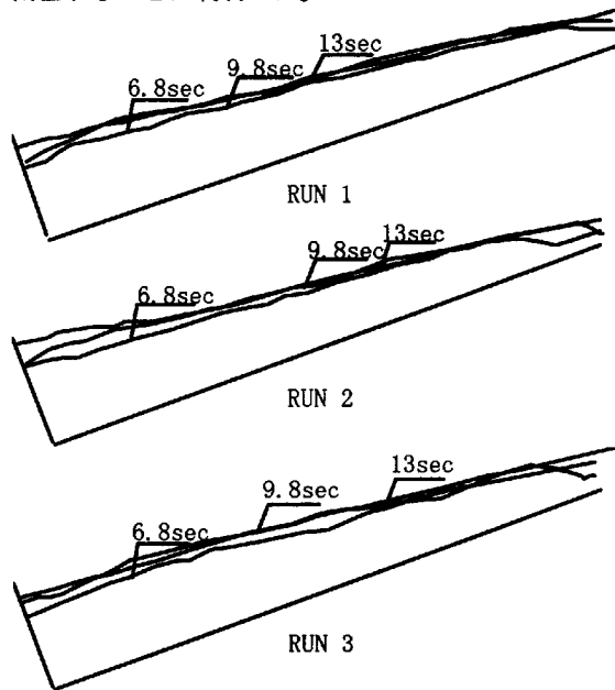
Fig.3 The depositional processes of debris flow by a open-type Sabo dam
