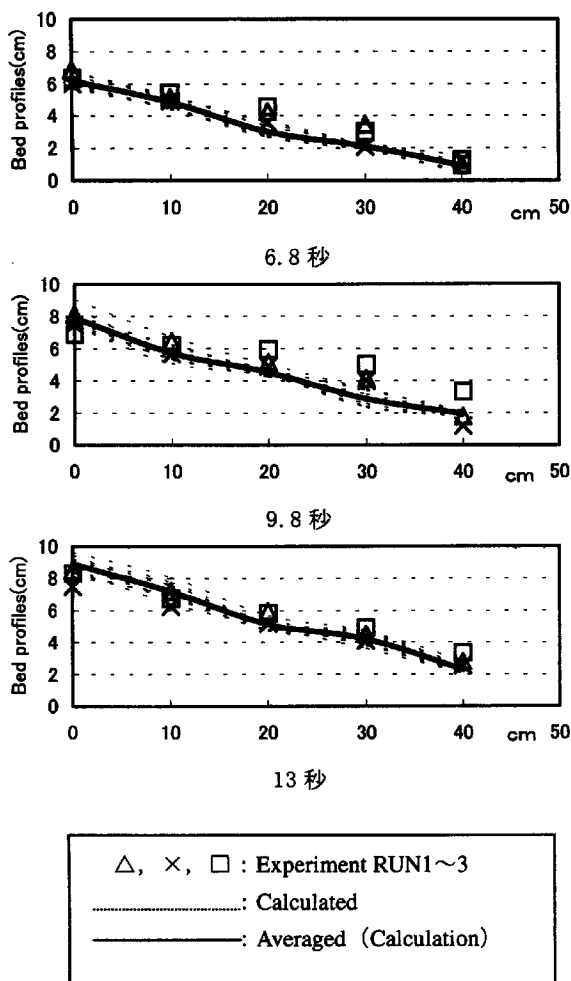
Fig. 8 Comparisons between calculated and Experimental bed profiles
