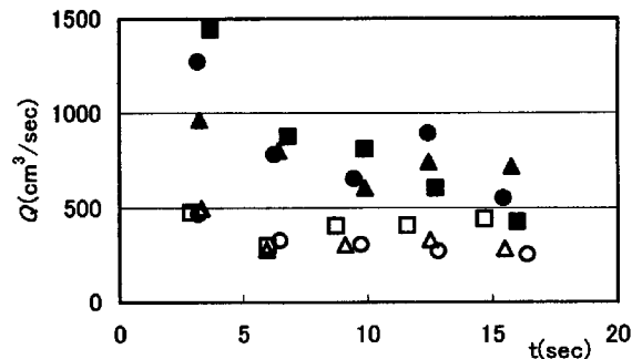
Fig.4 Experimental results of flow discharge
