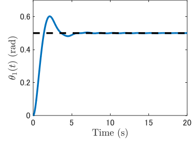
(c) the angle of the motor \theta_1(t)
