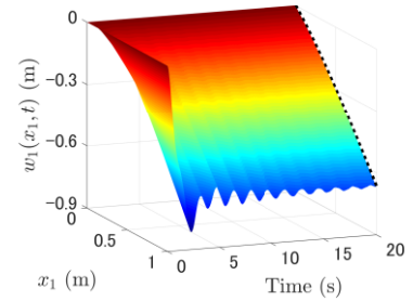
(a) the transverse displacement w_1(x_1, t)
