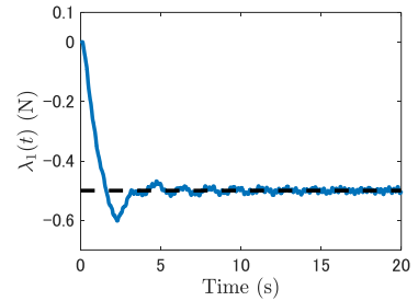
(e) the grasping force \lambda_1(t)
