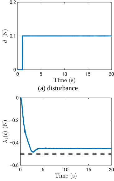
(b) the grasping force \lambda_1(t) with the disturbance. The response of \lambda_1(t) without the disturbance is Fig. 2(e).
