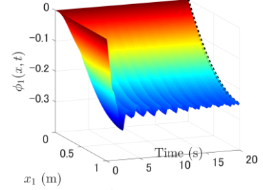
(b) the rotation of the cross section \phi_1(x_1, t)
