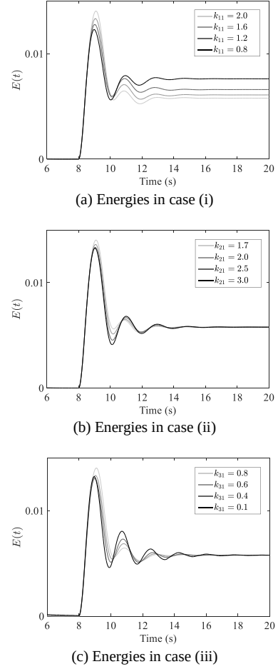
Fig. 5. Influences of gains in the disturbance response
