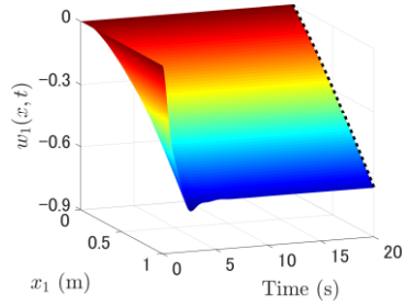
(a) the transverse displacement w_1(x_1, t)
