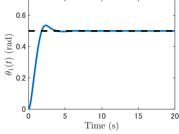
(c) the angle of the motor \theta_1(t)
