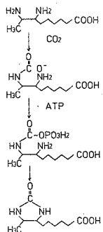
Fig. 3. Proposed mechanism for DTB synthetase reaction.
