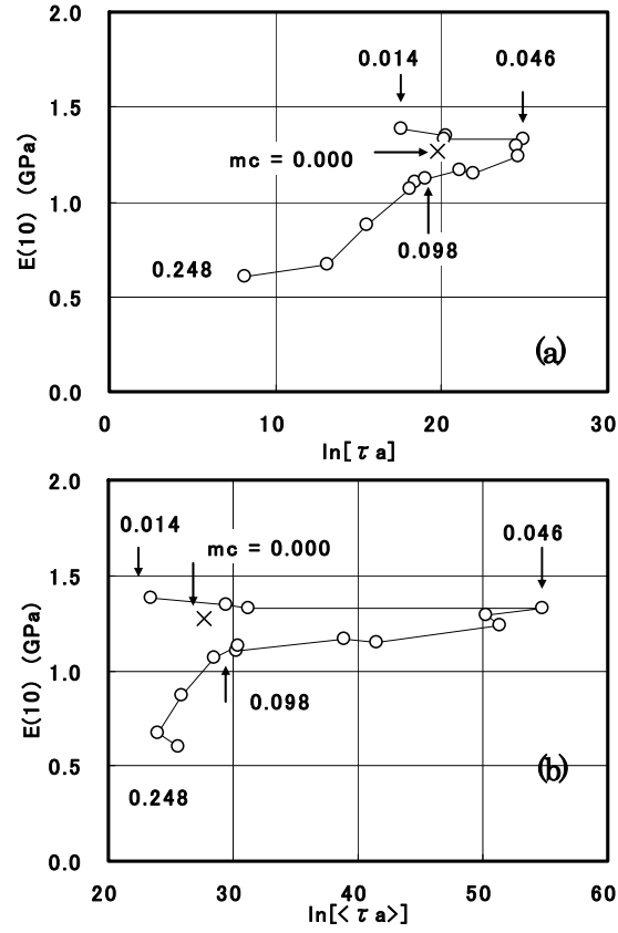
Fig.5. Relationships between E(10) and \tau_a and \langle\tau_a\rangle . Note: E(10) is a relaxation modulus at t=10 , \tau_a is the characteristic relaxation time, \langle\tau_a\rangle is average relaxation time calculated from KWW function's parameters.
