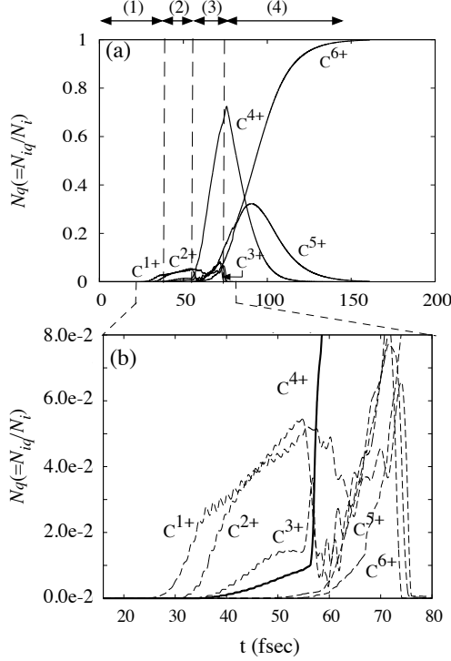
Fig 3.11: (a) Time history of ion abundance for each charge state C^q+ . The dashed lines classify the time region for each ionization phase as different dynamics. (b) Expanded time history of that in the region of 20 \leq t \leq 80 fsec as focused on rapid transition of ionization to C^4 .
