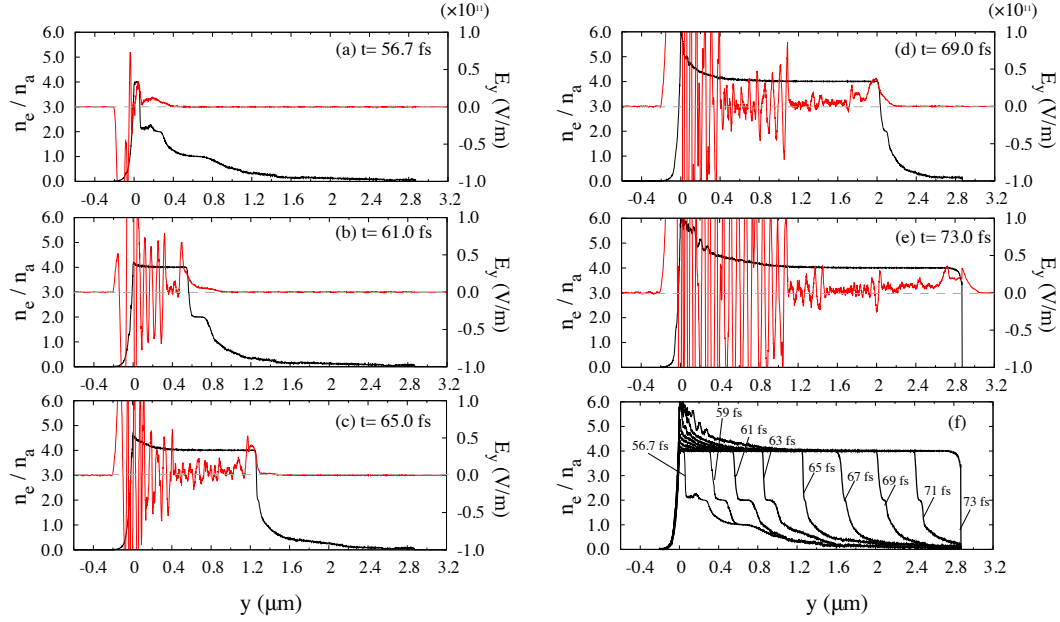
Fig3.7: In (a)-(e), spatial distributions of electron density (black) and electric field for longitudinal direction (red) in total simulation domain ( -0.6 \leq y \leq 3.2 \mu\text{m} ). In (f), the electron density profiles every 1.9 fsec from 56.7 fsec as ionization phase (3).
