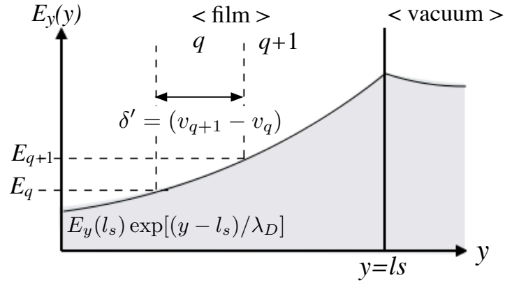
Fig5.8: Schematic representation of Debye screening of sheath field and charge distributions around rear surface of the film.
