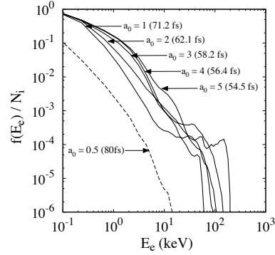
Fig3.18: The normalized electron distribution f(E_e)/N_i with respect to the electron energy E_e , where the electron distribution f(E_e) and total ion number N_i .
