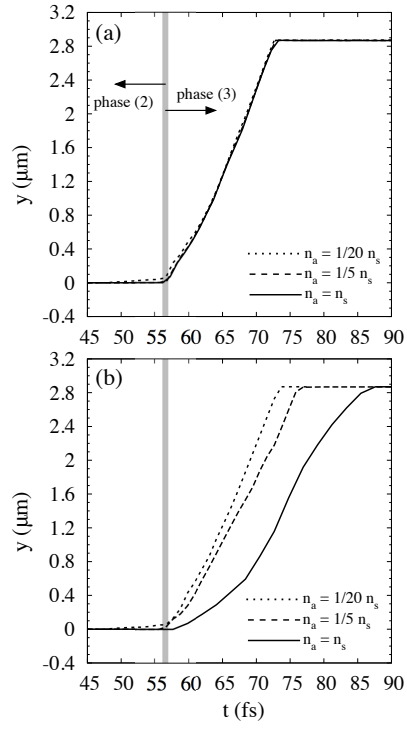
Fig3.16: Time history of the ionization front location of C^4 in the carbon density n_a = 1/20 n_s (dotted line), n_a = 1/5 n_s (dashed line), and n_a = n_s (solid line) without field ionization loss (a) and with field ionization loss (b), where n_a is the atomic density and n_s is the solid carbon density.
