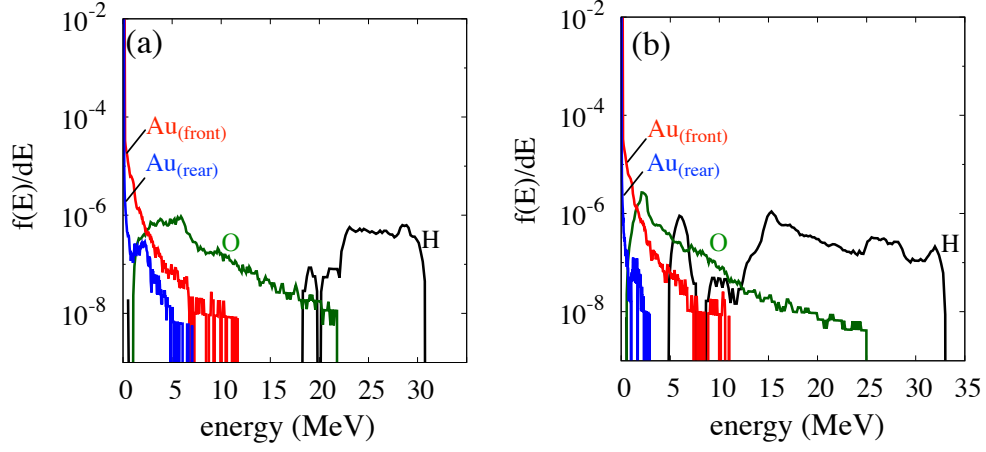
Fig5.7: Ion energy distribution of Au from the front surface Au_{(front)} and the rear surface Au_{(rear)} , and the distributions of p, and O which initially locate on the rear surface with the thickness of (a) 10.0 nm and (b) 20.0nm
