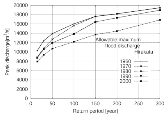
Fig. 5.7 Simulated peak discharges at Hirakata with different magnitude of input rainfall. Years (1960, 1970, etc.) denote that the dams existed in the year are included in the simulation at Kamo
