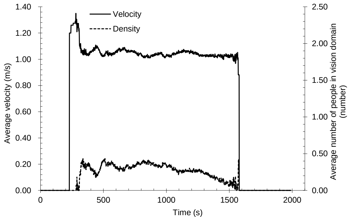
Fig. 5.17 Time series of average velocity and average number of people in vision domain for model-1 at test area for unidirectional flow
