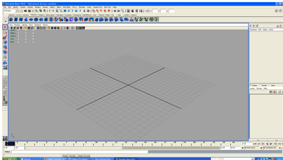
Fig. 3.8 Maya interface
