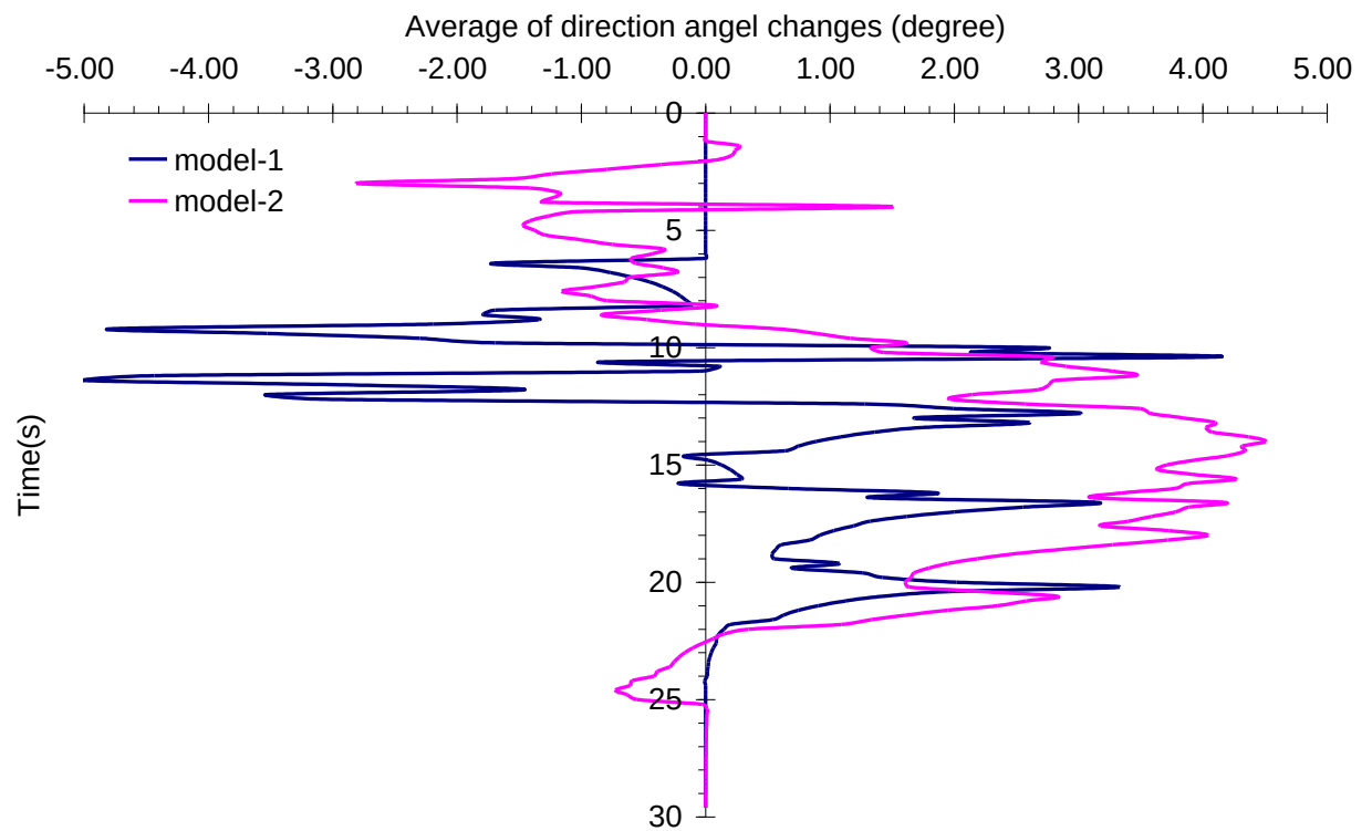
Fig 5.9 The time series of the average of direction angle change for the validation process set 2
