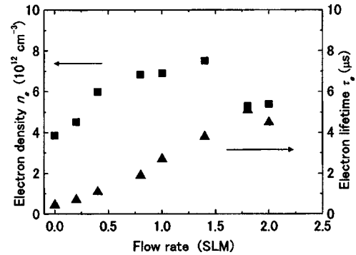
FIG. 8. Electron density and lifetime in the afterglow measured in the mesh-electrode system as a function of the gas flow rate at atmospheric pressure.
