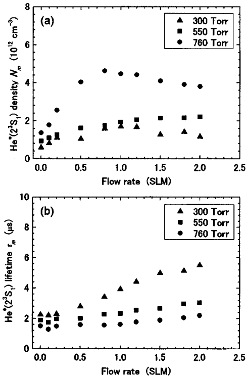
FIG. 5. (a) Density of \text{He}^*(2^3S_1) atoms and (b) their lifetime in the afterglow measured in the mesh-electrode system as a function of the gas flow rate at three different pressures.
