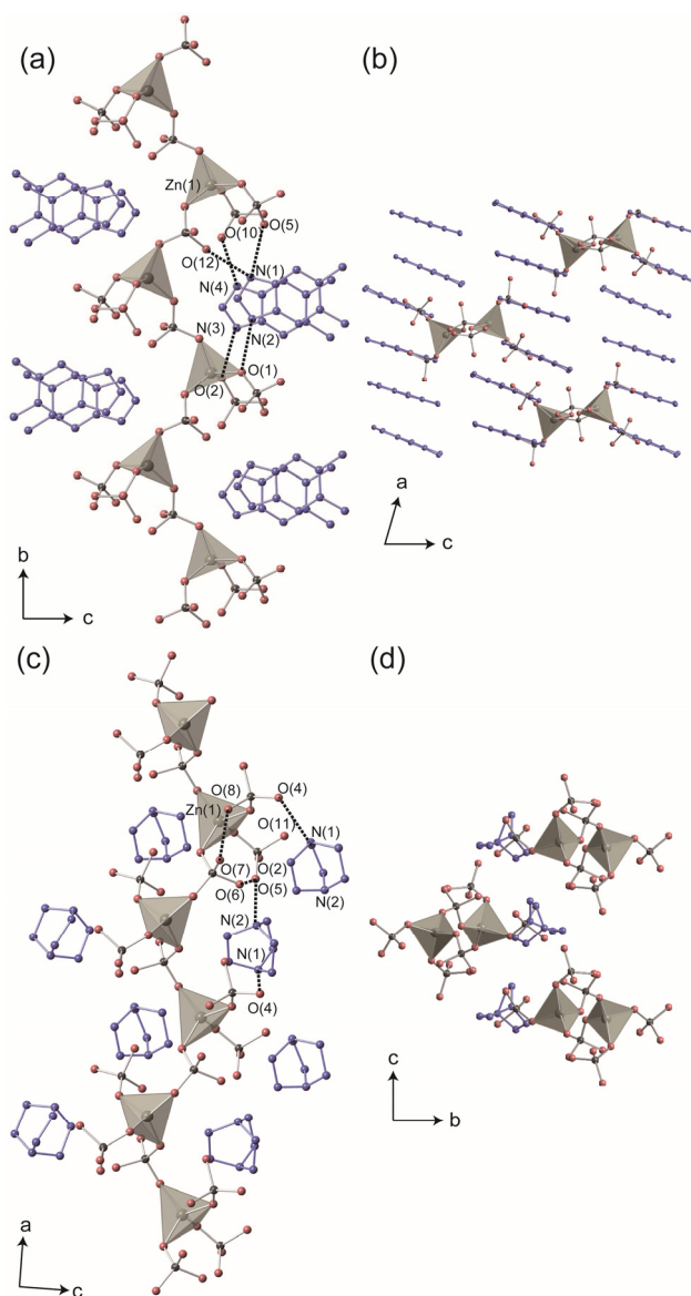
Fig. 1 (a) Crystal structure of [\text{Zn}(\text{H}_2\text{PO}_4)_2(\text{HPO}_4)] \cdot (\text{H}_2\text{dmbim})_2 ( 1 ) along the a axis and (b) the b axis at -50^\circ\text{C} . (c) Crystal structure of [\text{Zn}(\text{H}_2\text{PO}_4)_2(\text{HPO}_4)] \cdot \text{H}_2\text{dabco} ( 2 ) along the b axis and (d) the a axis at -50^\circ\text{C} . The \text{H}_2\text{dmbim}^+ ions and \text{H}_2\text{dabco}^{2+} ions are highlighted as purple and hydrogen atoms are omitted. H-bonds between the 1-D chain and \text{H}_2\text{dmbim}^+ and \text{H}_2\text{dabco}^{2+} are shown as black dotted lines. [Color coding: Gray: Zn and P, pink: O, purple: N and C.]
