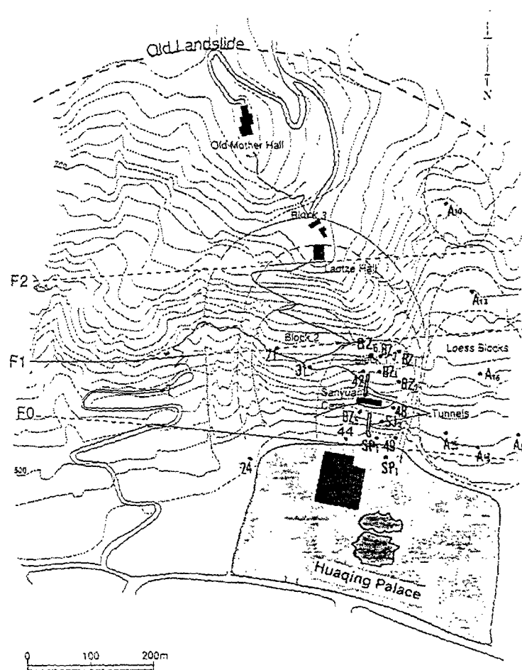
Fig. 3 Location map of boreholes and faults.
