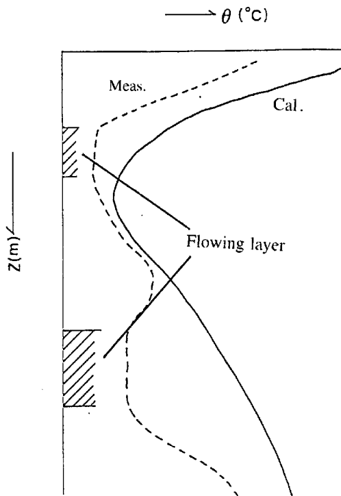
Fig. 1 Disturbance of usual temperature by existing of ground water-flowing layers.
