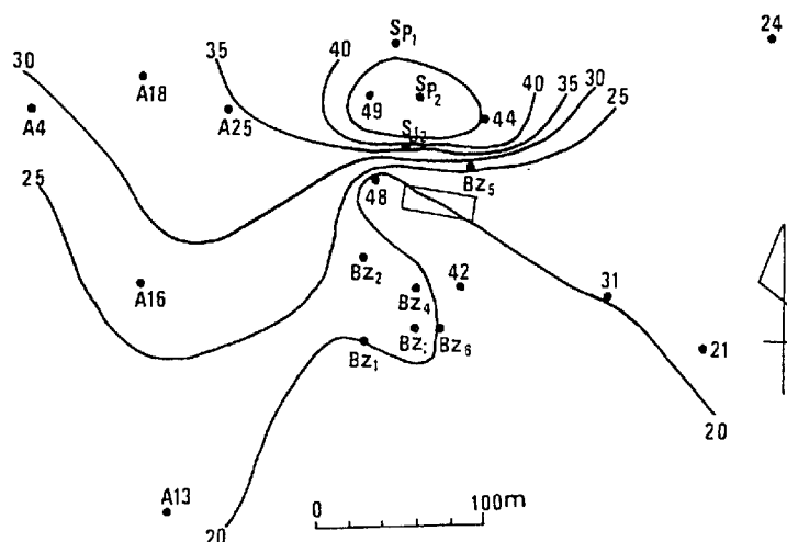
Fig. 27 Temperature distributing map at the bottom of each borehole.
