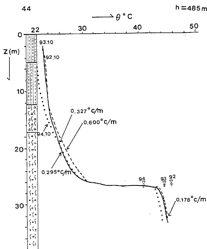
Fig. 9 Temperature logging curves at No. 44 borehole.
