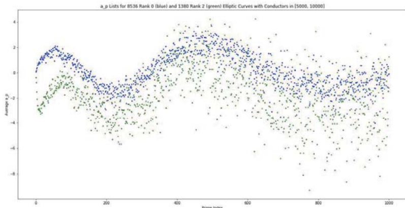
FIGURE 3. Plot of f_r(n) for N \in [5000, 10000] with r = 0 and r = 2 . Original plot due to [HLOP24].
