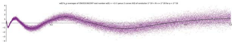
FIGURE 6. Genus 2 curves over \mathbb{Q} with Sato-Tate group \mathrm{USp}(4) .
