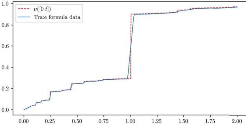
FIGURE 10. Plot of \nu([0, t]) scaled by t\sqrt{N} and numerical data with R = 6900 , H = 100 and t \in [0, 2] from Theorem 3.3. Note that this graph is identical to the plot for \delta = 0 from Figure 9.
