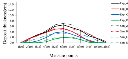
Figure 3.24 Comparison of deposit thicknesses for sediment B
