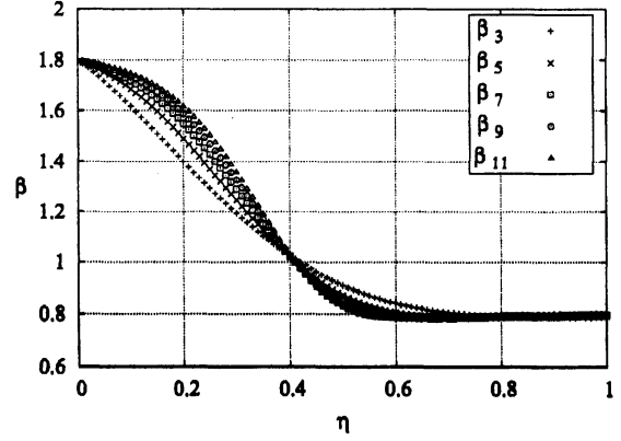
Fig. 16. Finite range scaling exponent for p = 1.8 .
