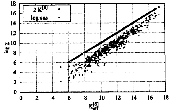
Fig. 11. Random coupling constant check of the susceptibility upper bound.
