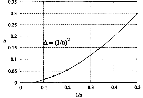
Fig. 14. Finite range scaling exponent for the weak region, p = 2 , \eta = 0.1 . Expected exponent is 2.0.
