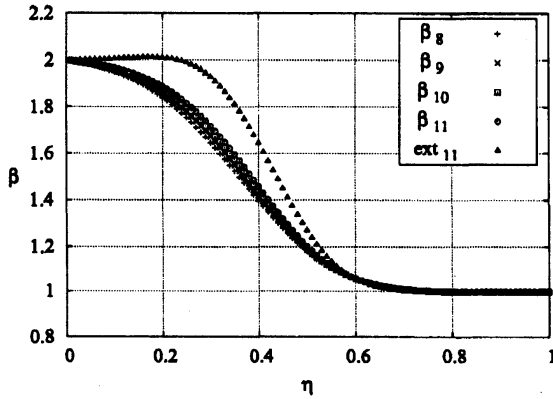
Fig. 19. Extrapolation with up to n = 11 data for p = 2.0 .
