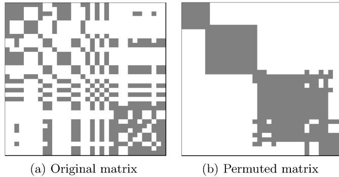
Figure 1: Comparison with two matrices
