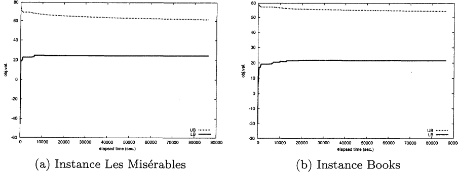
Figure 2: The upper and lower bounds vs. elapsed time in the branch-and-bound
