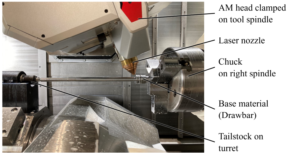
Fig. 6.4 Experimental setup for the DED coating on the drawbar using the LASERTEC 3000 DED hybrid machine.
