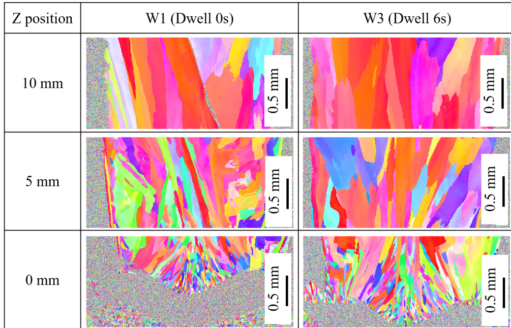
Fig. 3.14 Inverse pole figures observed with EBSD for workpieces W1 and W3.
