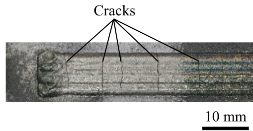
Fig. 4.4 Multiple cracks across a layer of Stellite 1, deposited on a S50C steel substrate without preheating (laser power of 2400 W).
