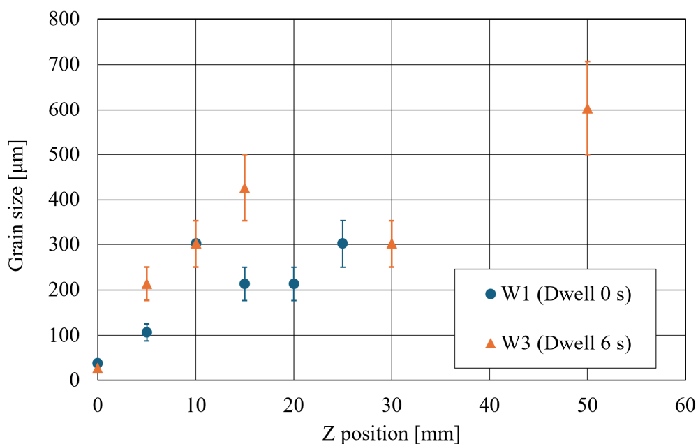
Fig. 3.16 Grain size at each deposition height for workpieces W1 and W3.
