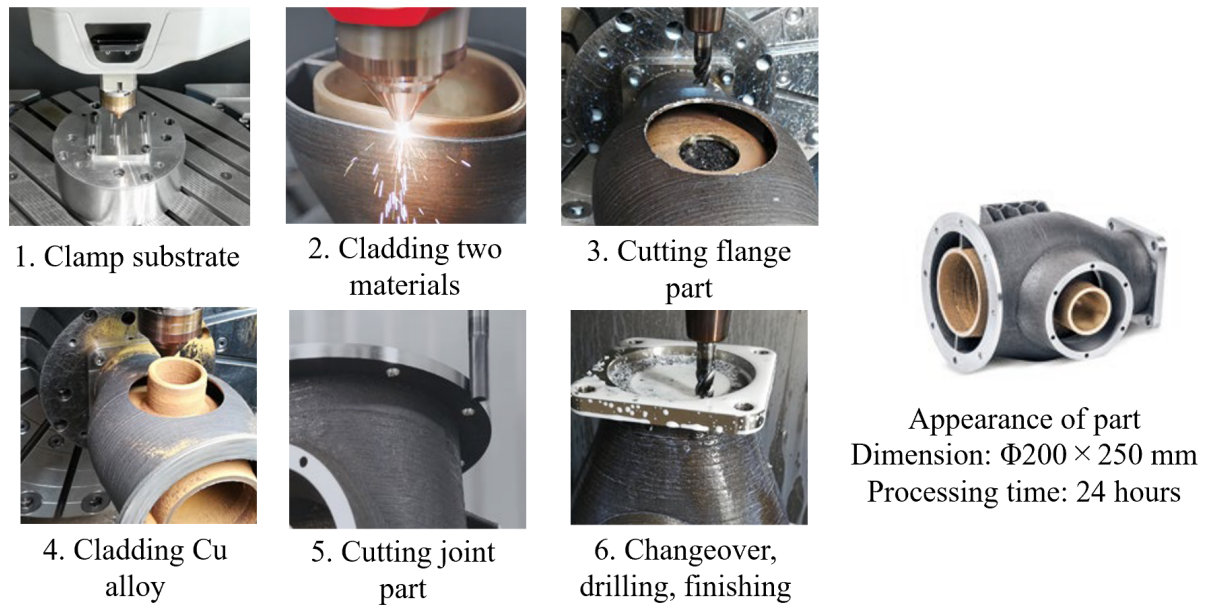
Fig. 2.3 Fabrication of a bimetal heat exchanger using a hybrid DED machine.
