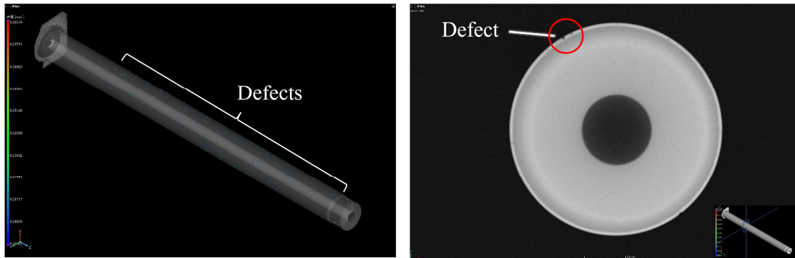
Fig. 6.6 Example image of the X-ray CT scan where defects were detected.
