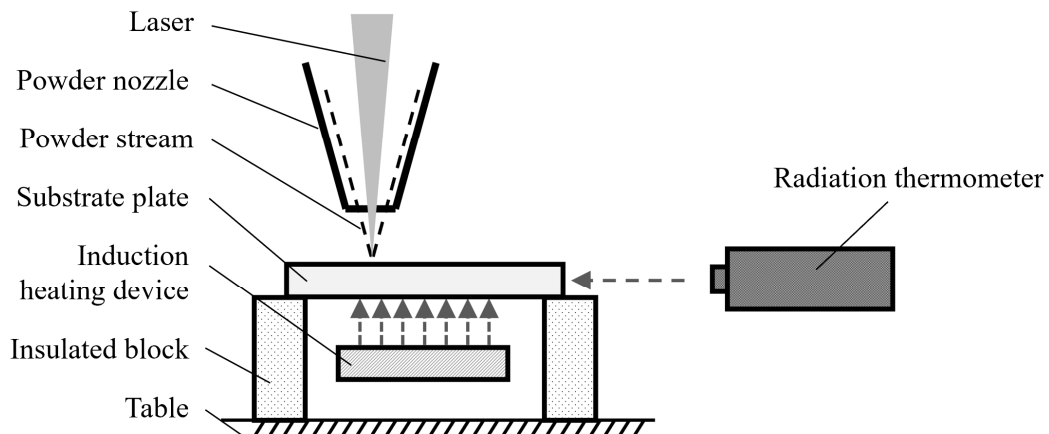
Fig. 4.1 Schematic of the DED process with induction preheating.
