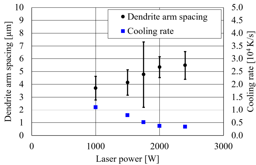
Fig. 4.17 Relationship between laser power and the dendrite arm spacing and cooling rate.
