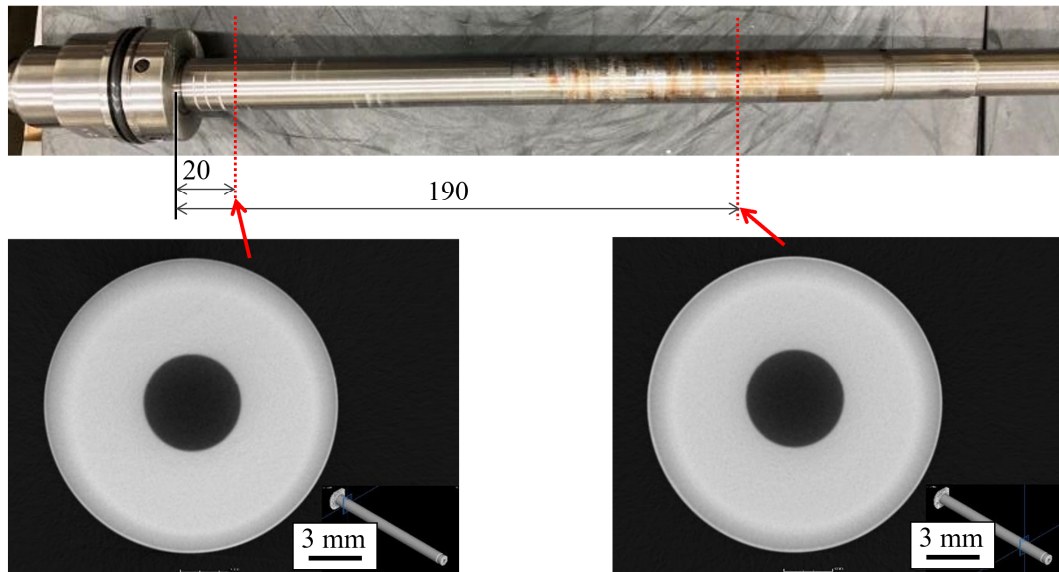
Fig 6.10 Internal crack evaluation by X-ray CT scan.
