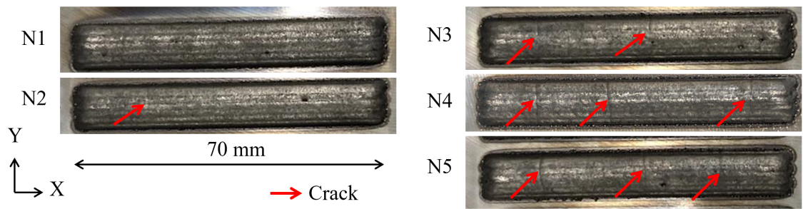
Fig. 5.6 Images of deposited workpieces.
