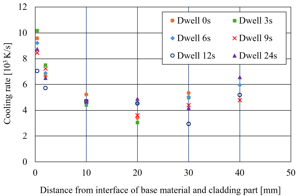
Fig. 3.9 Cooling rate for each deposition condition at each deposition height.
