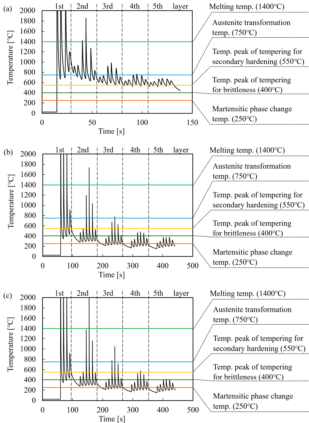
Fig. 5.10 Thermal history simulated by thermal analysis for (a) N1 (0.1 mm height), (b) N5 (0.3 mm height), and (c) N5 (0.6 mm height).
