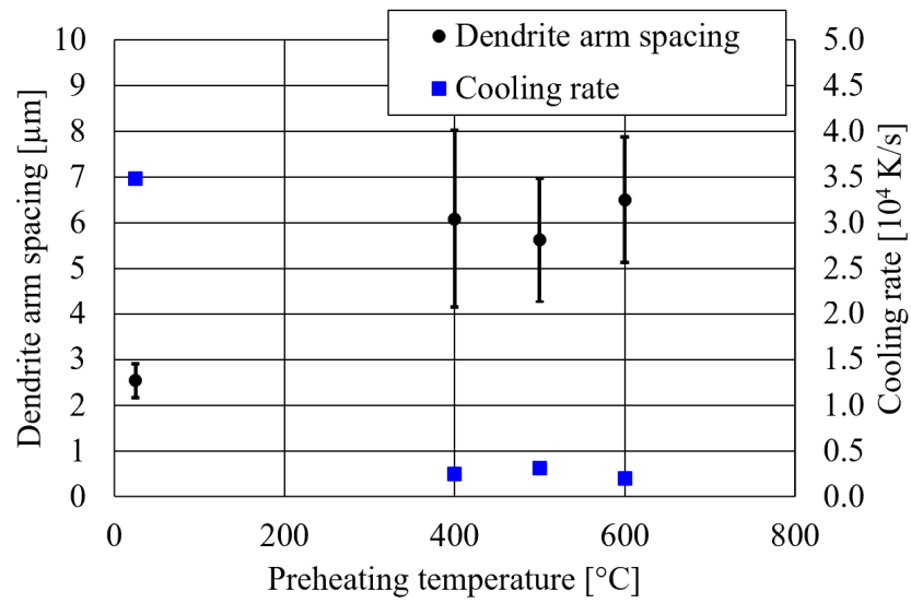
Fig. 4.16 Relationship between preheating temperature and the dendrite arm spacing and cooling rate.
