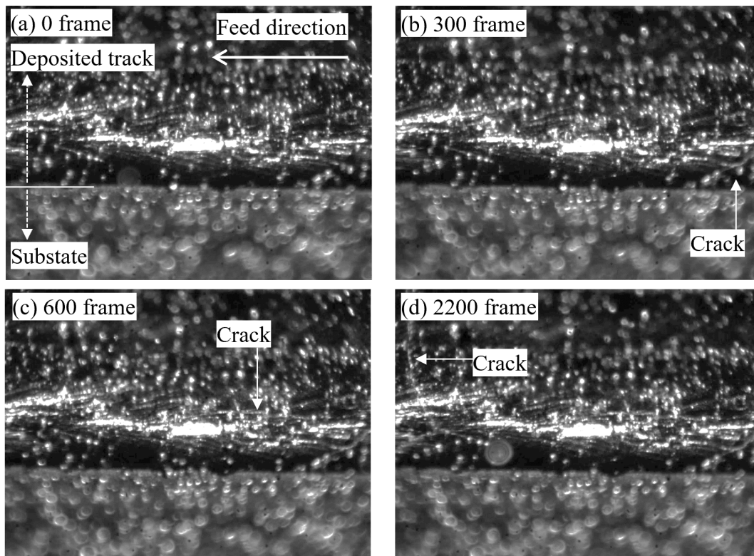
Fig. 4.9 Observation of cracks using images taken with a high-speed camera: (a) before crack generation at 0 frame, (b) parallel crack with path at 300 frame, (c) 0.5 s after solidification at 600 frame, and (d) vertical crack with path at 2200 frame.
