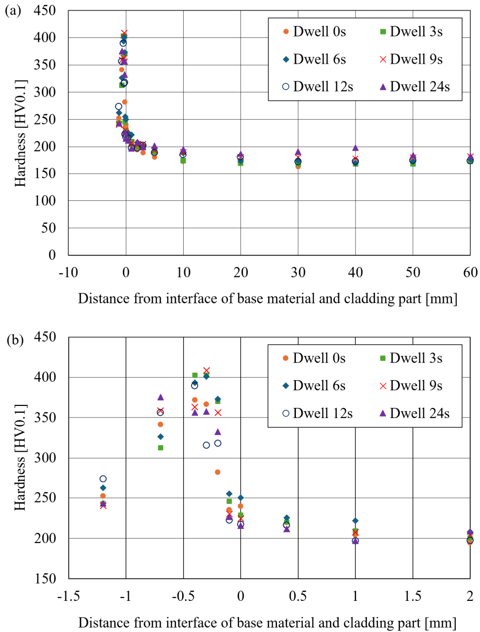
Fig. 3.11 (a) Measured hardness of each workpiece for the entire region and (b) magnification of the near interface between the base material and cladding.
