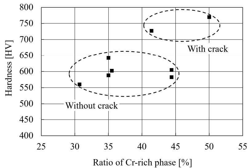
Fig. 4.13 Relationship between hardness and the Cr-rich phase ratio for each test piece.
