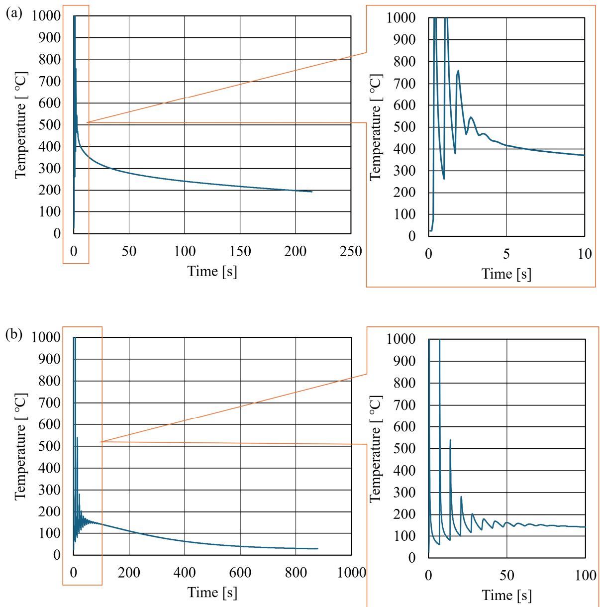
Fig. 6.3 Thermal history of Point A (shown in Fig. 6.2) estimated by thermal simulation for dwell times of (a) 0 and (b) 6 s.
