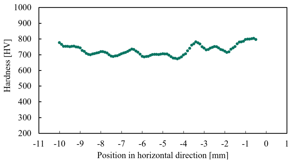
Fig. 5.8 Hardness distribution in the horizontal direction for N5 (0.5 mm height).
