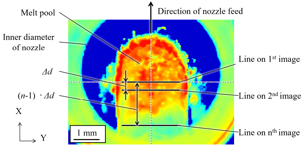
Fig. 3.4 Temperature evaluation lines and melt pool displacement per one frame \Delta d on a melt pool image (length of the lines is 2.2 mm).
