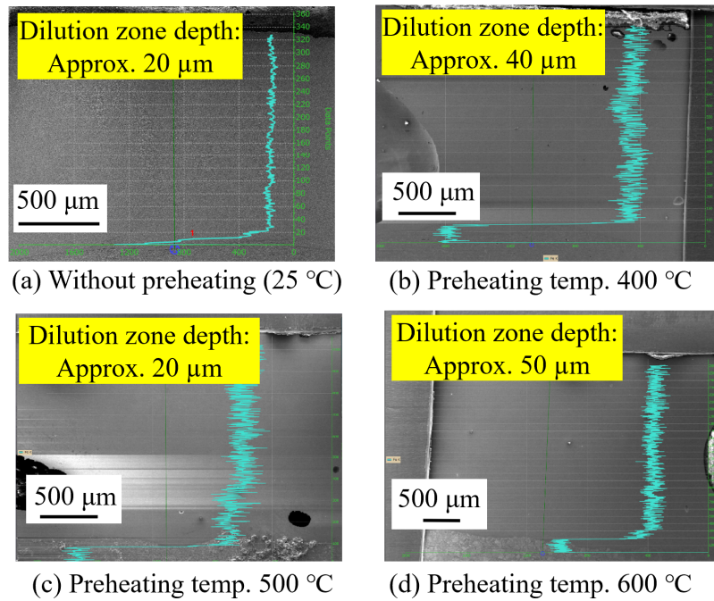
Fig. 4.15 Dilution zone depth estimated by EDX line mapping for each test piece deposited with different preheating temperatures.
