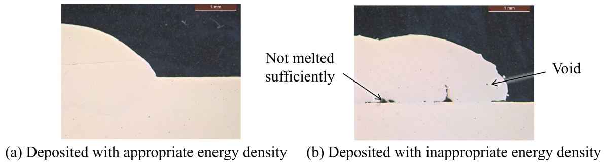
Fig. 2.6 Cross-section of the beads deposited with appropriate and inappropriate energy densities.
