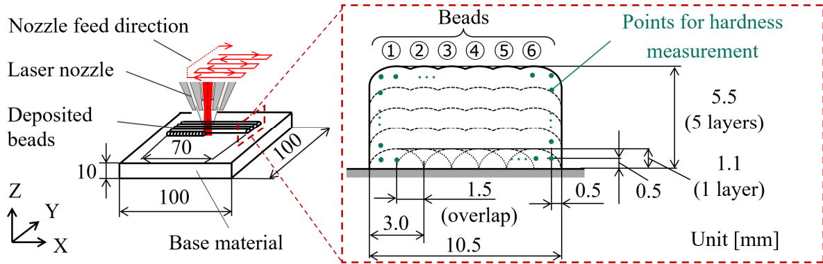
Fig. 5.5 Experimental setup.
