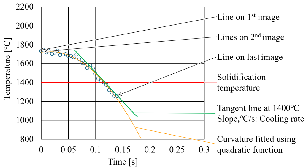
Fig. 3.5 Calculation results of the average temperature and estimation of the cooling rate for a dwell time of 12 s and deposition height of 10 mm.
