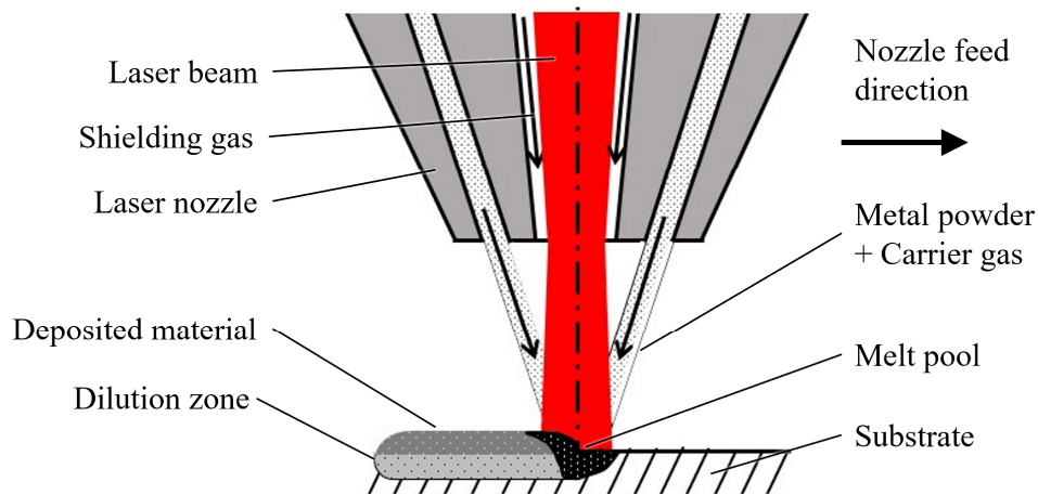
Fig. 2.5 DED process with a metal powder.
