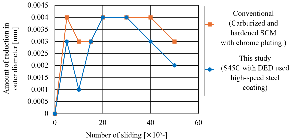
Fig. 6.11 Wear resistance evaluation result for drawbar cladding by DED.
