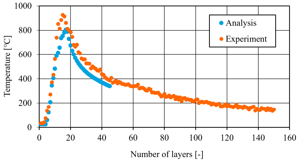
Fig. 5.4 Comparison between the measured and simulated workpiece temperatures during thin-wall deposition.
