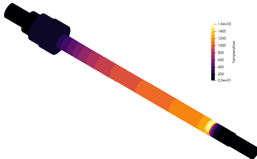
Fig. A.2.1 Temperature distribution of the drawbar immediately after completion of deposition.
