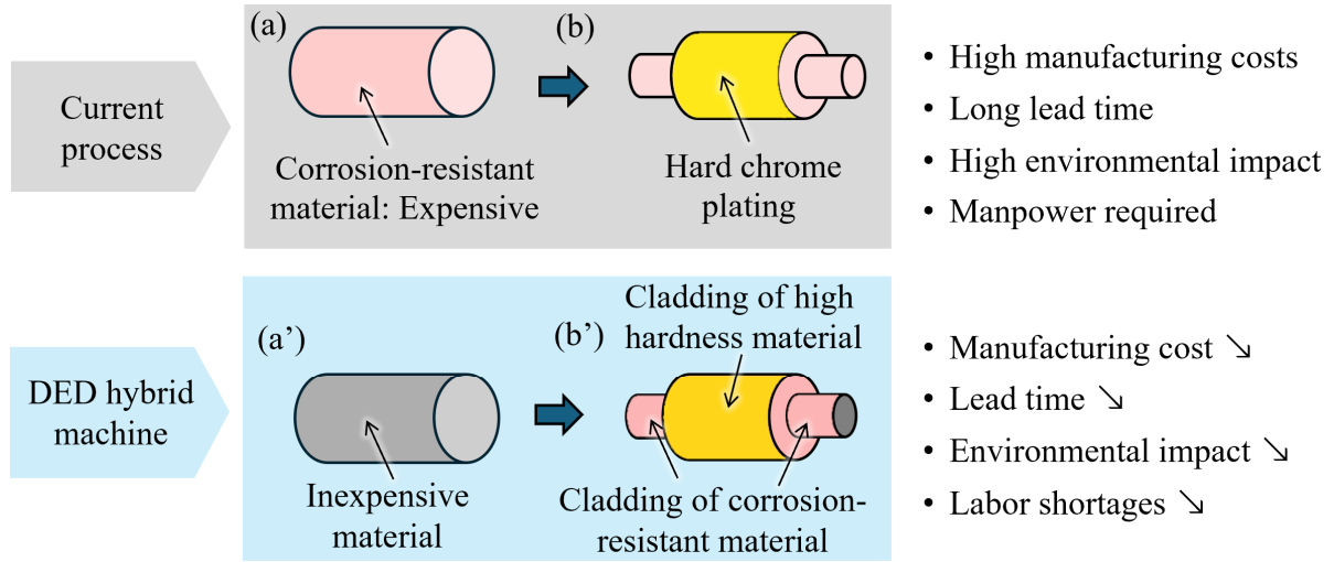
Fig. 2.4 Comparison of the conventional process with the innovative process using hybrid DED in the production of a die cut roll part.
