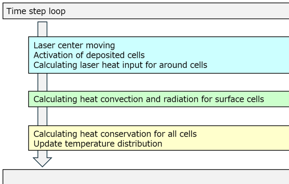
Fig. 5.2 Algorithm flow for heat transfer simulation.
