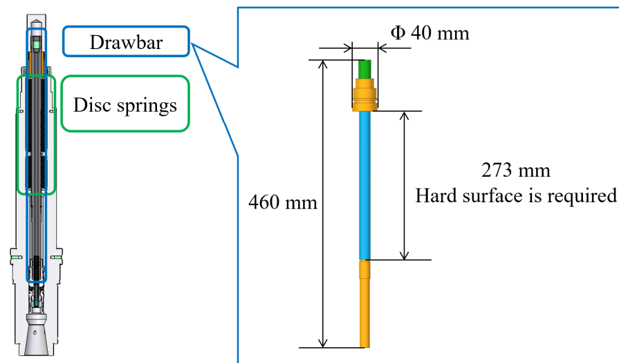
Fig. 6.1 Appearance of a drawbar and disc springs.
