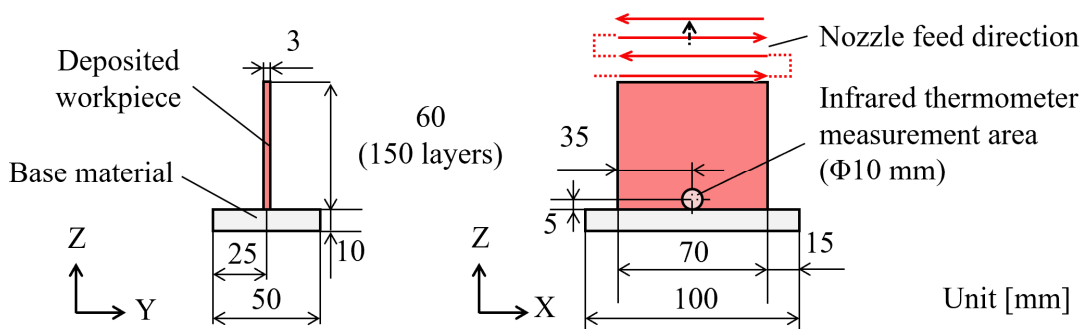
Fig. 5.3 Schematic of the wall deposition experiment.
