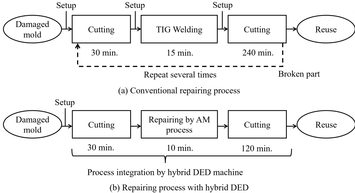
Fig. 2.2 Comparison between conventional and hybrid DED repairing process.
