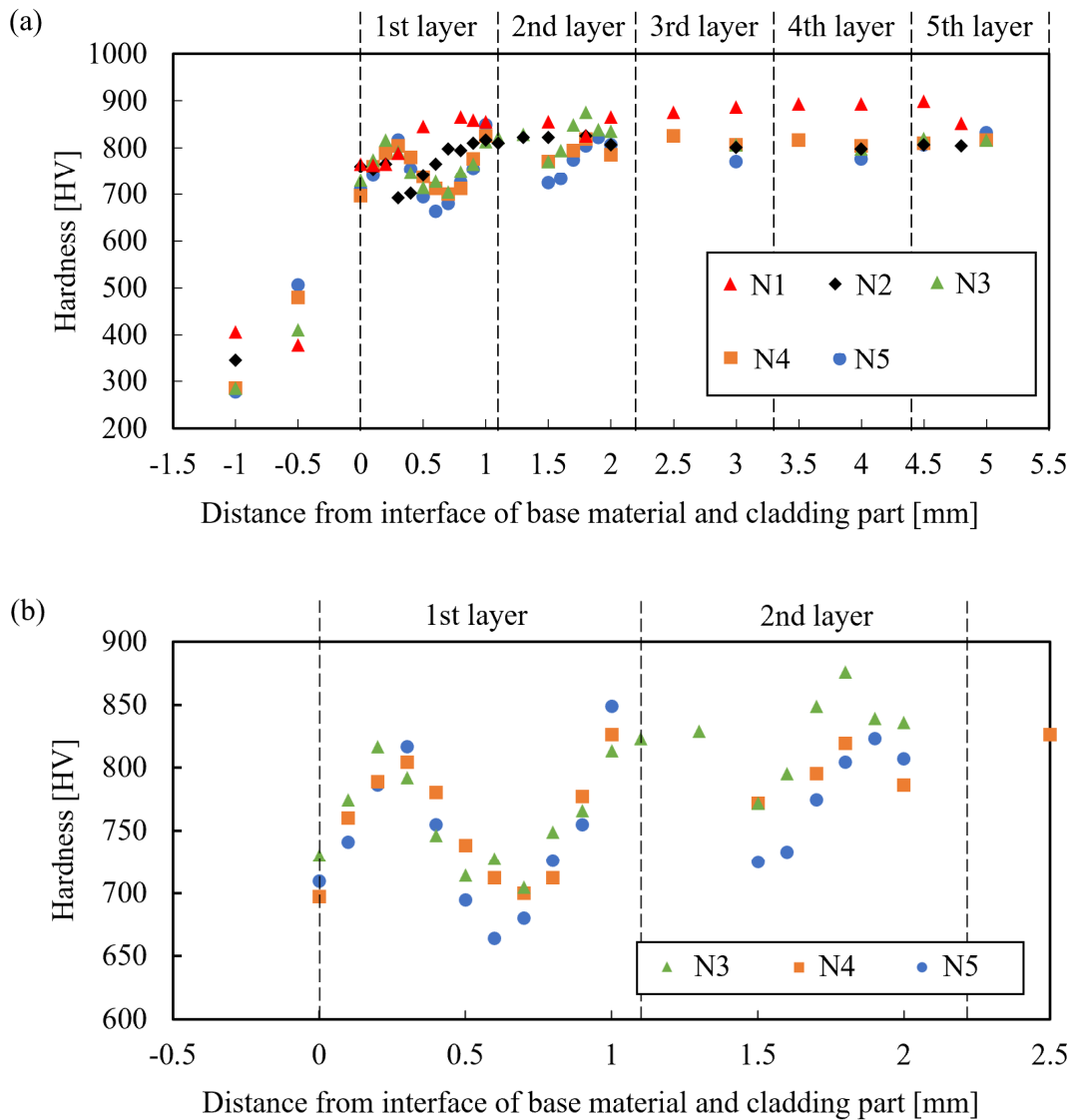
Fig. 5.9 Measured hardnesses for (a) all samples, (b) samples deposited with the same dwell time on the path level and different dwell times on the layer level.
