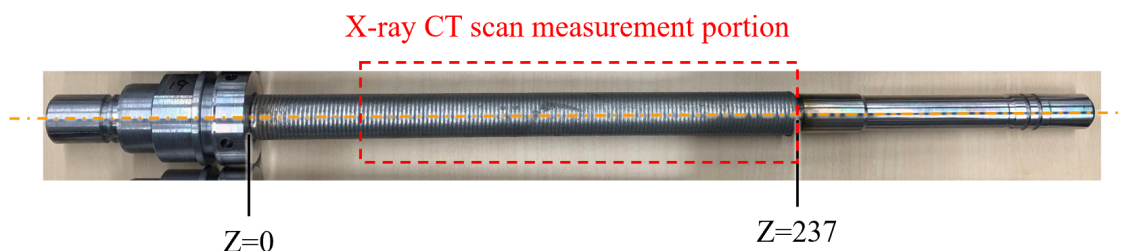
Fig. 6.5 Measurement portion of the X-ray CT scan of the drawbar.
