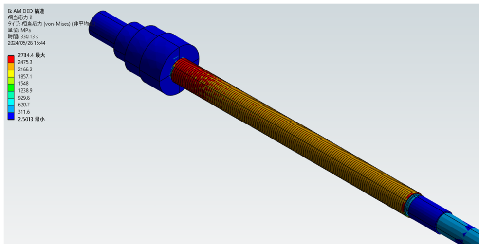
Fig. A.2.2 Stress distribution of the drawbar after completion of deposition.
