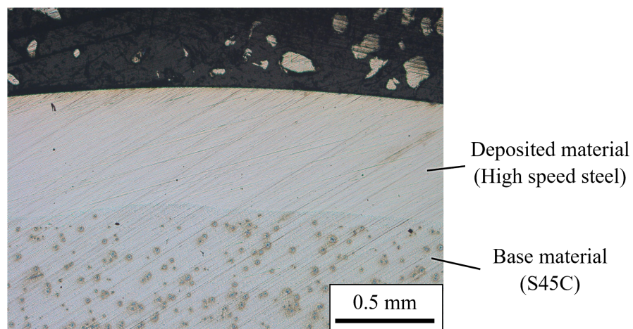
Fig. 6.8 Cross-section of the drawbar cladding by DED.
