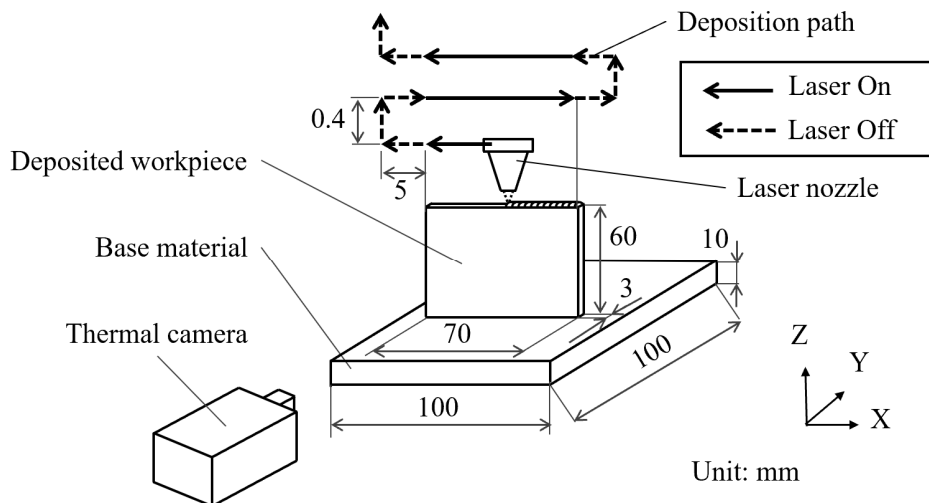
Fig. 3.1 Schematic of the measuring temperature setup and deposited layer size.
