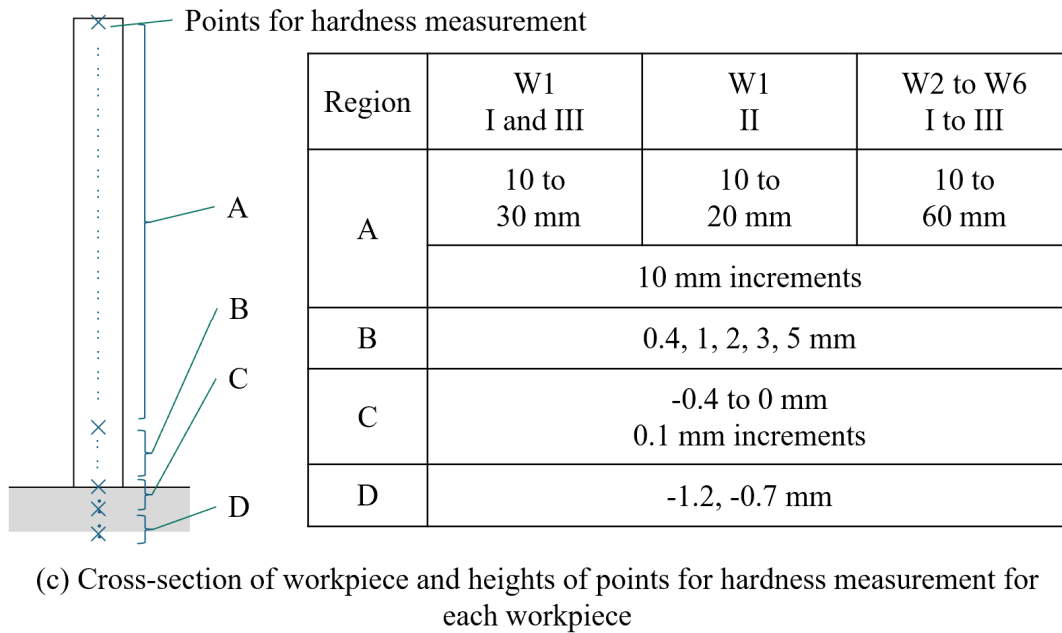
Fig. 3.7 Hardness measurement schematic.
