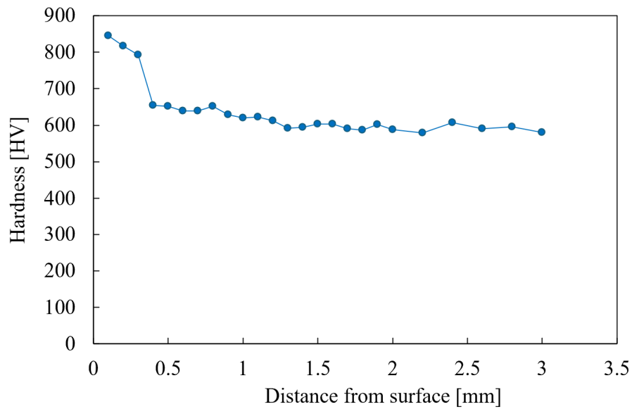
Fig. 6.7 Hardness measurement result of the drawbar coating by DED.
