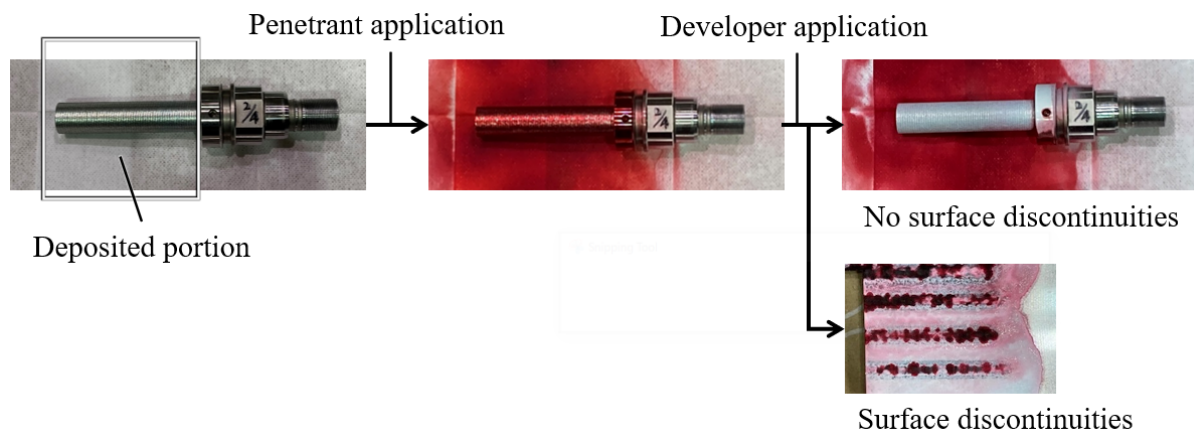
Fig. 6.9 Color-check procedures and result for the drawbar cladding by DED.
