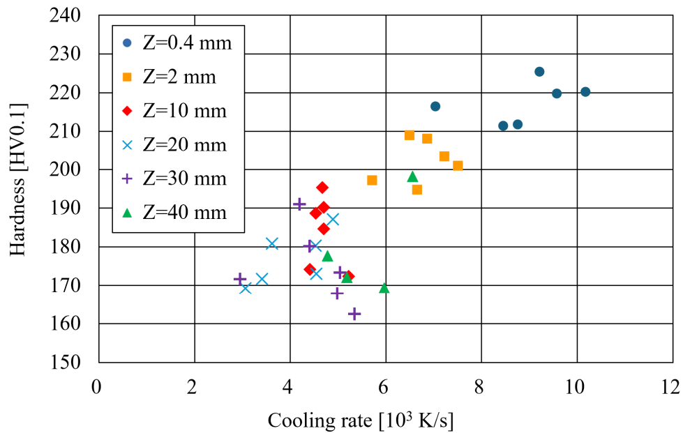
Fig. 3.20 Relationship between cooling rate and measured hardness.
