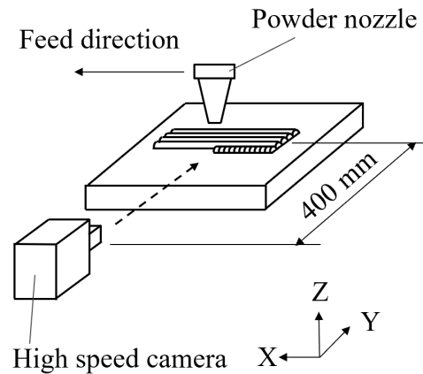
Fig. 4.3 Setup for crack observation using a high-speed camera.
