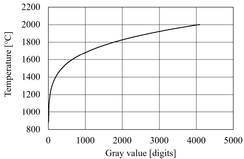
Fig. 3.3 Light intensity and temperature conversion curve.
