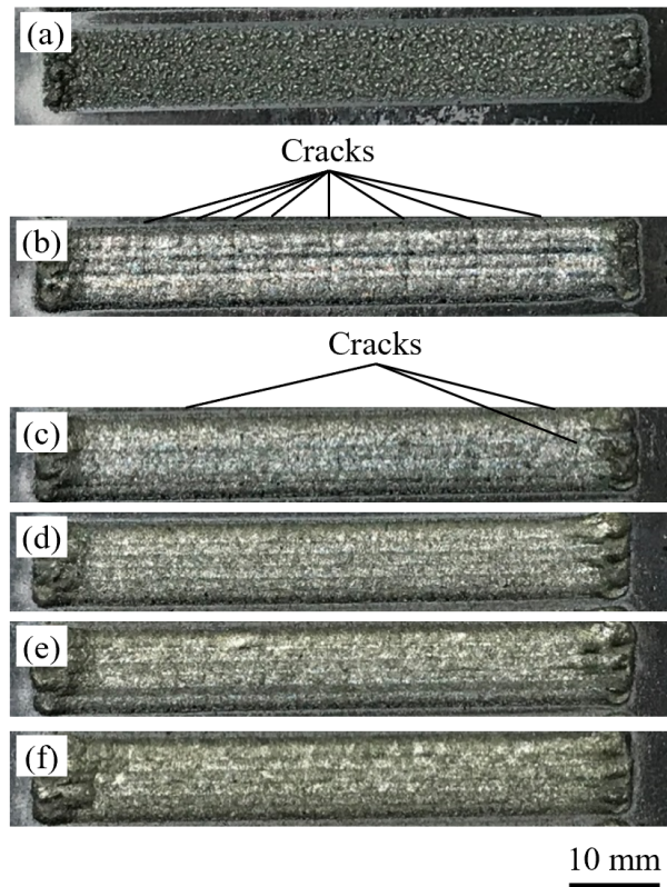
Fig. 4.7 Appearance of the test pieces at a preheating temperature of 500 °C and laser power of (a) 500, (b) 1000, (c) 1500, (d) 1750, (e) 2000, and (f) 2400 W.
