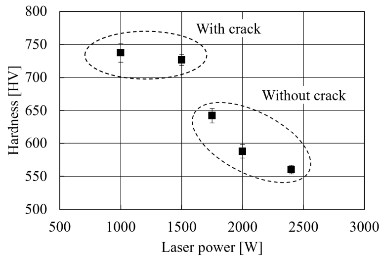
Fig. 4.8 Relationship between laser power and hardness of the test pieces (preheating temperature of 500 °C).
