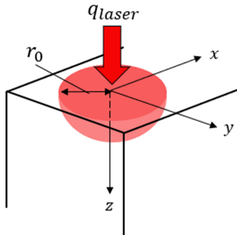
Fig. 5.1 Schematic of the local coordinate system in the laser heat input equation.
