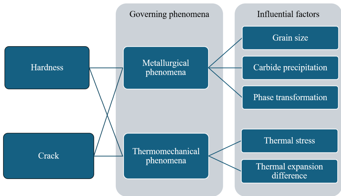
Fig. 2.8 Factors and physical phenomenon influencing hardness and cracking.
