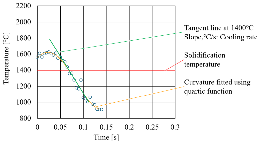
Fig. 3.6 Calculation results of the average temperature and estimation of the cooling rate for a dwell time of 9 s and deposition height of 0.4 mm.
