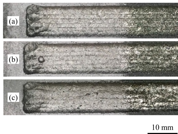
Fig. 4.5 Appearance of the test pieces at preheating temperature of (a) 400, (b) 500, and (c) 600 °C (laser power of 2400 W).
