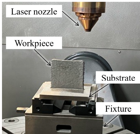
(a) Thin wall shaped workpiece deposited by DED
