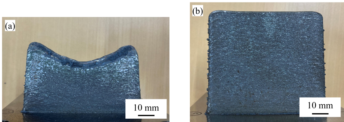
Fig. 3.8 Overview of samples deposited with interpass dwell times of (a) 0 and (b) 6 s.
