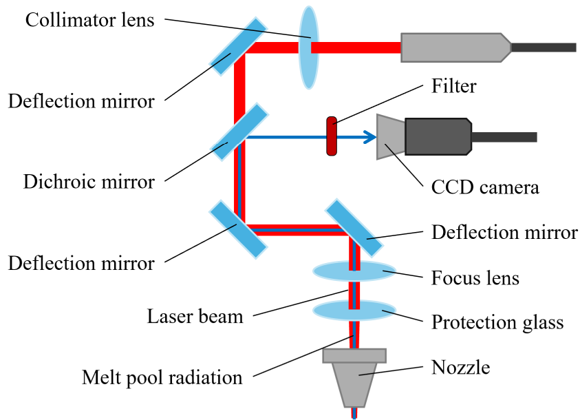
Fig. 3.2 Measurement of melt pool temperature distribution with CCD camera mounted along with the laser beam axis.
