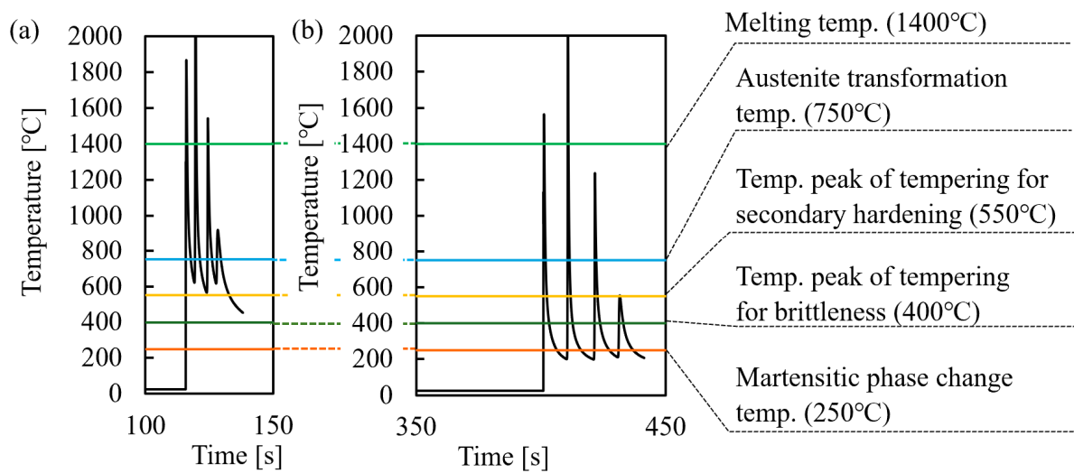
Fig. 5.12 Thermal history simulated by thermal analysis for (a) N1 and (b) N5 (4.5 mm height).
