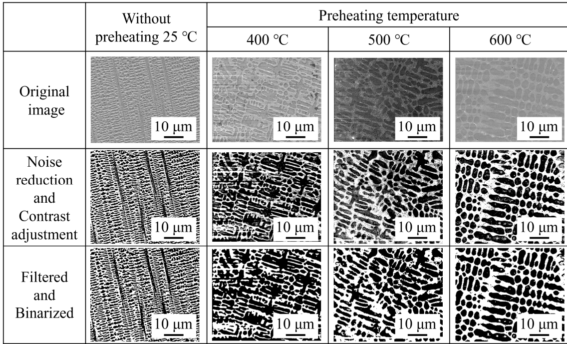
(a) Test pieces deposited with different preheating temperature
