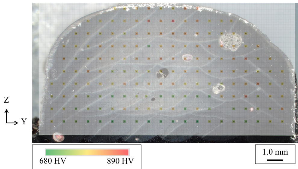
Fig. 5.7 Entire hardness map of the N5 cross-section.
