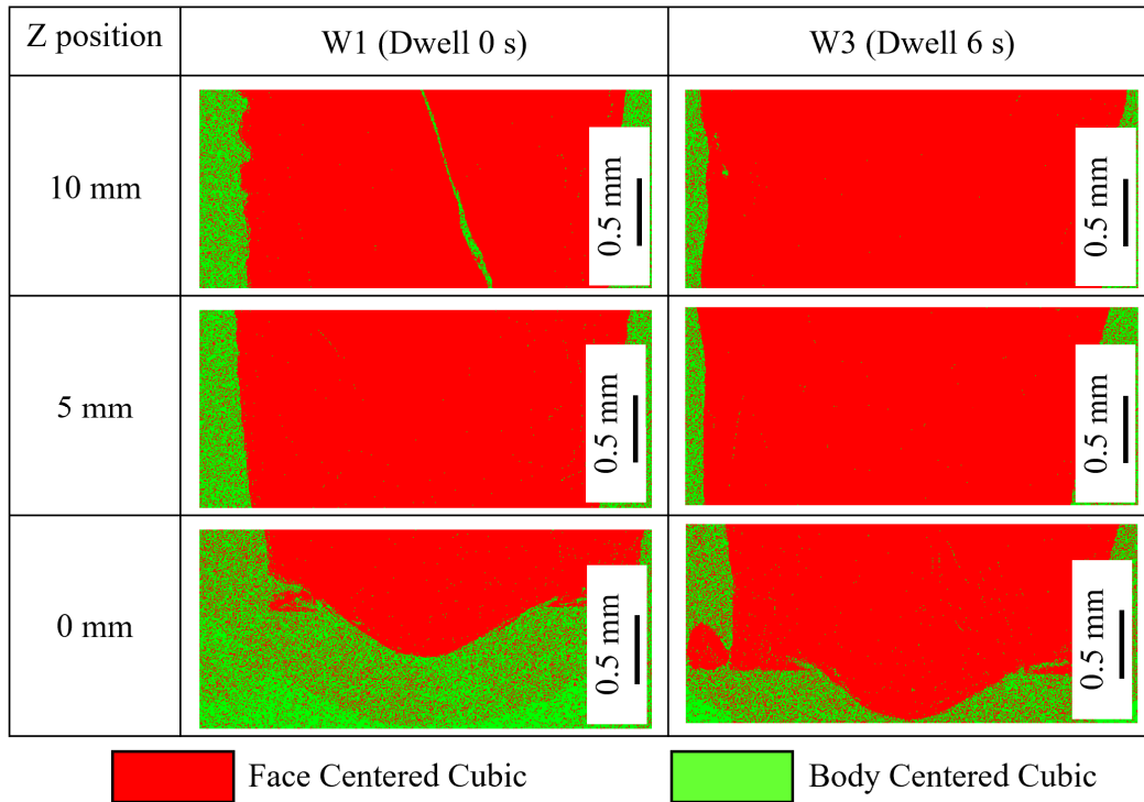
Fig. 3.17 Phase maps observed by EBSD for workpieces W1 and W3.
