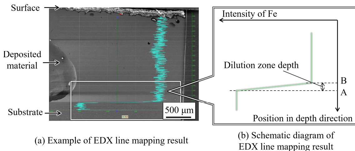
Fig. 4.14 EDX line mapping example of Fe intensity and a schematic thereof.
