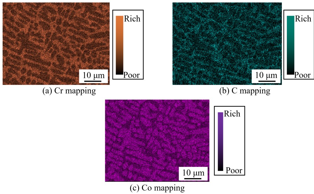
Fig. 4.11 EDX mapping images of the test piece deposited with a preheating temperature of 500 °C and laser power of 2400 W (measurement area is B as for Fig. 4.10).
