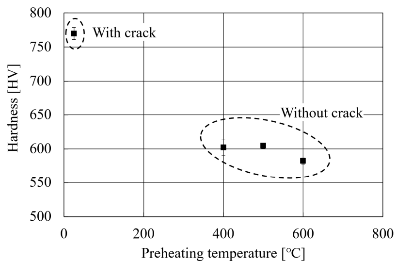
Fig. 4.6 Relationship between the preheating temperature and hardness of the test pieces (laser power of 2400 W).
