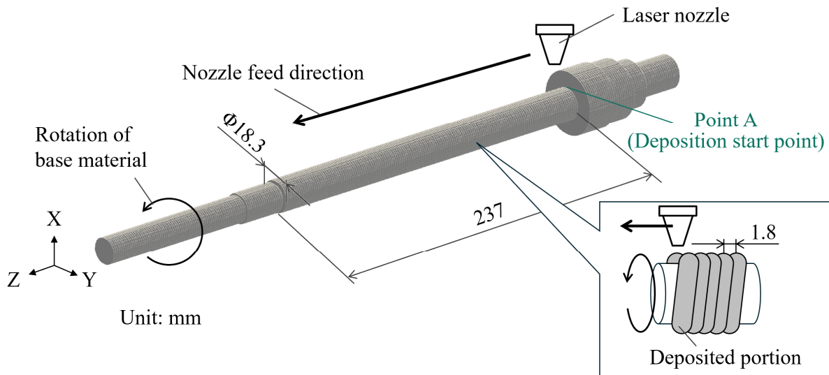
Fig. 6.2 Schematic of DED cladding on a drawbar.
