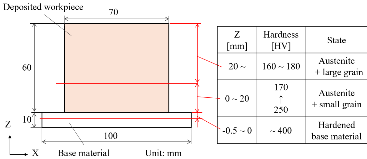
Fig. 3.19 Schematic of the hardness, phase composition, and grain size changes as well as deposition height.
