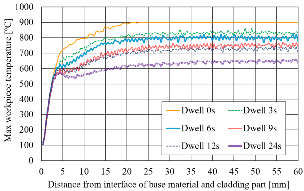
Fig. 3.12 History of maximum workpiece temperature for each dwell time condition.
