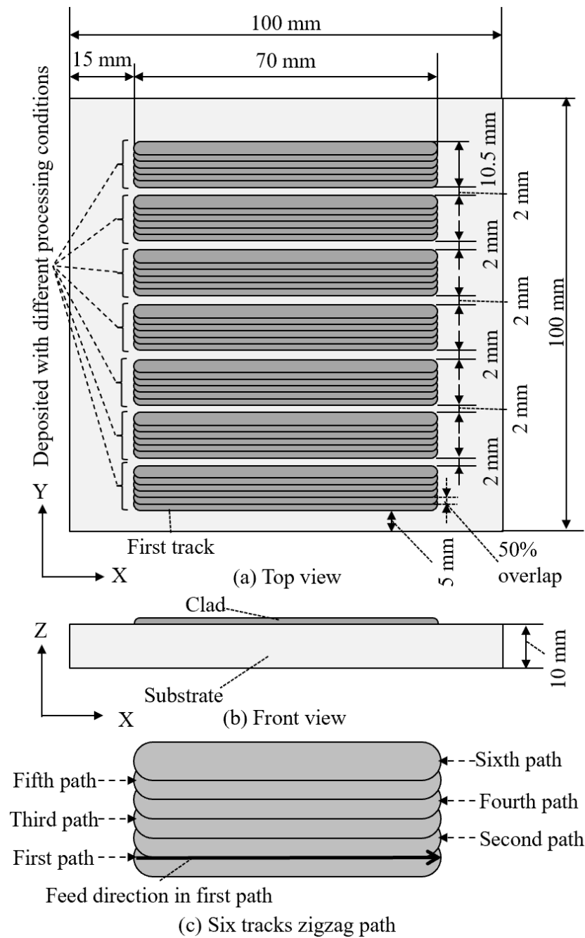
Fig. 4.2 Schematic of the deposition process and path pattern.
