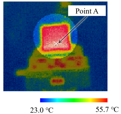
(b) Temperature distribution of deposited workpiece measured by a thermal camera
