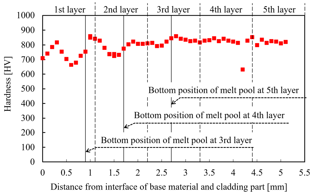
Fig. 5.11 Comparison between the measured hardness and bottom position of the melt pool at each deposition layer estimated by thermal history analysis for N5.
