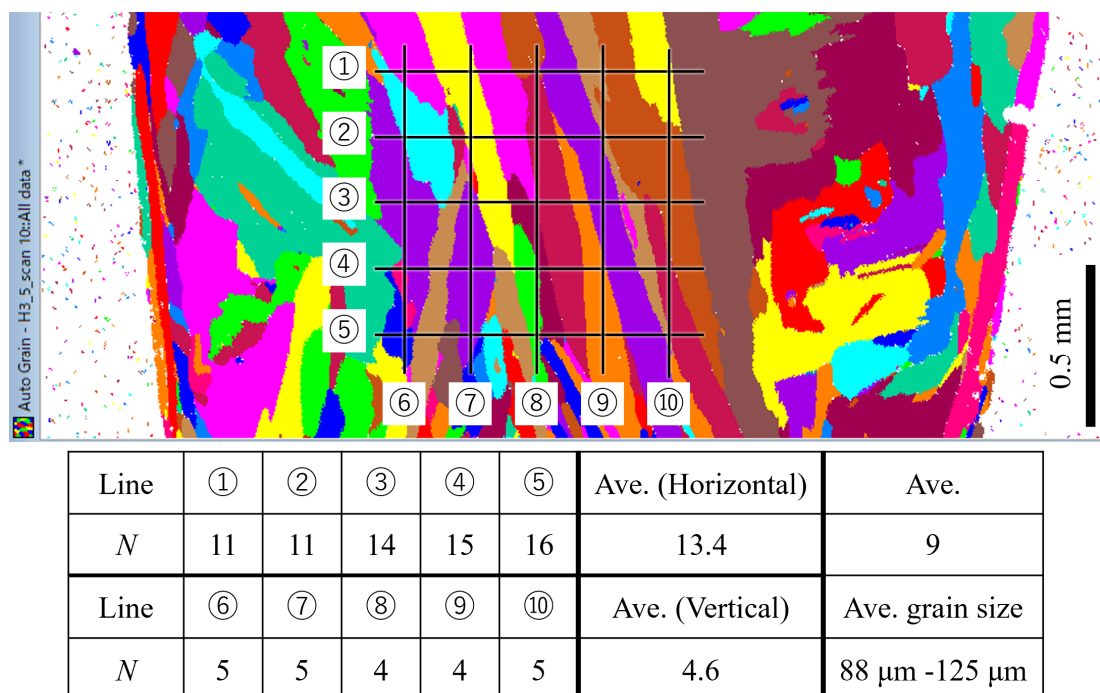
Fig. 3.15 Test lines on the inverse pole figure for evaluating grain size for W1, Z = 5 mm.
