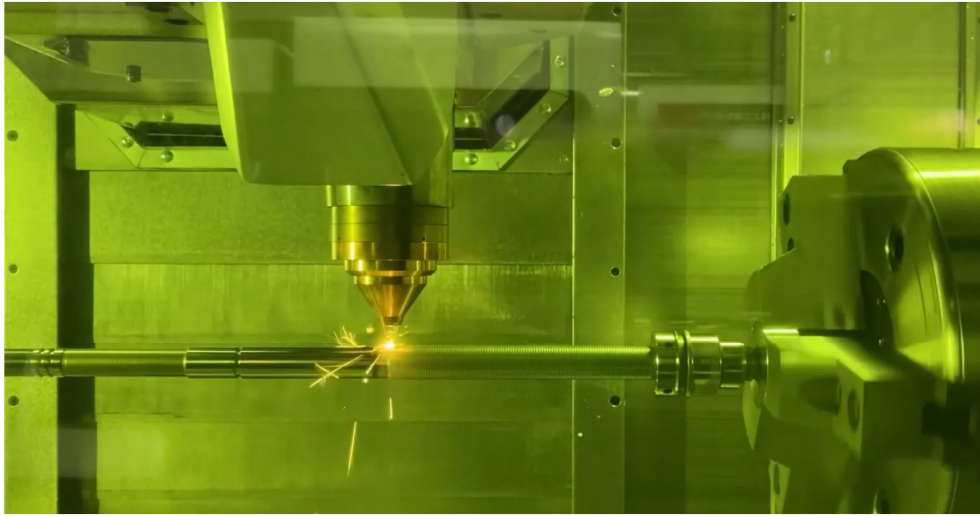
Fig. 6.4 View of the high-speed steel coating of the drawbar.
