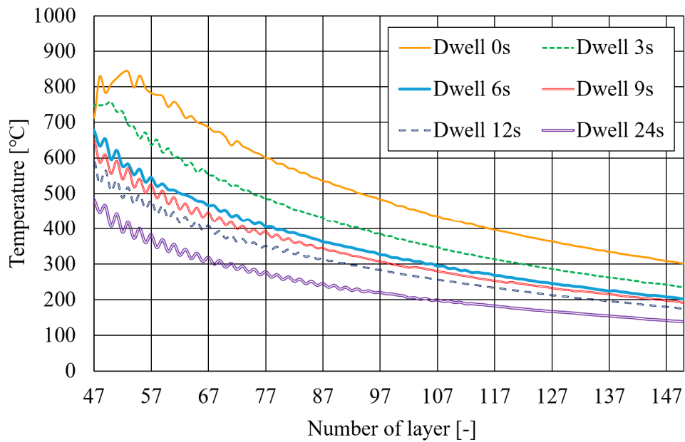
Fig. 3.13 History of workpiece temperature at a fixed point for each dwell time.
