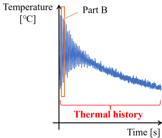
(c) Temperature change during deposition process at Point A
