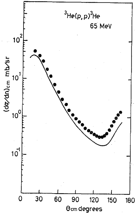
Fig. 2. Differential cross section in elastic p\text{-}^3\text{He} scattering at 65 MeV. Points are obtained from the experimental data in ref. 8. The curve is calculated using Eq. 9 with |\eta|^2 and the cross section of elastic p\text{-}d scattering 6) .
