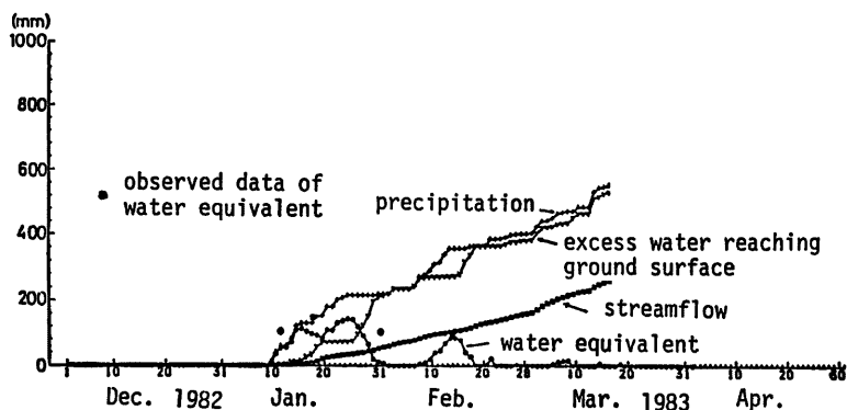
Fig. 11 Observed and synthesized water equivalent and excess water reaching the ground surface etc. at 1983 (by the improved model)
