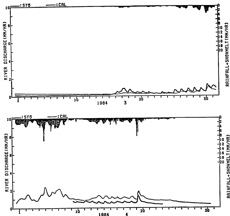
Fig. 24 Observed and synthesized hourly streamflows at 1984
