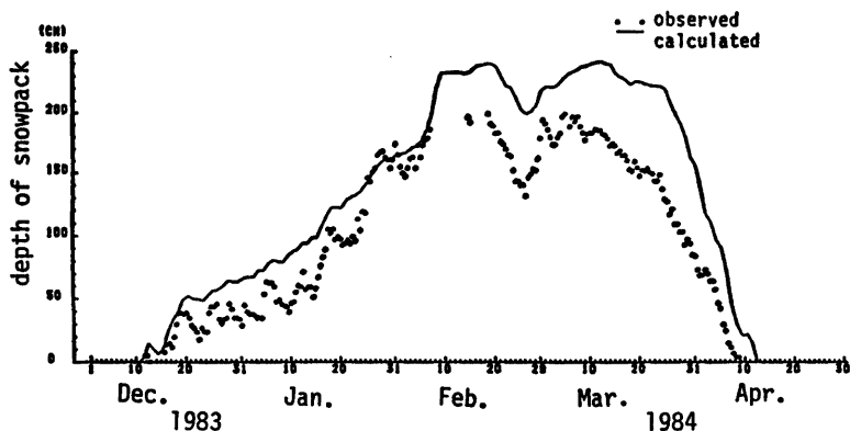
Fig. 6 Observed and synthesized snow depths at 1984 (by the previous model)
