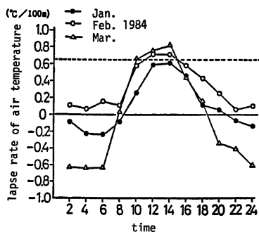
Fig. 20 Diurnal changes in the lapse rate of air temperature with elevation
