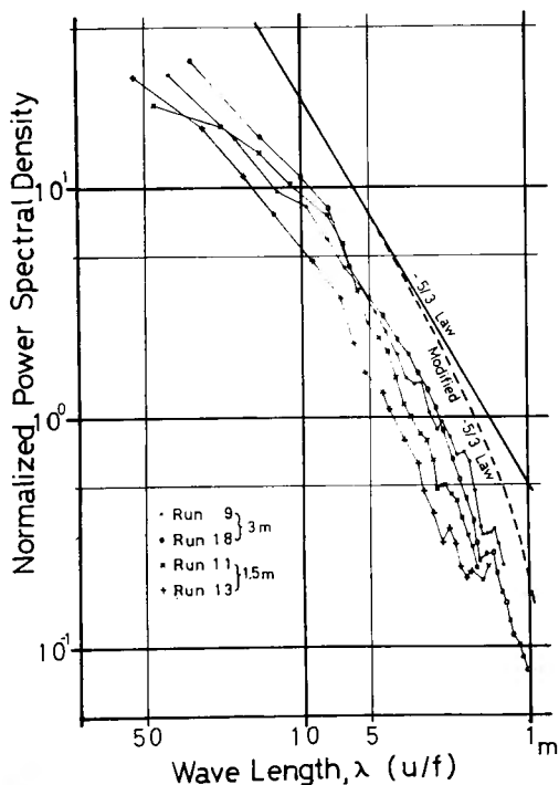
Fig. 4. Normalized power spectra of the vertical wind velocity components observed by a sonic anemometer with path length of 50 cm. The dotted line shows -5/3 law modified for attenuation caused by the line averaging character of the sound path length.
