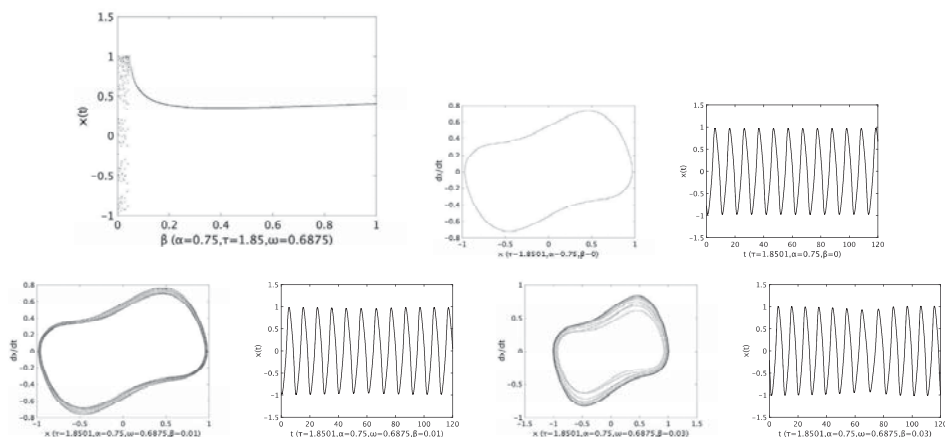
図 1: When \beta \leq 0.034 almost periodic waves are observed by numerical simulation ( \alpha = 0.75, \tau = 1.85, \omega = 0.6875 ).
