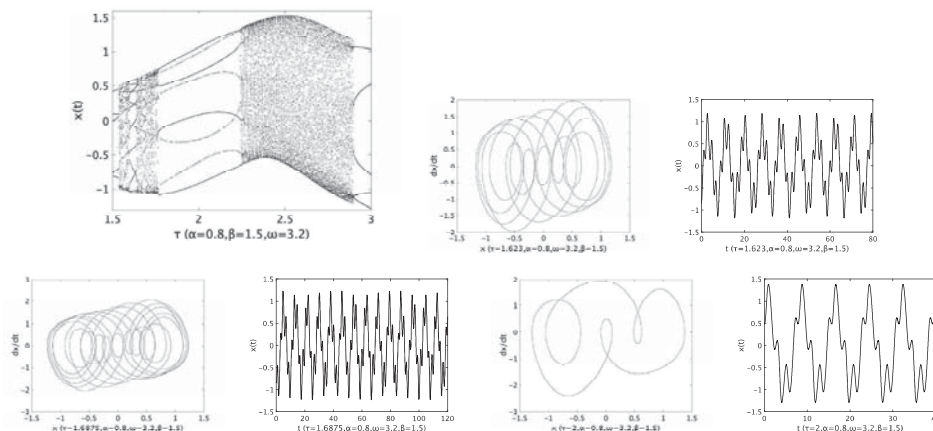
図 3: Stroboscopic bifurcation diagram obtained by numerical integration
