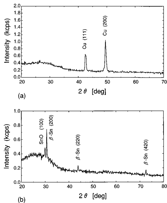
FIG. 2. X-ray-diffraction patterns of the films which were obtained by thermal decomposition of (a) \text{Cu}_3\text{N} film at 470 °C for 10 min and (b) \text{SnN}_x film at 550 °C for 30 min on a borosilicate glass substrate.
