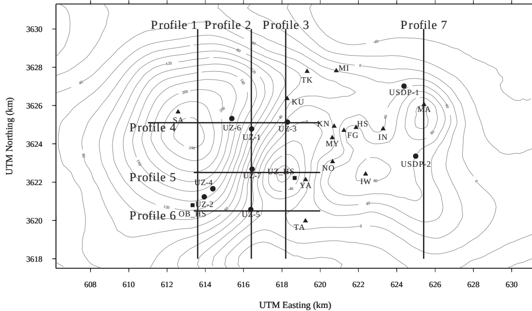
Fig.3. Terrain corrected reduced-to-the-pole magnetic anomaly map of box A, and the locations of profiles of forward modeling. Contour interval is 20 nT.
