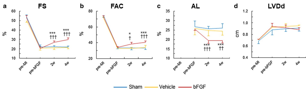
Fig. 1 Echocardiograms of cardiac function after bFGF–GHS treatment on rat chronic MI. a, b The left ventricular contractile function assessed by FS ( a ) and FAC ( b ) at 2 and 4 weeks after treatment. c Akinetic length assessed by AL at 2 and 4 weeks after treatment. d The diameter of left ventricle assessed by LVDd. * P < 0.05 ,
