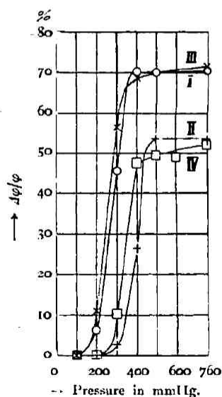
Fig. 9—Influence of external air pressure (Part 2).
