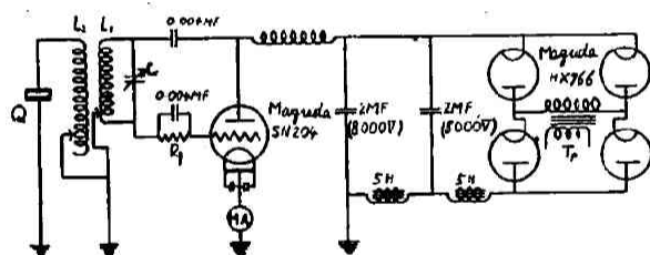
Fig. 1—Electric circuit for generating ultrasonic waves: Q, Quartz (dia.=40 mm, 800 KHz); C, 1000 MMF (5000V): L p , dia.=22 cm, 21 turns; L s , dia.=11 cm, 89 turns: R g , 10,000Ω; T, step up to 1,500V.
