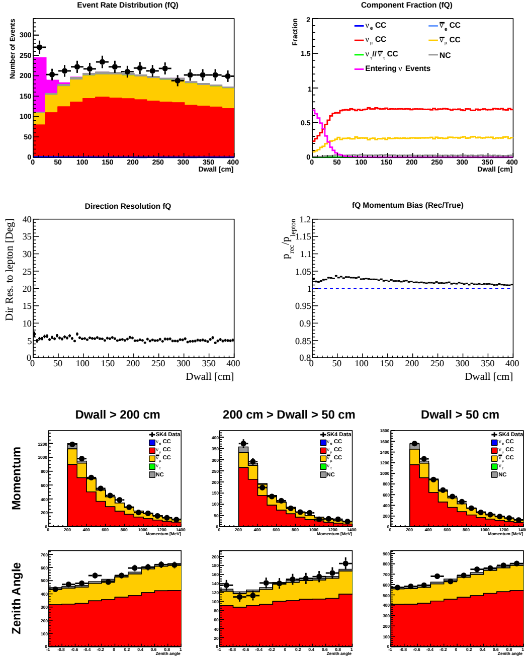
FIGURE B.4: Basic distribution for SubGeV single-ring \mu -like 1 decay-e sample reconstructed and selected by fitQun.
