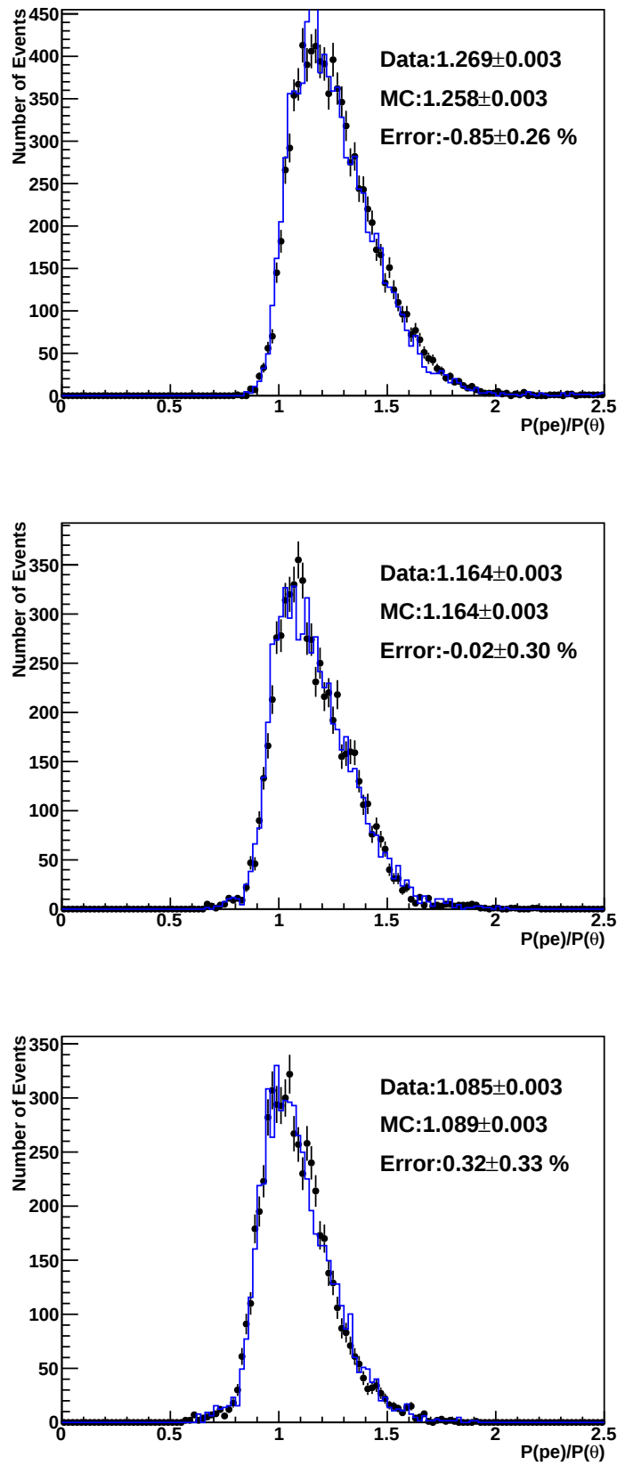
FIGURE 4.10: Distribution of p(\text{p.e.})/p(\theta) at each p(\theta) bin for data (black dots) and MC (blue line). From the top, the p(\theta) range is 200-280 MeV/c, 280-360 MeV/c and 360-440 MeV/c, respectively. MC are normalized to data by area.
