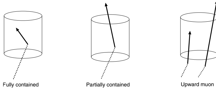
FIGURE 5.1: Schematic view of observed atmospheric neutrino in SK. Dashed lines represent the track of atmospheric neutrinos, while the solid lines show the lepton’s track.
