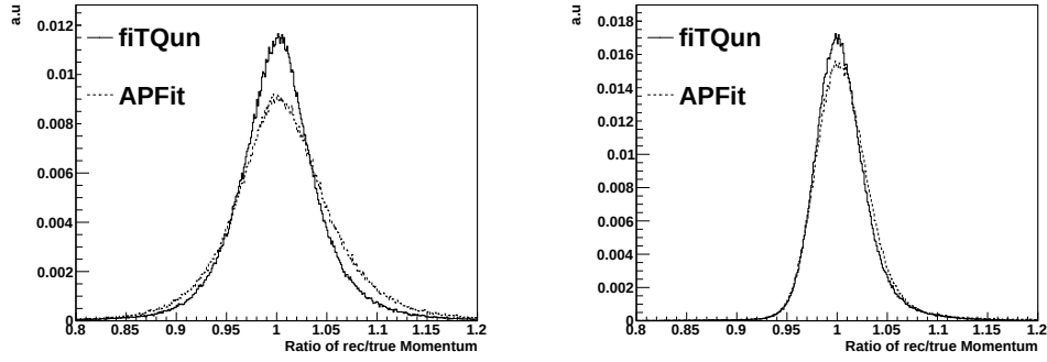
FIGURE 6.8: Single-ring electron (left) and muon (right) momentum resolution for FC CCQE events in atmospheric neutrino MC, compared between APFit (dashed line) and fiTQun (solid line). The bias (resolution) is defined as the mean (RMS) value of the ratio distribution between the reconstructed momentum and true momentum.
