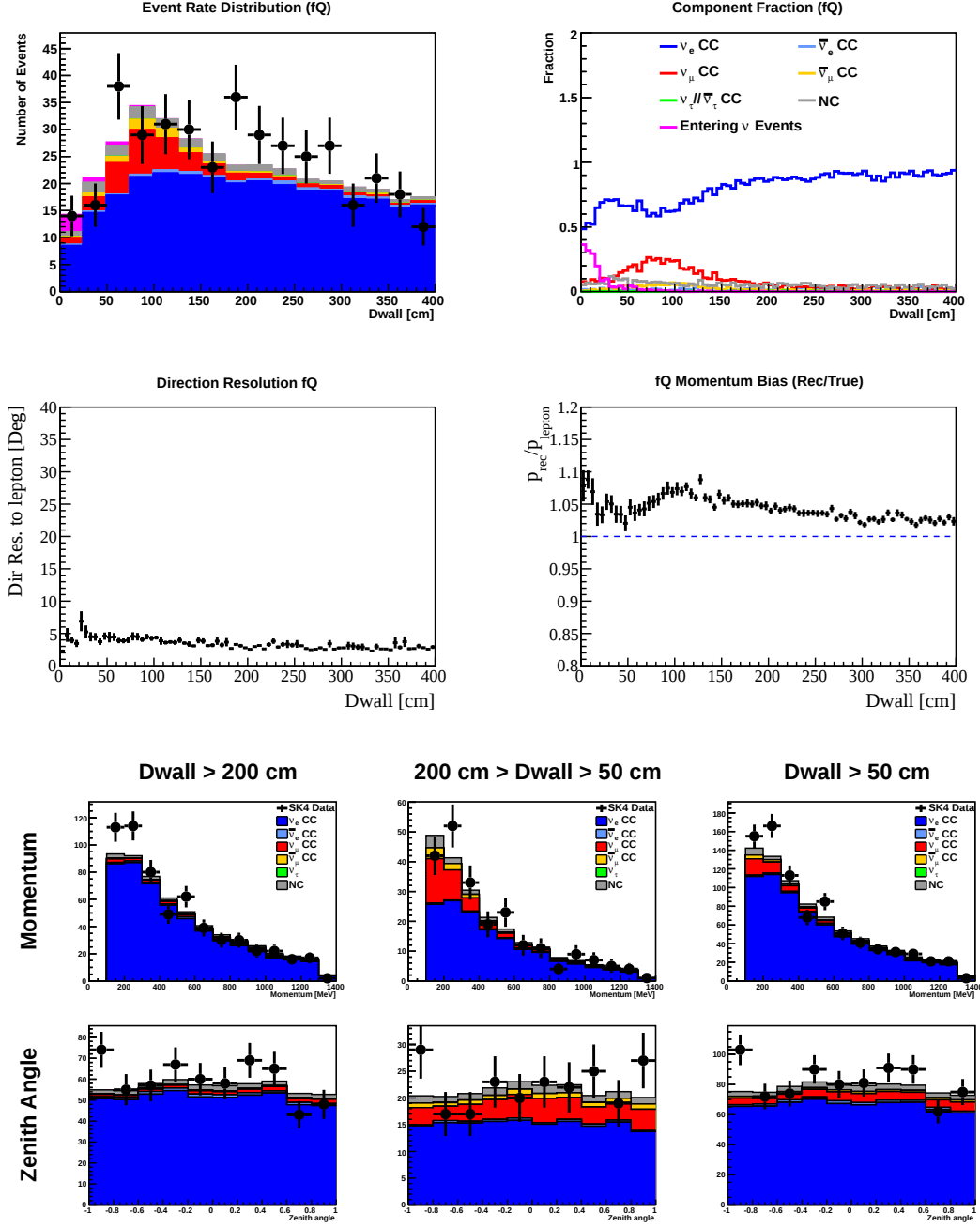
FIGURE B.2: Basic distribution for SubGeV single-ring e -like with 1 or more decay- e sample reconstructed and selected by fitQun.
