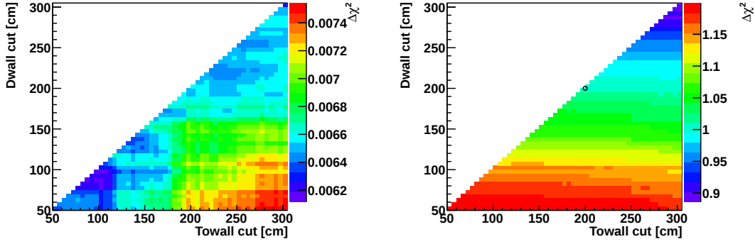
FIGURE 7.16: Sensitivity to reject wrong mass hierarchy. True mass hierarchy is NH. The left figure shows the contribution from sub-GeV single-ring e-like 1 decay sample, while the right figure shows the total sensitivity from all samples. The open circle at (200,200) in right figure represents the sensitivity at the FV cut used in previous APFit analysis.
