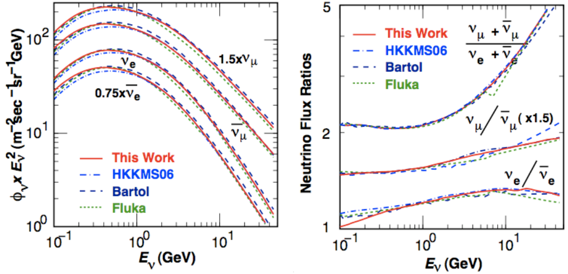
FIGURE 3.2: Atmospheric neutrino fluxes (left) and flavor ratio (right) after averaging over all directions. The prediction based on Honda 11 flux is shown by red solid line, while the result of the Bartol flux and the FLUKA flux are represented by dashed line and dotted line. Taken from [10].
