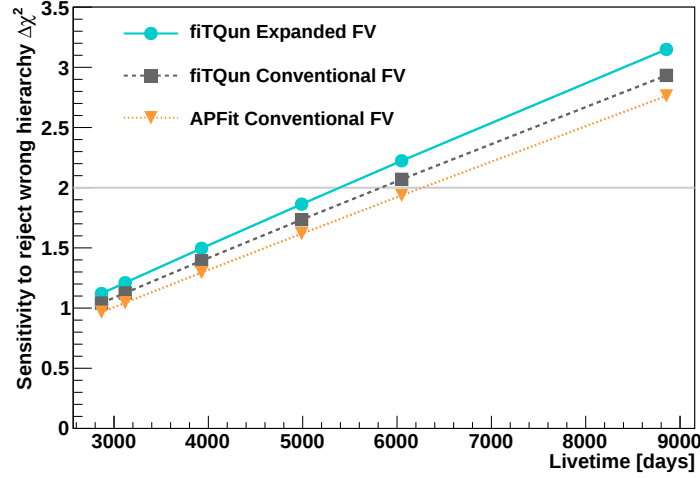
FIGURE 8.1: Median expected sensitivity to mass hierarchy for different livetime. Normal hierarchy is assumed to be true and the true value of \sin^2 \theta_{23} is assumed to be 0.5. Here the value of \sin^2 \theta_{13} is fixed to 0.0210. The result of the events reconstructed by fiTQun within the conventional FV and expanded FV are denoted by the gray and blue lines. The sensitivity with events reconstructed by APFit algorithm and the conventional FV is denoted by the orange line.
