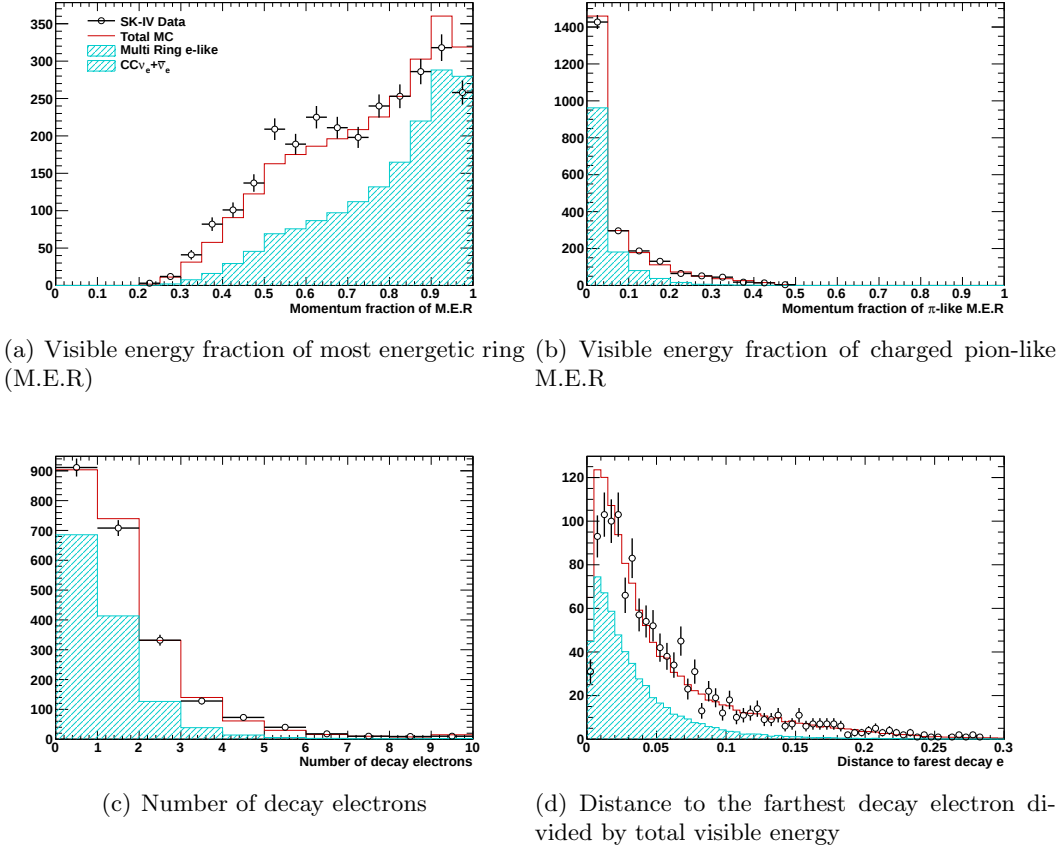
FIGURE 7.4: Distributions of the variables used in the multi-GeV multi-ring e -like (MME) likelihood for SK-IV. Shaded histogram represents CC\nu_e + \bar{\nu}_e , red solid line represents total atmospheric neutrino MC and open circle indicates the distribution of data. Error bars represent the statistical uncertainty of the data.
