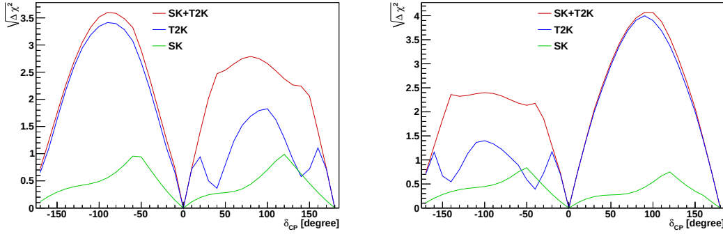
FIGURE 8.5: Sensitivity to CP violation ( \sin \delta_{CP} \neq 0 ) as function of true \sin \delta_{CP} . The true mass hierarchy of left figure is assumed to be normal hierarchy, while for right figure it is assumed to be inverted hierarchy. The green, blue and red lines represent the sensitivity with atmospheric neutrino only, accelerator neutrino only and combined analysis at the end of year 2026, respectively.
