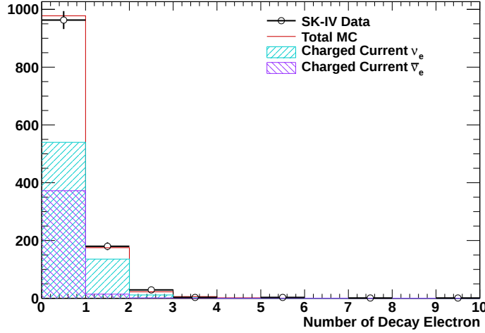
FIGURE 7.3: Distribution of number of decay electrons in both data and MC for SK-IV multi-GeV single-ring e -like sample. Cyan (magenta) shaded histogram represent the distribution of CC\nu_e ( CC\bar{\nu}_e ) events, red solid line represents total atmospheric neutrino MC and open circle indicates the distribution of data. Error bars show the statistical uncertainty of data.
