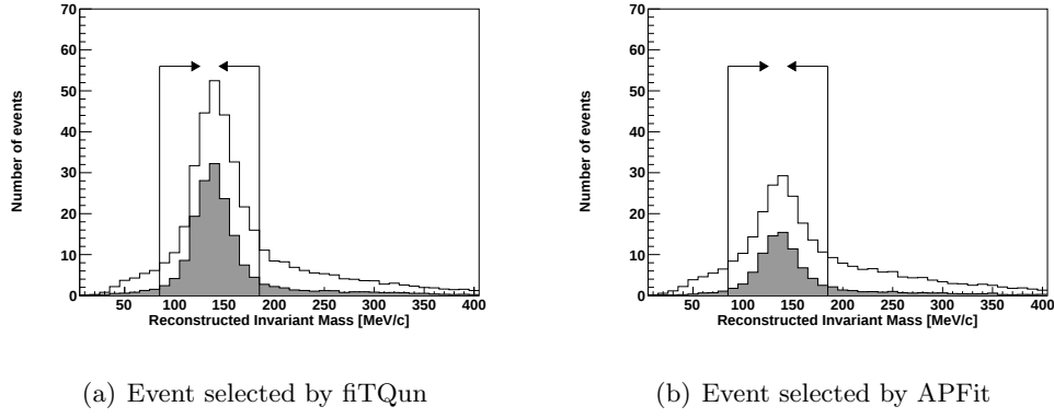
FIGURE 6.13: Reconstructed invariant mass calculated based the second and the third rings in order of energy for events with three e -like rings in the sub-GeV atmospheric neutrino MC sample. Left figure shows the events reconstructed by fiTQun, and right figure is for the events reconstructed by APFit. True \text{CC}\nu_e1\pi^0 events are denoted by shaded histograms. The invariant mass range used for the event rate and purity calculation is shown by arrows. The reconstructed event vertex to the nearest ID wall ( D_{\text{wall}} ) is required to be larger than 200 cm.
