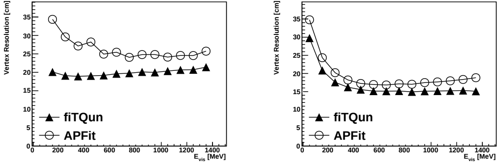
FIGURE 6.5: Vertex resolution of FC single-ring charged current quasi-elastic (CCQE) event as a function of visible energy. Left figure is for \text{CC } \nu_e events and right figure is for \text{CC } \nu_\mu events. The performance of fiTQun is indicated by the full triangles, while that for APFit is indicated by the open circles.
