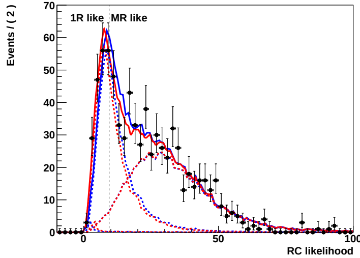
FIGURE 7.26: Ring counting likelihood distribution for multi-GeV e-like events in the new region ( D_{\text{wall}} from 50 cm to 200 cm). The original p.d.f constructed from MC (blue line), the fitted p.d.f. (red line) and the data (points) are shown. The dashed lines show the contribution from different components: true single-ring subsample and true multi-ring sample. The true number of rings is counted using only particles with energy more than 30 MeV above Cherenkov threshold in the final states. Error bars represent the statistical error.
