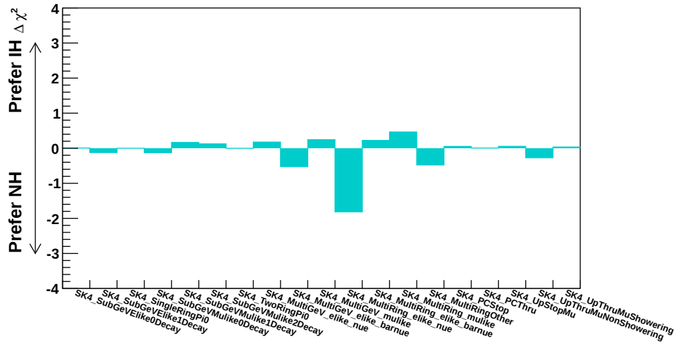
FIGURE 7.34: The preference for MH for each event types within expanded FV. The y-axis shows the difference of \chi^2 between normal hierarchy (NH) and inverted hierarchy (IH) contributed by each event sample at the best-fit oscillation parameters. The definition of the vertical axis is \Delta\chi^2 = \chi^2_{\text{NH}} - \chi^2_{\text{IH}} , which means that the negative value represent the preference for the normal hierarchy.
