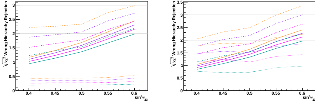
FIGURE 8.4: Sensitivity to mass hierarchy as function of true \sin^2 \theta_{23} . The solid lines (dotted lines) are the sensitivity with atmospheric neutrino only (accelerator neutrino only), while the dashed lines represent the result of joint analysis. The result shown in left figure assumes true \delta_{CP} = 0^\circ , while the right figure is for true \delta_{CP} = 270^\circ . The orange, purple, magenta and green lines represent the result at the end of year 2026, 2023, 2020 and 2017, respectively.
