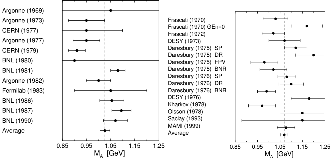
FIGURE 3.3: Axial mass M_A extractions. Left panel: From (quasi)elastic neutrino and antineutrino scattering experiments. The weighted average is M_A = (1.026 \pm 0.021) GeV. Right panel: From charged pion electroproduction experiments. The weighted average is M_A = (1.069 \pm 0.016) GeV. Taken from [11].
