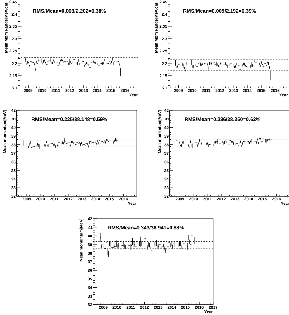
FIGURE 4.13: Time variation plots of the p/\text{range} of muon (top figures) and the momentum of decay electron (bottom three figures) for fitQun. The left two figures show the result for D_{\text{wall}} > 200\text{ cm} , while the right two figures are for D_{\text{wall}} > 50\text{ cm} . The bottom figure shows the time variation of the momentum of decay electron with 200\text{cm} > D_{\text{wall}} > 50\text{ cm} . The dashed line shows the range of average value with \pm 1\% error.
