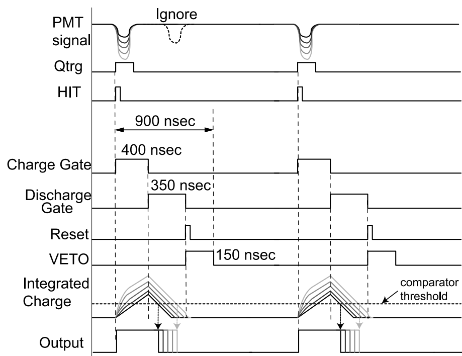
FIGURE 2.11: Timing chart for QTC operation. Taken from [9].
