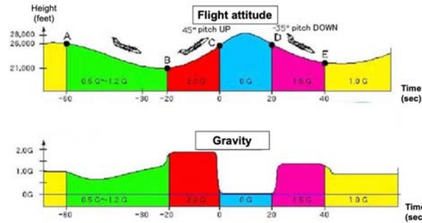
Fig. 3 Parabolic flight.
