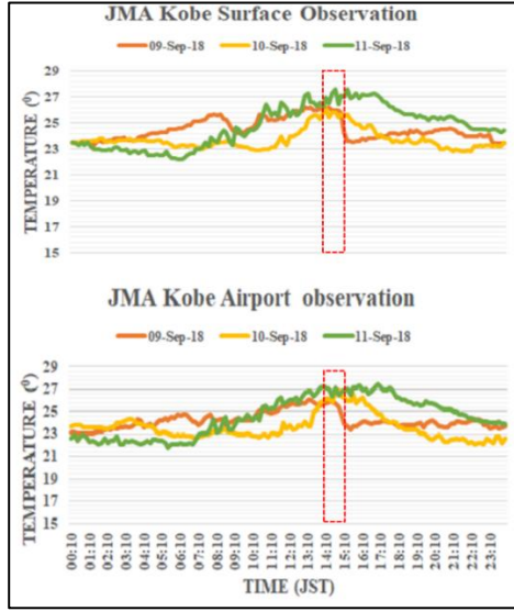
Fig. 3 Temperature observation from nearest JMA AMeDAS in Kobe area.
