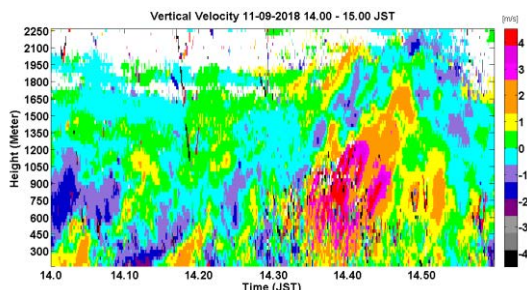
Fig. 1 BLR vertical velocity in 11 September 2018
