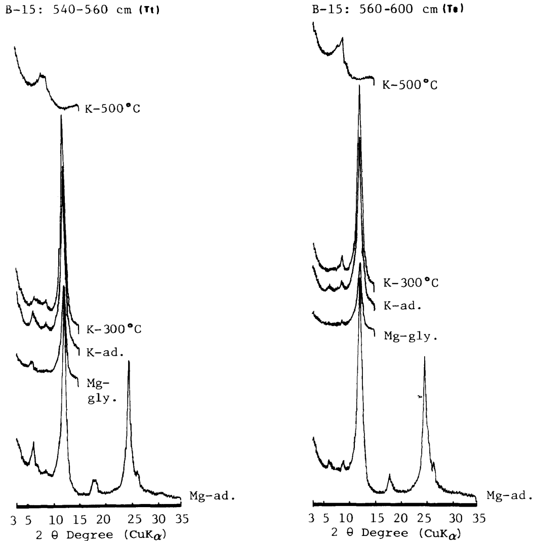
1-3 X-ray diffraction pattern of soil samples taken from two depths of profile B-15 of the ombrogenous peat zone
