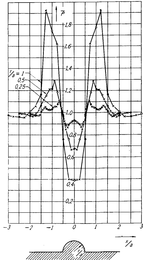
Fig. 22. Resistivity curves.
