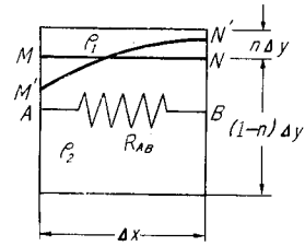
Fig. 6. Determining the value of resistors.
