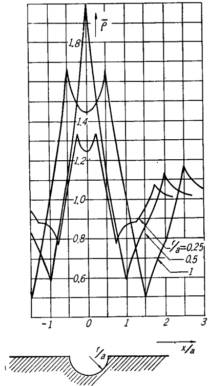
Fig. 30. Theoretical resistivity curves,
