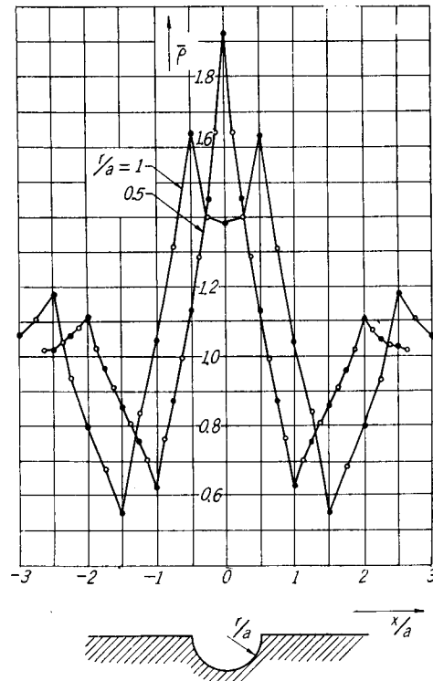
Fig. 25. Resistivity curves.
