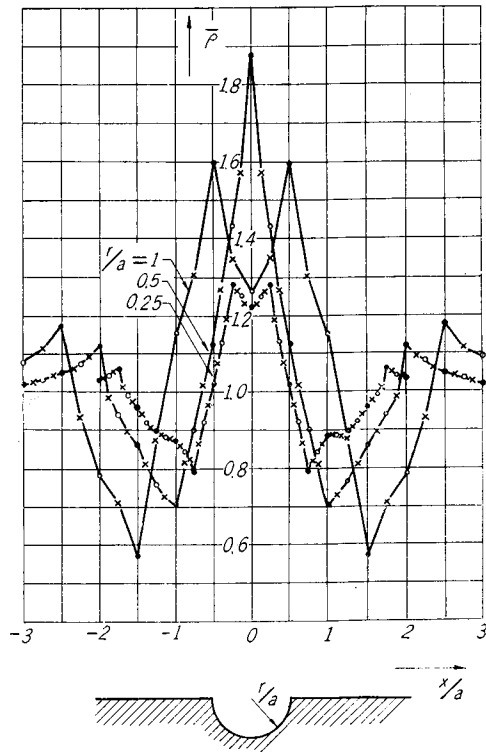
Fig. 27. Resistivity curves.
