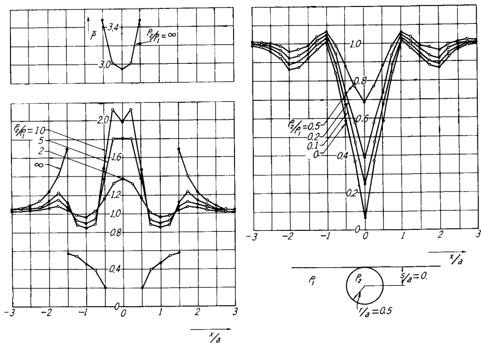
Fig. 14. Resistivity curves.
