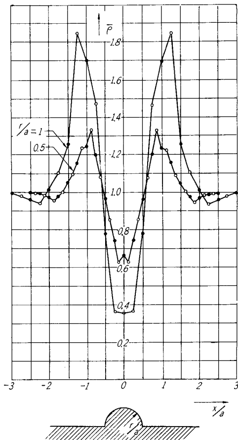
Fig. 18. Resistivity curves.
