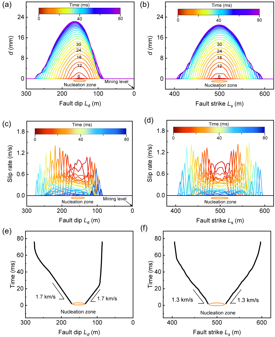
Fig. 4-12 Duration of slip and slip rate during fault rupture in Model_Cao with D_m = 60 m, P_L = 280 m, \mu_s = 0.375 , and \mu_d = 0.24 , C = 0.3 MPa. (a) Slip duration along the fault dip at L_s = 600 m; (b) Slip duration along the fault strike at L_d = 158 m; (c) Slip rate duration along the fault dip at L_s = 600 m; (d) Slip rate duration along the
