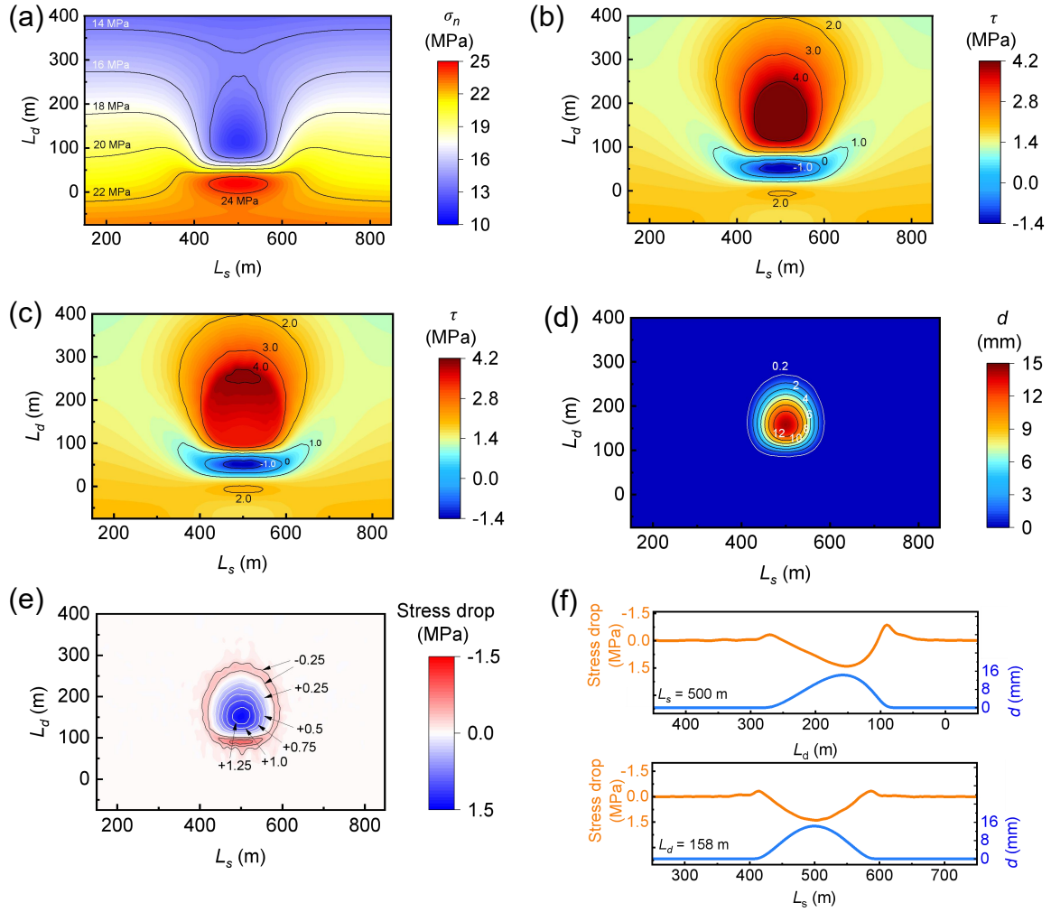
Fig. 4-8 Slip distribution and stress analysis on the fault plane with D_m = 60 m, P_L = 280 m, and \mu = 0.268 . (a) 2-D spatial variation of \sigma_n ; (b) 2-D spatial variation of \tau without slip ( \mu_s is considered infinite, numerically set as 100); (c) 2-D spatial variation of \tau ; (d) 2-D spatial variation of fault slip; (e) 2-D spatial variation of stress drop; (f) stress drop across fault strike ( L_s ) and fault dip ( L_d ) with specific focus at L_d = 158 m and L_s = 500 m.
