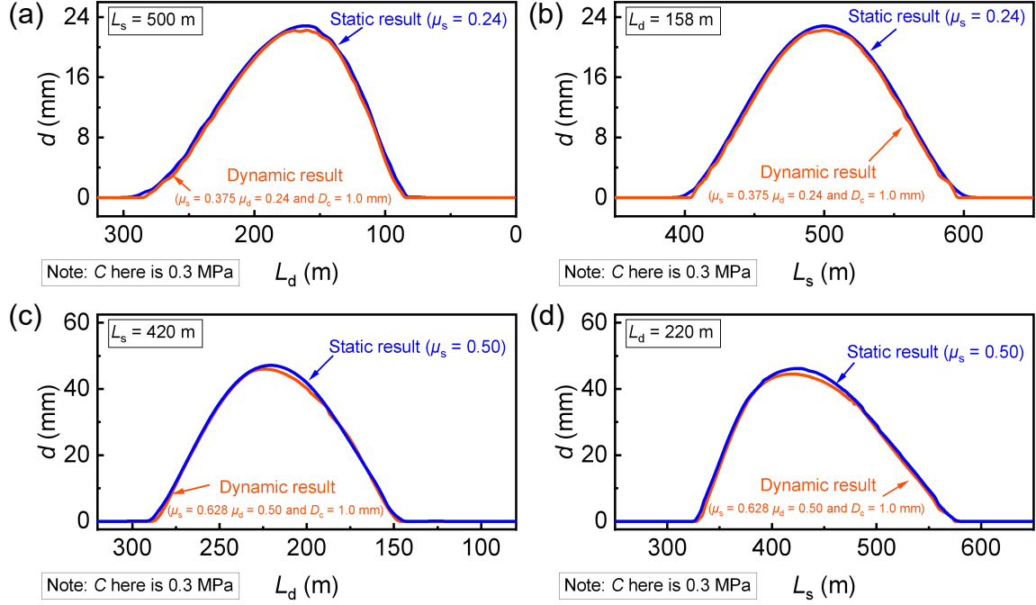
Fig. 4-18 Comparison of static and dynamic rupture stages in Model_Cao and Model_Cai.
