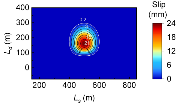
Fig. 4-19 Static modeling results from Cao et al.(2023) for \mu_s = 0.24 , C = 0.3 , and D_m = 60 m.
