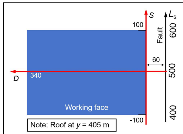
Fig. 4-23 Analysis of the local coordinates D and S on the working face during seismic wave vibrations. The analysis focuses on the position 1 m above the working face, at y = 405 m. Considering the distribution affected by wave fluctuations, I analyze
