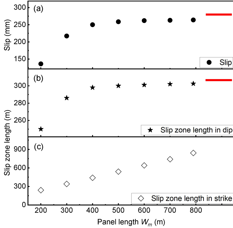
Fig. 3-13 Correlations of W_m with (a) maximum slip; (b) Slip zone length in dip-direction and (c) strike-direction. The red bars represent the 2-D plane strain result from Li et al. (2024a).
