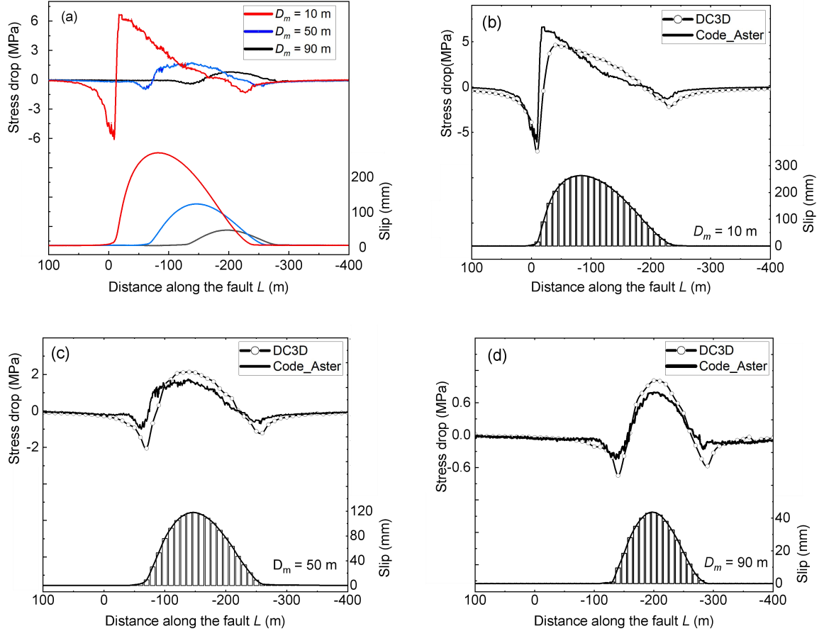
Fig. 2-10 Distribution of stress drop (top) and coseismic slip displacement (bottom) for different D_m under r_b = 2 , \mu_s = 0.7 , and \varphi = 30^\circ . (a) Stress drops and slip distributions for different D_m obtained from Code_Aster. Comparison of stress drop slip distributions between Code_Aster and DC3D for the case of (b) D_m = 10 m, (c) D_m = 50 m, and (d) D_m = 90 m. The bar graph at the bottom of the figure indicates the piecewise constant slip distribution used in DC3D, and the black curve is the coseismic slip obtained by the Code_Aster. (Reproduced from Li et al., 2024a)
