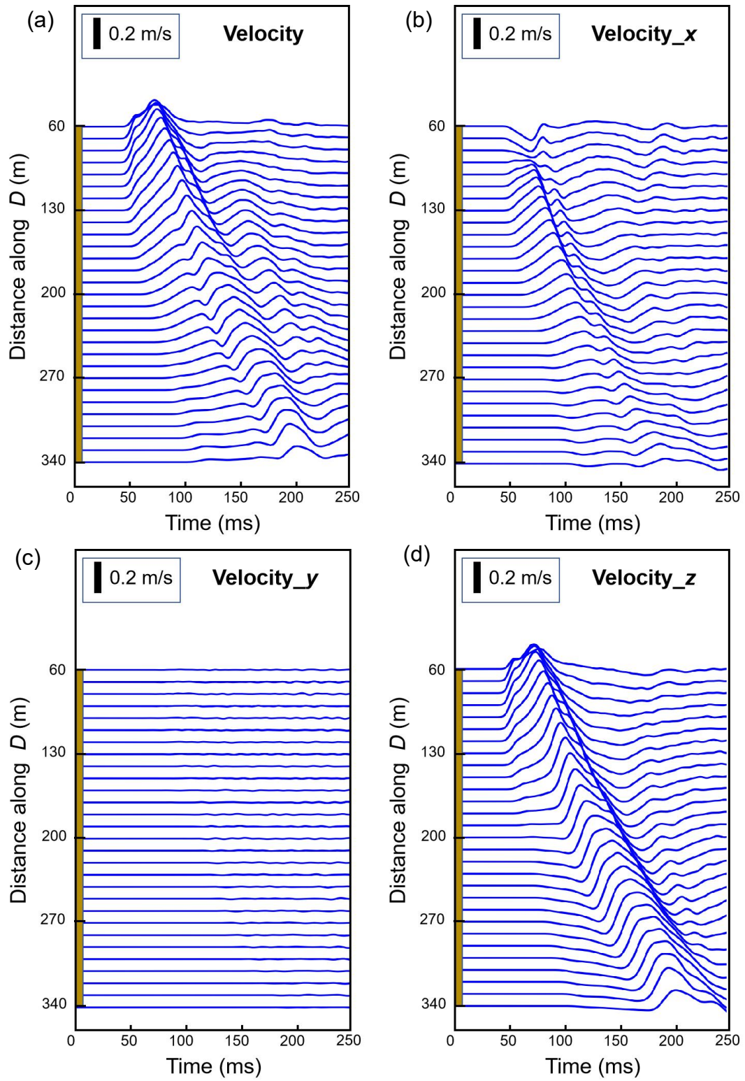
Fig. 4-24 Velocity at 1 m above roof induced by fault rupture in Model_Cao. a–d correspond to velocity and the x , y , and z components, respectively. A total of 29 points were plotted along D at 10 m intervals from the position S = 0 m.
