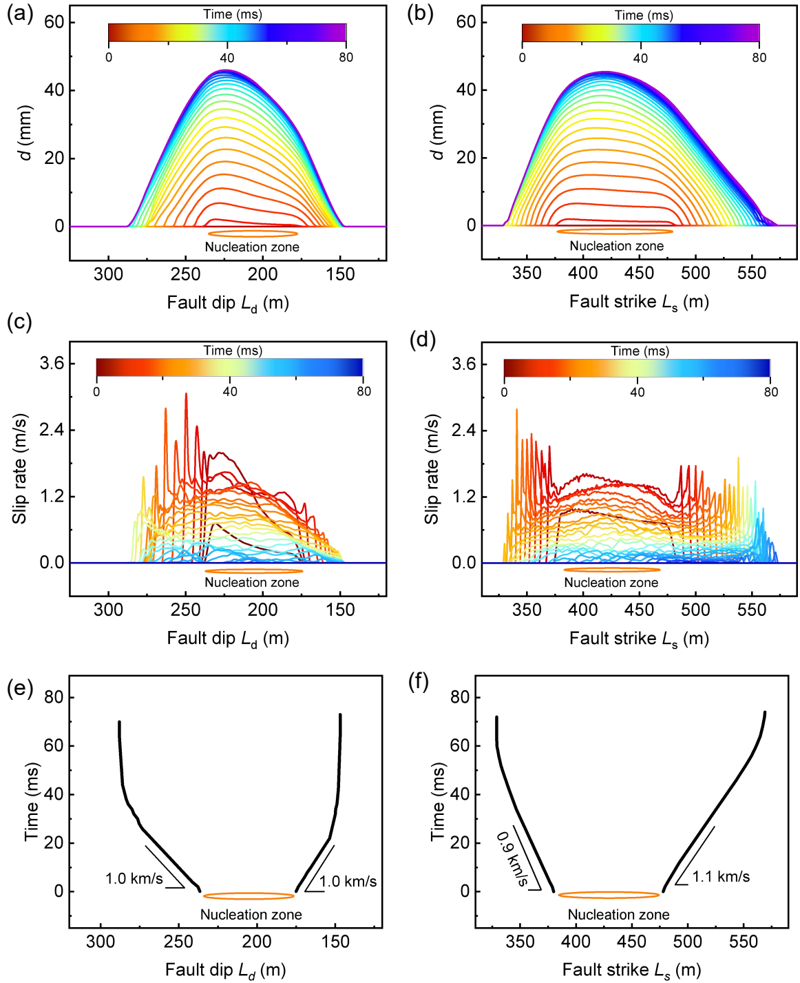
Fig. 4-15 Duration of slip and slip rate during fault rupture in Model_Cai with D_m = 60 m, P_L = 280 m, \mu_s = 0.628 , and \mu_d = 0.5 , C = 0.3 MPa. (a) Slip duration along the fault dip at L_s = 420 m; (b) Slip duration along the fault strike at L_d = 220 m; (c) Slip rate duration along the fault dip at L_s = 420 m; (d) Slip rate duration along the fault
