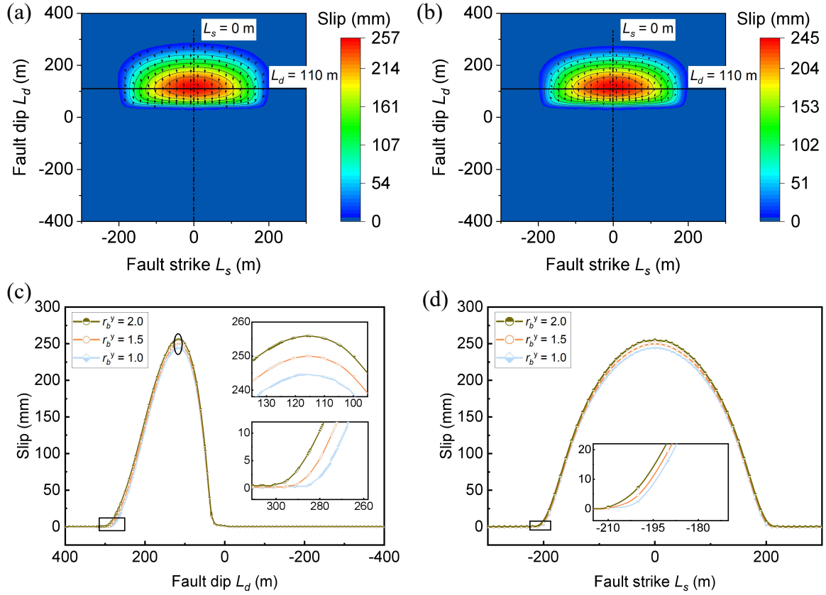
Fig. 3-6 Slip Variation under different \sigma_y with D_m of -30 m on the footwall side, \mu_s = 0.7 , and W_m = 400 m. (a) Slip distribution on the fault plane with \sigma_x = \sigma_y > \sigma_z ( r_b^y = 2.0 ); (b) Slip distribution on the fault plane with \sigma_x > \sigma_y = \sigma_z ( r_b^y = 1.0 ); (c) Slip sectional curves along the fault dip direction for the three cases at L_s = 0 m; (d) Slip sectional curves along the fault strike direction for the three cases at L_d = 110 m.
