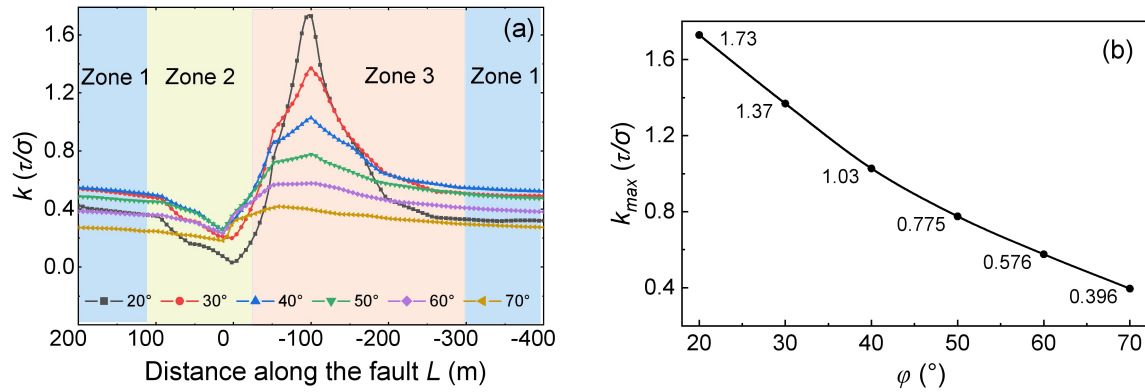
Fig. 2-5 Distribution of k along the fault with different \varphi when D_m = 0 m and r_b = 3 . (a) Distribution of k for \varphi from 20^\circ to 70^\circ at 10^\circ intervals. Zone 1 represents the initial area where no mining-induced stress disturbances occur. Zone 2 corresponds to an area where mining activities lead to an increase in fault stability. In contrast, Zone 3 denotes an area where mining operations result in a decrease in fault stability; (b) Variation of k_{\max} as a function of \varphi at L = -100 m. (Reproduced from Li et al., 2024a)
