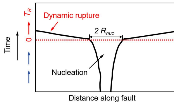
Fig. 5-2 A rupture nucleation model (adapted from Fig. 29 of Ohnaka and Shen, 1999). In this model, it is assumed that rupture initiates and propagates bidirectionally at a rapid rupture velocity starting from the critical time, t = 0 . The parameter 2 R_{nuc} represents the critical size of the nucleation zone, as defined in Eq. (4-6).
