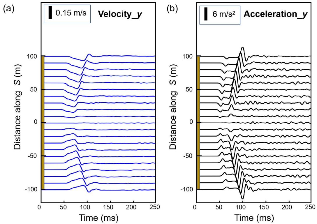
Fig.4-28 Velocity and acceleration in y components induced by fault rupture in Model_Cao. a and b show velocity and acceleration in y components, respectively. A total of 21 points were plotted along S at 10 m intervals from position D = 60 m.
