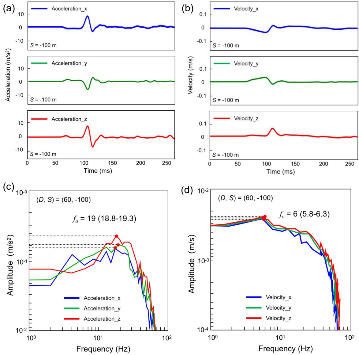
Fig. 4-30 Example of dominant frequency measurement via Fourier transform of time-domain seismic data: (a-b) Seismic data recorded at S = -100 m and D = 60 m in Model_Cao; (c-d) Corresponding Fourier transform of the time-domain data in (a) and (b), with a 30 Hz low-pass filter applied.
