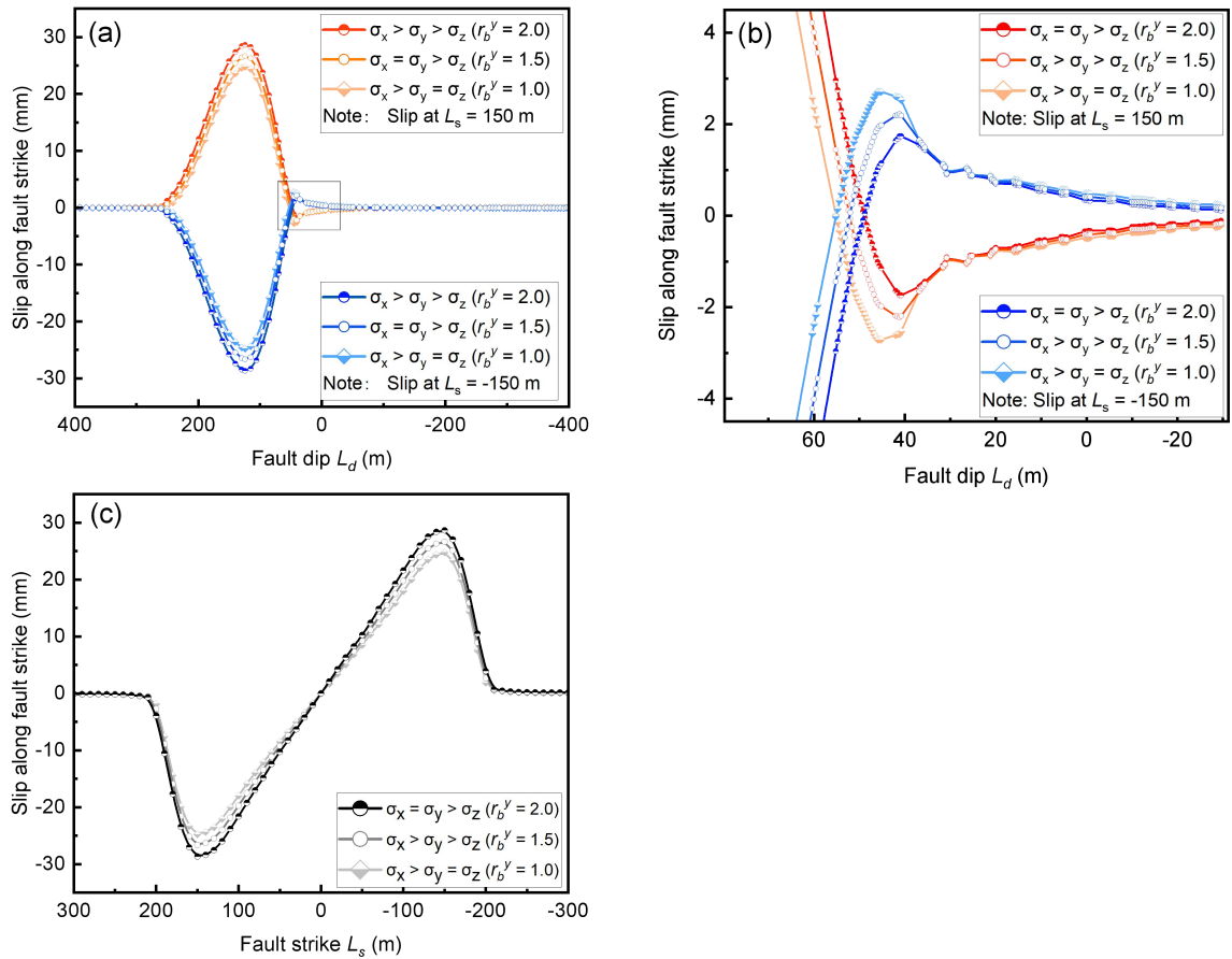
Fig. 3-9 The relationship between the coseismic slip components and the length of the fault strike direction with different intermediate far-field stress under the
