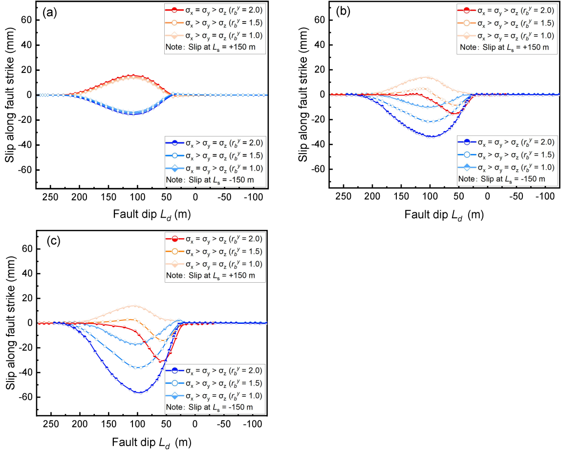
Fig. 3-11 Coseismic slip along the fault strike component with far-field stress rotating counterclockwise around the z -axis by (a) 0^\circ ; (b) 15^\circ ; and (c) 30^\circ , with intermediate far-field stress r_b^y values of 1.0, 1.5, and 2.0, W_m = 200 m, and D_m = -30 m.
