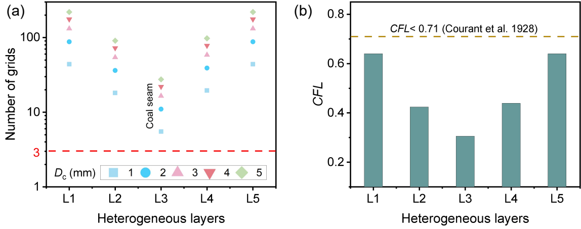
Fig. 4-7 Mesh size and time step setting. (a) Number of grids inside the cohesive zone under different layers and critical slip distance D_c . The heterogeneous layers are denoted as L1 to L5. (b) Time step setting according to the Courant-Friedrichs-Lewy (CFL) condition. CFL values are less than 0.71. As the results for L5 and L6 are identical, only the results up to L5 are displayed.
