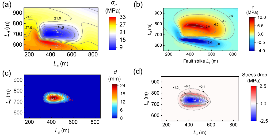
Fig. 4-10 Slip distribution and stress analysis on the fault plane for Model_Cai with D_m = 60 m, P_L = 280 m, and \mu = 0.628 . (a) 2-D spatial variation of \sigma_n ; (b) spatial variation of \tau ; (c) 2-D spatial variation of fault slip; (d) 2-D spatial variation of stress drop.
