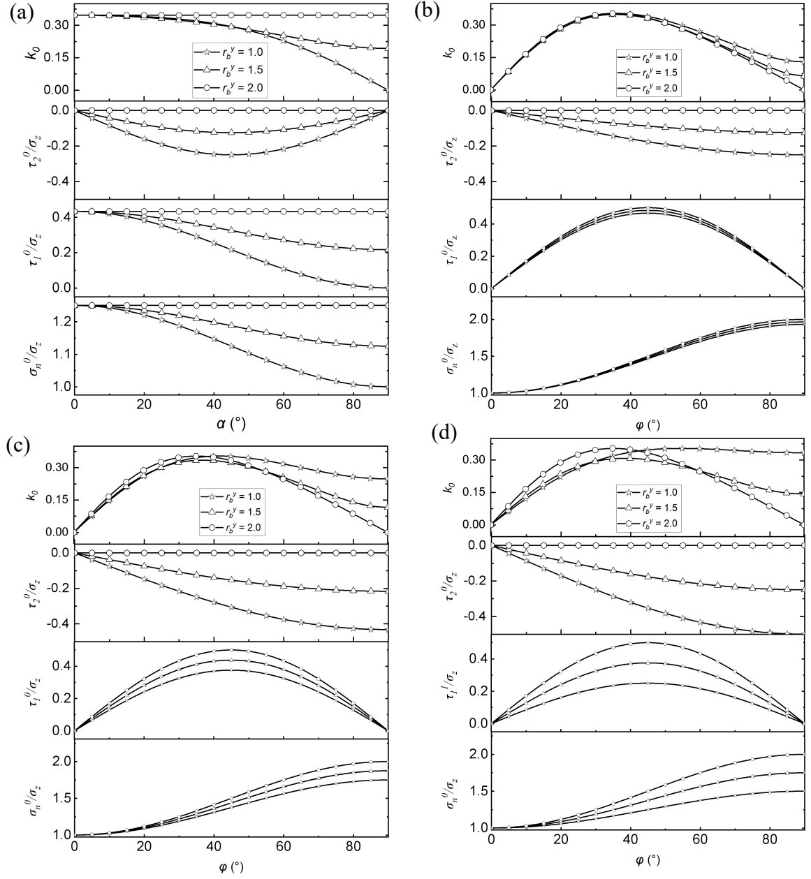
Fig. 3-3 The influence of fault dip angle ( \varphi ) and rotation of far-field stress ( \alpha ) (Fig. 3-1c) on the background stress ratio ( k_0 ). In the diagram presented, I plotted the stress values normalized by \sigma_z . (a) k_0 , s_n^0/s_z , t_1^0/s_z , and t_2^0/s_z as a function of \alpha with a fixed \varphi value of 30^\circ for the cases of r_b^\gamma = 1.0, 1.5 , and 2.0 ; (b) k_0 , s_n^0/s_z , t_1^0/s_z , and t_2^0/s_z as a function of \varphi for a fixed \alpha value of 15^\circ for the cases of r_b^\gamma = 1.0, 1.5 , and 2.0 ; (c) k_0 , s_n^0/s_z , t_1^0/s_z , and t_2^0/s_z as a function of \varphi for a fixed \alpha value of 30^\circ for the cases of r_b^\gamma = 1.0, 1.5 , and 2.0 ; (d) k_0 , s_n^0/s_z , t_1^0/s_z , and t_2^0/s_z as a function of \varphi for a
