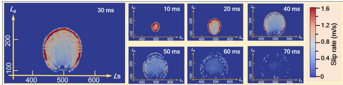
Fig. 4-14 Fault slip rate at 10 ms intervals in Model_Cao. In the subfigure showing the fault slip rate distribution at 10 ms, the red circle indicates the nucleation zone.
