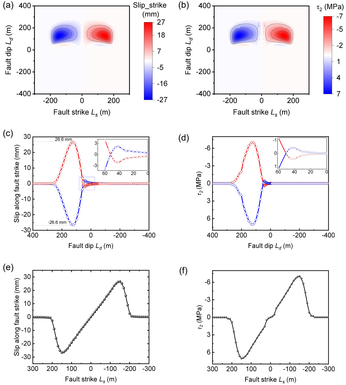
Fig. 3-7 Shear stress and slip components along the strike direction. (a) Slip component and (b) shear stress component. (c) Slip component and (d) stress components along dip for L_s = 150 m (red curve) and L_s = -150 m (blue curve); (e) Slip component and (f) shear stress components along strike for L_d = 150 m.
