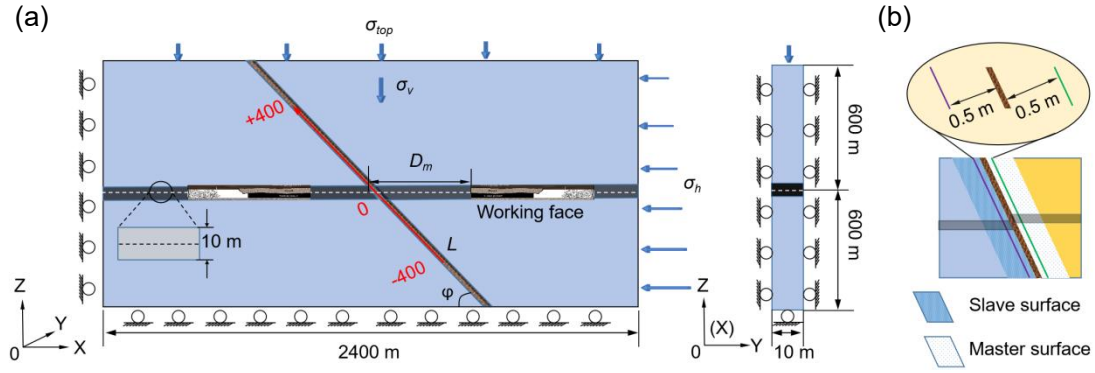
Fig. 2-1 A schematic illustration of the 2-D plane strain model, including the coal mining working face and the fault ahead of the working face. (a) The xyz -coordinate system is set as shown in the bottom left of the figure. The origin is located at the bottom left corner of the modeling region. \sigma_{top} is the \sigma_{zz} stress at the top of the model that simulates overburden weight. \sigma_v is vertical principal stress. \sigma_h is horizontal principal stress in the x -direction. On the left and bottom sides of the model, the displacement boundary condition is applied as described in the text. \varphi stands for fault dip angle. The local coordinate (red line) L is set along the fault, being the origin is at the center of the coal seam, and the positive direction of L is taken upward. D_m is the mining distance measured from the origin of the local coordinate L to the working face, taken positive at the hanging wall side. The thickness of the coal seam is 10 m. (b) Master and slave surfaces are applied to the model. The green line, located 0.5 m from the fault, represents the measurement line, along which \tau , \sigma_n , and coseismic slip are measured on the hanging wall side. Similarly, the purple line, positioned 0.5 m away from the fault, represents the measurement line on the footwall side. (Reproduced from Li et al., 2024a)
