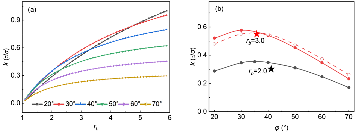
Fig. 2-2 Distribution of k as a function of r_b and \varphi . (a) Distributions of k , as a function of r_b when \varphi is 20°, 30°, 40°, 50°, 60°, and 70°. (b) Distributions of k as a function of \varphi for the cases where r_b = 2 and 3. Red and black stars represent the maximum value of k ( k_{\max} ). The dashed line with open circles represents the distributions of k at L = 200 m (Fig. 2-5a), as a function of \varphi . (Reproduced from Li et al., 2024a)
