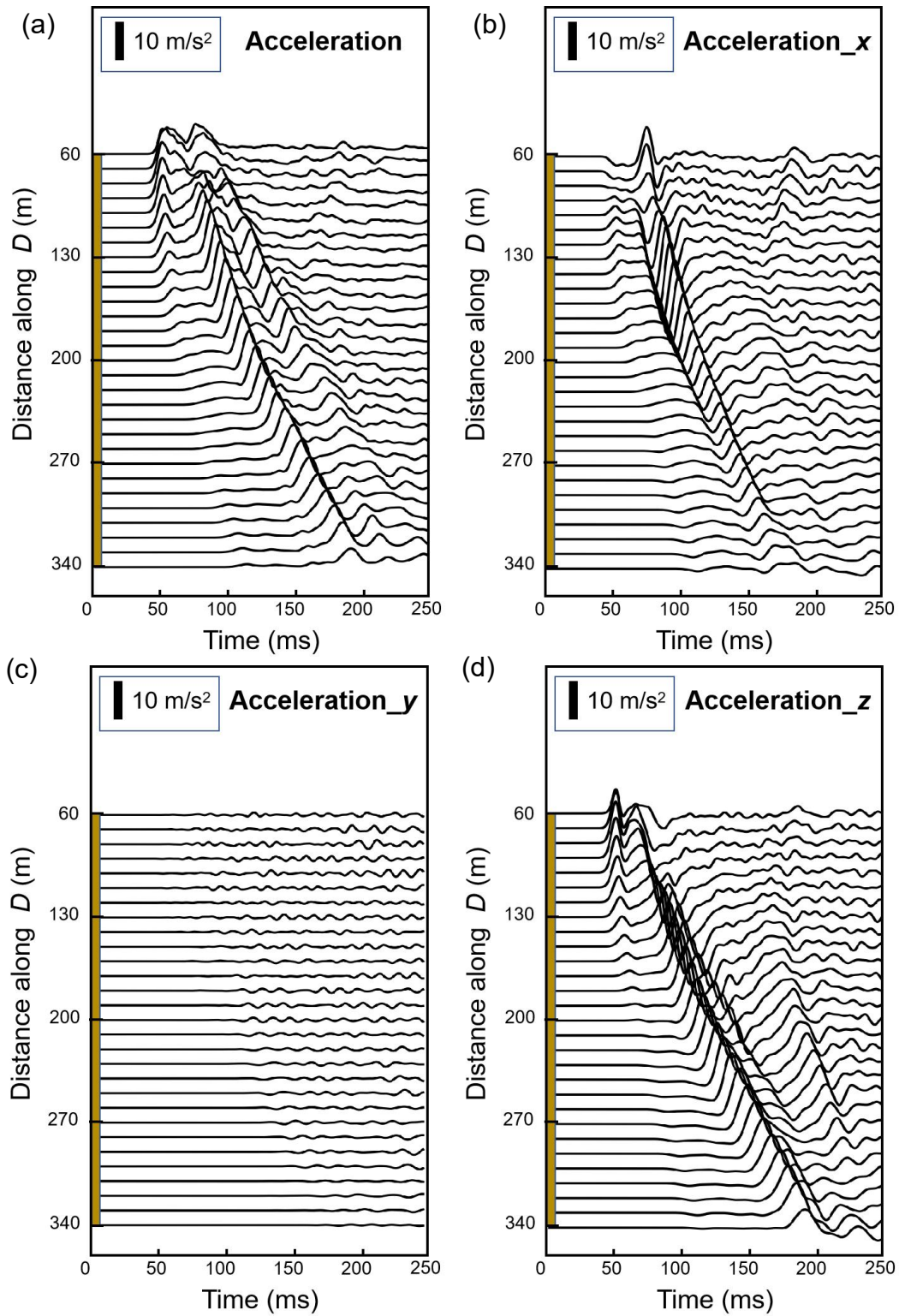
Fig. 4-25 Acceleration at 1 m above roof induced by fault rupture in Model_Cao. a–d correspond to acceleration and the x , y , and z components, respectively. A total of 29 points were plotted along D at 10 m intervals from the position S = 0 m.
