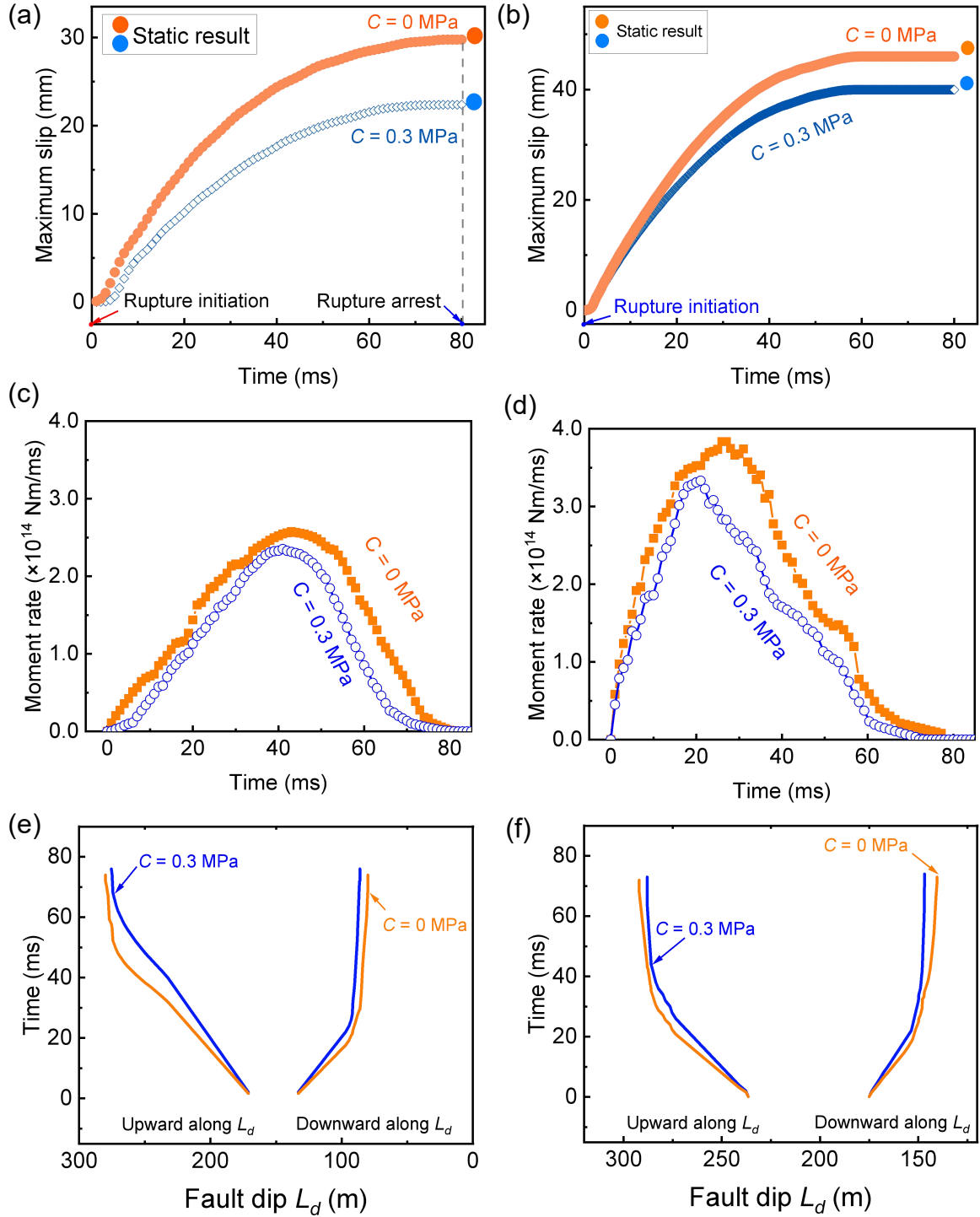
Fig. 4-32 Cohesive effects on dynamic rupture. (a) Maximum slip in Model_Cao (b) Maximum slip in Model_Cai. (c) Moment rate function in Model_Cao. (d) Moment rate function in Model_Cai. (e) Rupture front arrival along the fault dip for in Model_Cao at L_s = 500 m; (f) Rupture front arrival along the fault dip in Model_Cai at L_s = 420 m. Orange and blue dots represent static results for cohesive values of 0 MPa and 0.3 MPa. The measurement point for maximum slip in (a) is located at (L_s, L_d) = (500, 158) , and in (b), it is at (420, 220) .
