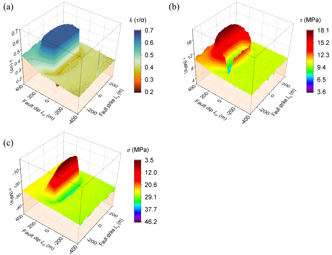
Fig. 3-5 Mining-induced stress and k distribution on the fault plane, considering the parameters r_b^y = 1.5 , D_m = -30 m, and W_m = 400 m. (a) The spatial distribution of k ; (b) The spatial distribution of \tau ; (c) The spatial distribution of \sigma .
