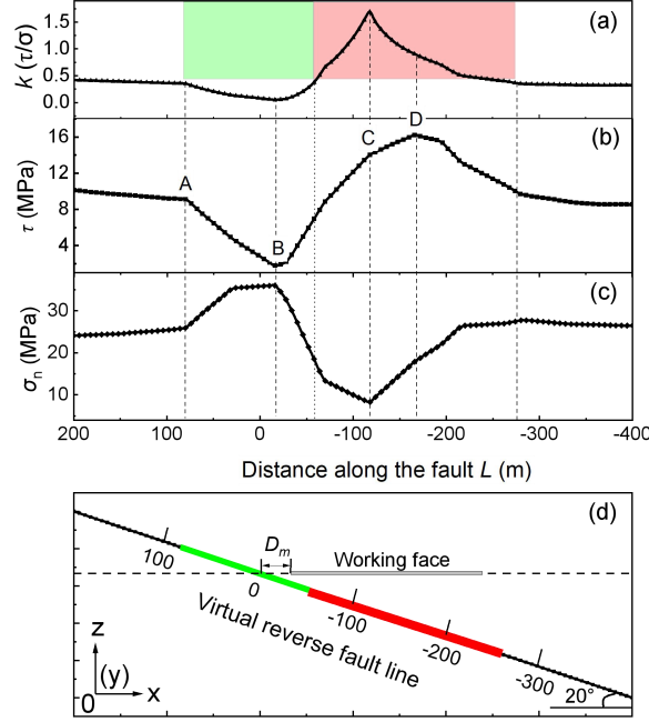
Fig. 2-3 Mining-induced stress distribution along the fault when D_m = 20 m, r_b = 3 , and \varphi = 20^\circ . (a) distribution of k , (b) distribution of \tau , and (c) distribution of \sigma_n along the fault. (d) The geometry between the fault (black, green, and red lines) and the working face (gray solid horizontal line). Green and red areas/lines in (a) and (b) stand for where k decreases and increases due to mining activity, respectively. (Reproduced from Li et al., 2024a)
