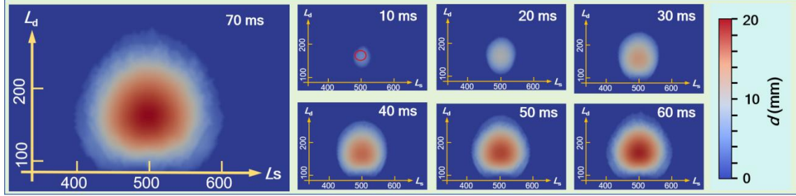
Fig. 4-13 Fault slip distribution at 10 ms intervals in Model_Cao. In the subfigure showing the fault slip distribution at 10 ms, the red circle indicates the nucleation zone.
