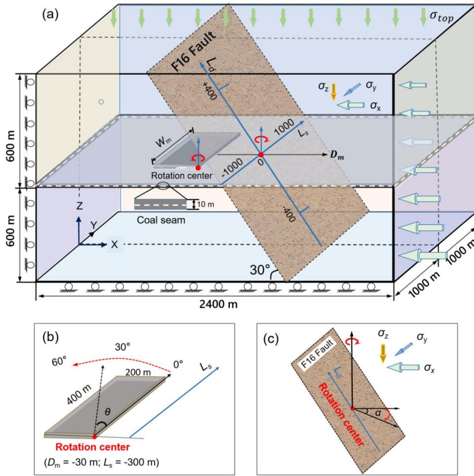
Fig. 3-1 A schematic illustration of the 3-D mining model. (a) Configuration of the deep mining model with a central reverse fault. The direction of the xyz -coordinate system is situated at the bottom left corner of the figure. L_s and L_d represent local coordinates along the fault strike and dip directions, respectively. These coordinates are set to 0 at the cross-section where the mining level intersects the fault at y = 0 . W_m is the length of the panel. D_m represents the mining distance, with the positive direction indicating the hanging wall side and the negative direction indicating the footwall side. Vertical far-field stress is denoted as \sigma_z , and horizontal far-field stresses in the x - and y -directions are denoted as \sigma_x and \sigma_y , respectively; (b) Schematic diagram of the panel rotation angle, where the ‘rotation center’ denotes the commencement of rotation. Rotation starts from a position parallel to the local coordinate L_s at 0^\circ , with the angle increasing in a counterclockwise direction; (c) Diagram illustrating the principal stress rotation
