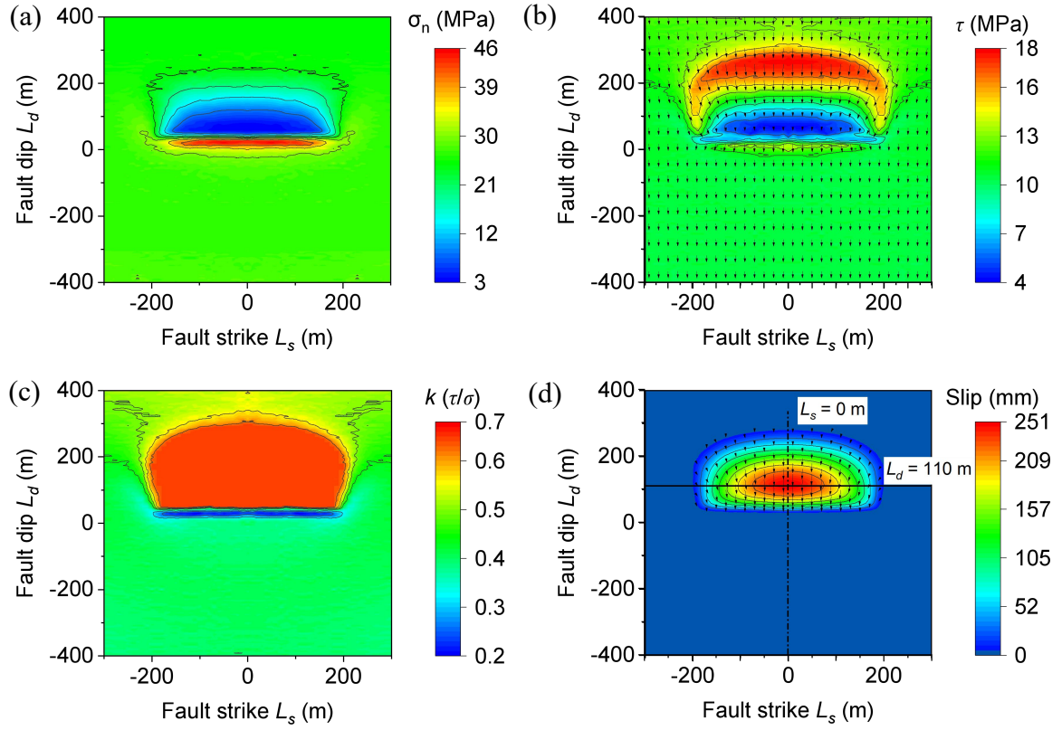
Fig. 3-4 Mining-induced slip and stress distribution on the fault plane, considering the parameters r_b^y = 1.5 , D_m = -30 m, and W_m = 400 m. (a) The spatial distribution of \sigma_n ; (b) The spatial distribution of \tau . The black arrow indicates the size and direction of \tau on the fault; (c) The spatial distribution of k ; (d) The spatial distribution of slip. The black arrow indicates the size and direction of the total slip on the fault.
