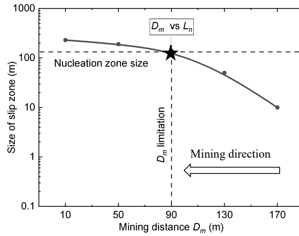
Fig. 2-9 The relation between the coseismic slip zone size and D_m (see Table 2-3). The nucleation zone size of 138 m (broken horizontal line) is assumed under the condition that \mu_s - \mu_d = 0.1 , D_c = 0.03 m, and the average normal stress is 20 MPa. The solid star indicates the location of the limit line of D_m . (Reproduced from Li et al., 2024a)
