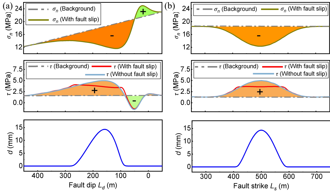
Fig. 4-11 Faulting in deep mining driven by increased shear stress and decreased normal stress. (a) Mining-induced changes in \sigma_n , \tau , and d along L_d specific focus at L_s = 500 m. (b) Mining-induced changes in \sigma_n , \tau , and d along L_s with specific focus at L_d = 158 m. In subfigure \sigma_n , orange represents mining-induced \sigma_n release, while green represents \sigma_n accumulation. In subfigure \tau , orange indicates areas of mining-induced \tau accumulation, while green indicates \tau release. The dashed lines represent the distribution under pure background stress conditions, without the
