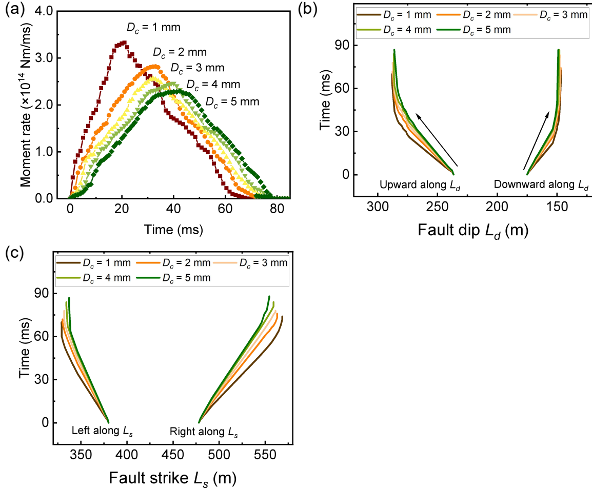
Fig. 4-31 Influence of D_c on dynamic rupture. (a) Moment rate function. (b) Rupture front arrival along L_d for various D_c at L_s = 420 m; (c) Rupture front arrival along L_s for various D_c at L_d = 220 m.
