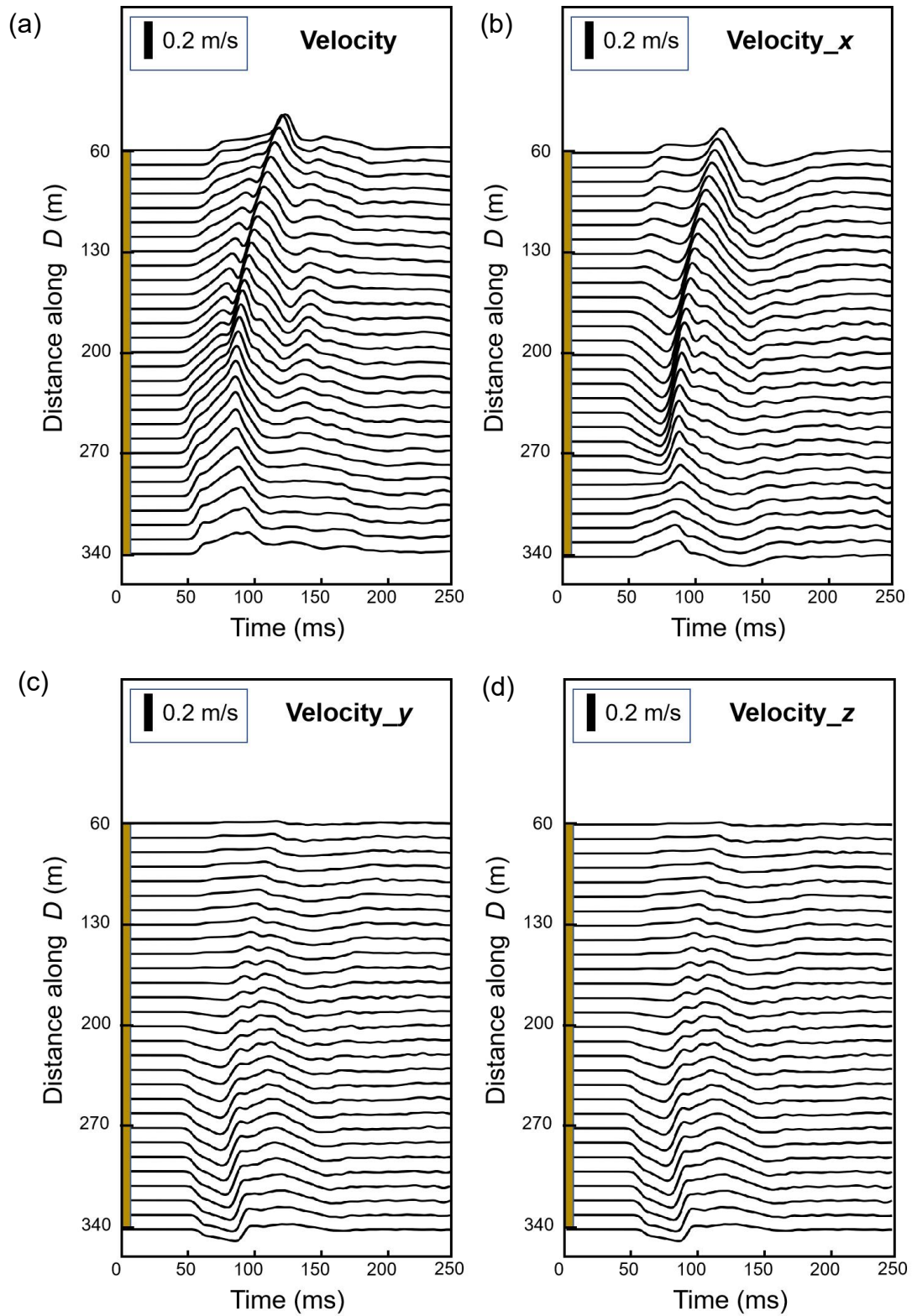
Fig.4-26 Velocity at 1 m above roof induced by fault rupture in Model_Cai. a–d correspond to velocity and the x , y , and z components, respectively. A total of 29 points were plotted along D at 10 m intervals from the position S = 0 m.
