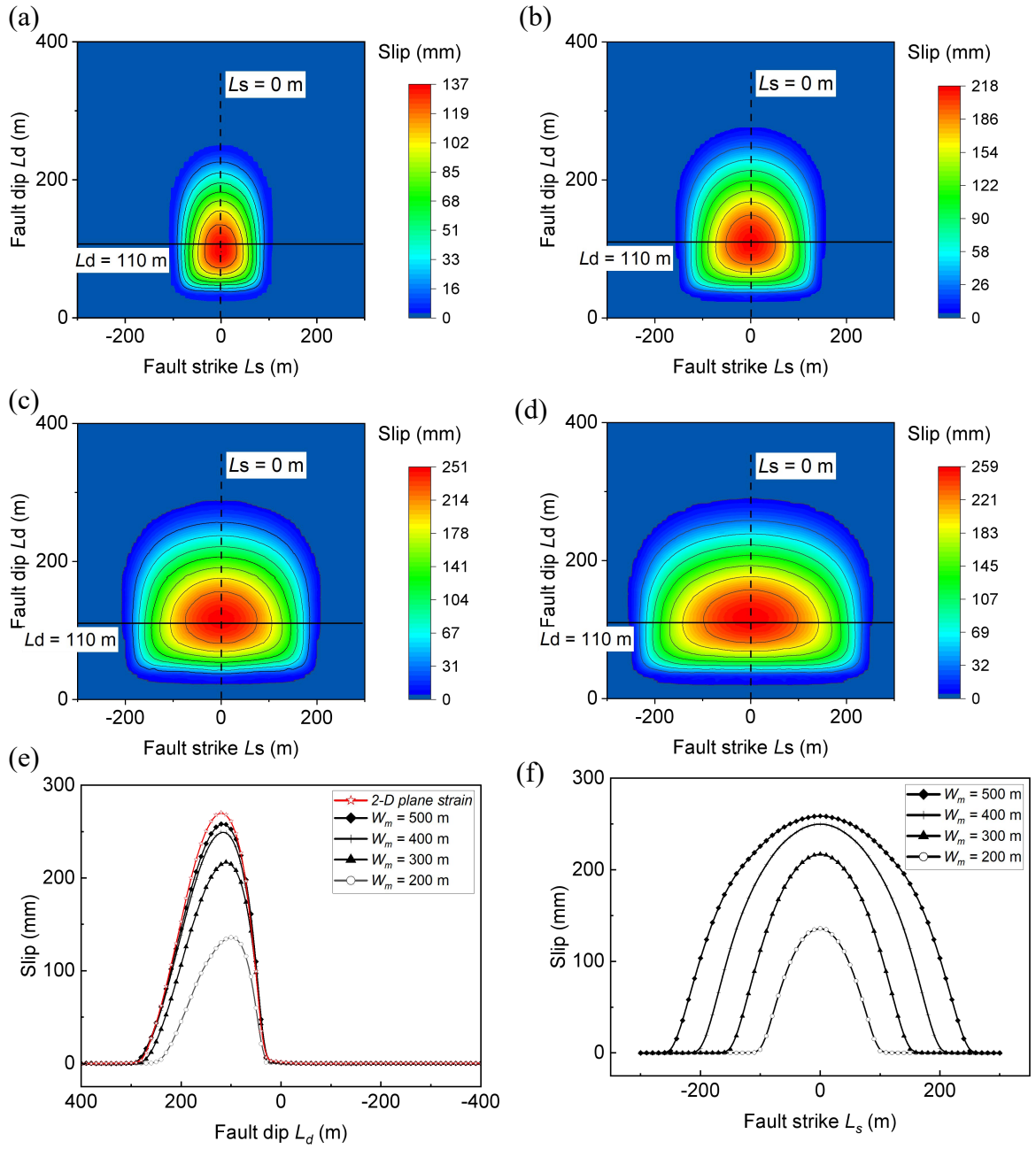
Fig. 3-12 The distribution of fault slip investigated under the influence of varying panel lengths, ranging from W_m = 200 m to W_m = 500 m at intervals of 100 m with D_m = -30 m and \mu_s = 0.7 . (a) Fault slip distribution for a panel length of W_m = 200 m; (b) for W_m = 300 m; (c) for W_m = 400 m; and (d) for W_m = 500 m; (e) Fault slip curves at L_s = 0 m along the fault dip direction; (f) Fault slip curves at L_d = 110 m along the fault strike direction.
