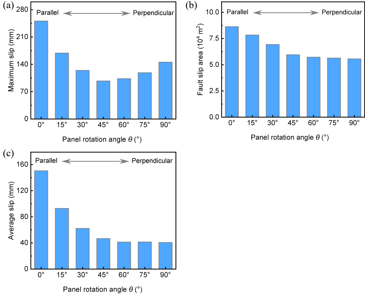
Fig. 3-14 Fault coseismic slip, as the panel rotates counterclockwise along the fault strike from 0^\circ to 90^\circ , with increments of 15^\circ , under conditions of r_b^y = 1.5 , W_m = 400 \text{ m} , and D_m = -30 \text{ m} . (a) Maximum slip; (b) Fault slip area; (c) Average slip.
