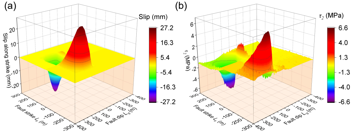
Fig. 3-8 Shear stress and slip components along the fault strike direction in 3-D plots: (a) Slip components along the fault strike direction on the fault plane; (b) Shear components along the fault strike direction on the fault plane.
