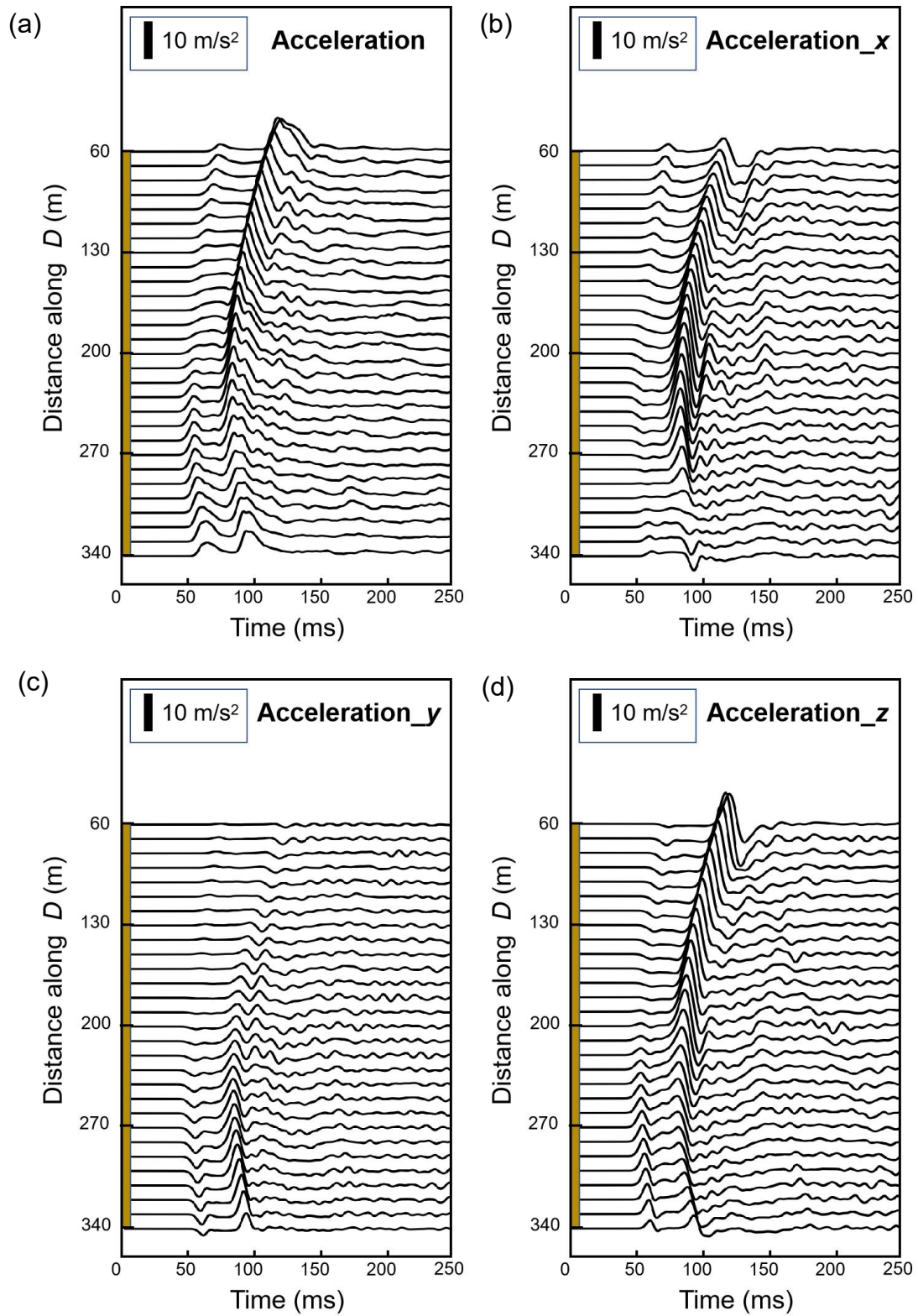
Fig.4-27 Acceleration at 1 m above roof induced by fault rupture in Model_Cai. a–d correspond to acceleration and the x , y , and z components, respectively. A total of 29 points were plotted along D at 10 m intervals from the position S = 0 m.
