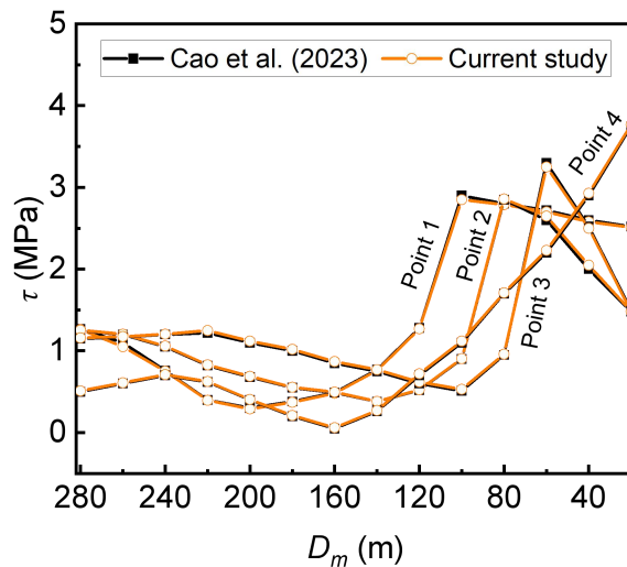
Fig. 4-9 Variation in shear stress with decreasing D_m from 280 m to 20 m at L_s = 500 m.
