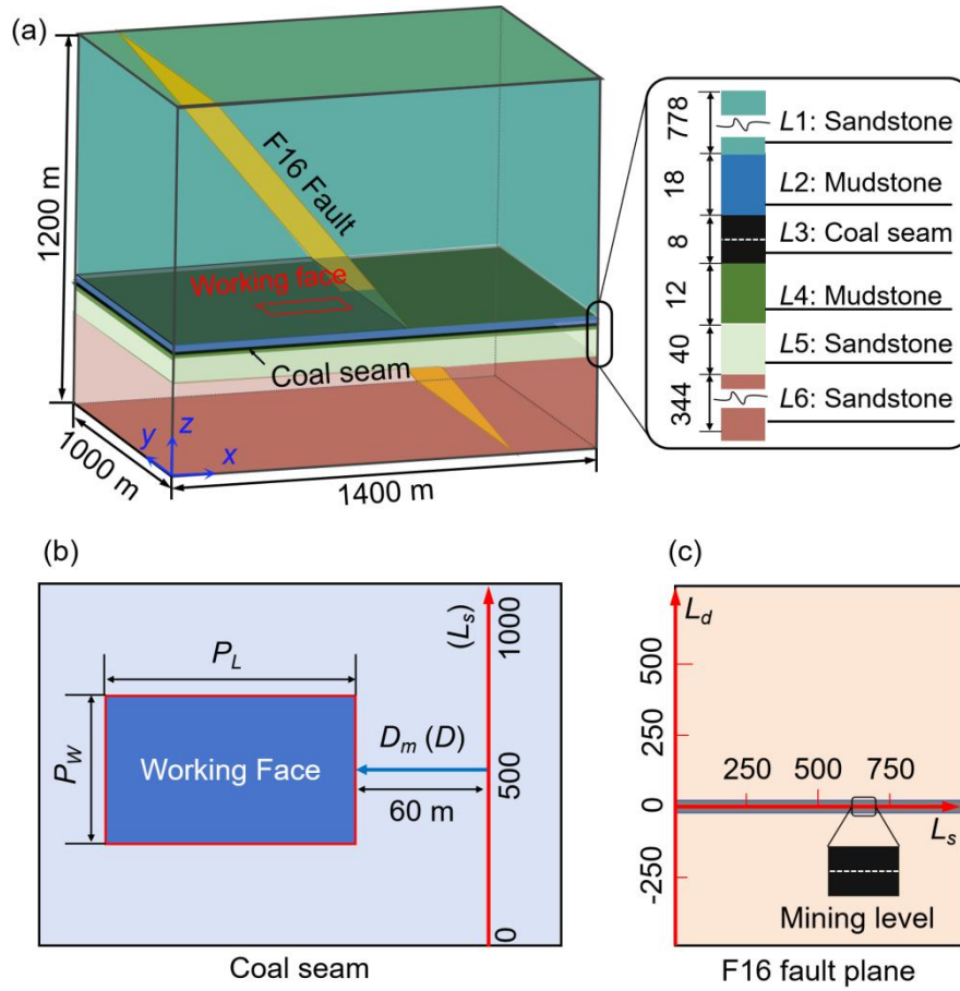
Fig. 4-2 3-D structural model (Model_Cao) based on Cao et al. (2023b). (a) Geometry of the 3-D model simulating mining-induced faulting and earthquake. L1 - L6 represents different geological layers in the 3-D structural model, with L1 being the surface layer and L6 the deepest layer. (b) Local coordinate system on the working face. P_L is the panel length, P_W is the panel width, D_m is the mining distance, and L_s is the distance along the fault strike direction. (c) Local coordinate system on the fault plane. L_s represents the length along the fault strike direction, starting from the origin at the intersection of the fault plane and the working face, located on the left side at y = 0 , and extending horizontally in the positive y -direction. L_d represents the length along the fault dip direction, starting from the same origin and extending upwards, with positive values in the upward direction along the fault plane.
