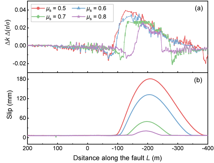
Fig. 2-7 Distribution of (a) \Delta k and (b) coseismic slip along the fault for different \mu_s from 0.5 to 0.8 under the condition of r_b = 2 , D_m = 90 m, and \varphi = 30^\circ . (Reproduced from Li et al., 2024a)
