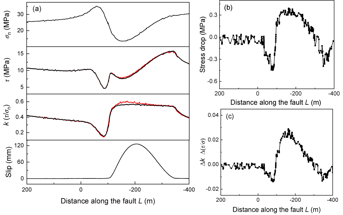
Fig. 2-6 Distributions of \sigma_n , \tau , k , and coseismic slip along the fault under the condition of D_m = 90 m, \mu_s = 0.55 , and \varphi = 30^\circ . (a) Distributions of \sigma_n , \tau , and k on the hanging wall and footwall, respectively. The red curves represent \tau and k at the hanging wall side, and the black curves represent \tau and k at the footwall side. The bottom trace is the distribution of coseismic slip on the fault. (b) Stress drop distribution in \tau of Fig. 2-6a. c \Delta k distribution in k of Fig. 2-6a. (Reproduced from Li et al., 2024a)
