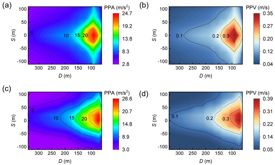
Fig. 4-29 PPA and PPV distribution on the roof: (a–b) PPA and PPV for Model_Cao; (c–d) PPA and PPV for Model_Cai.
