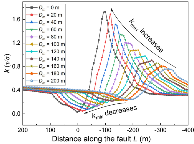
Fig. 2-4 The distribution of k along the fault as a function of distance along the fault. Different color corresponds to different D_m when r_b = 3 and \varphi = 20^\circ . (Reproduced from Li et al., 2024a)
