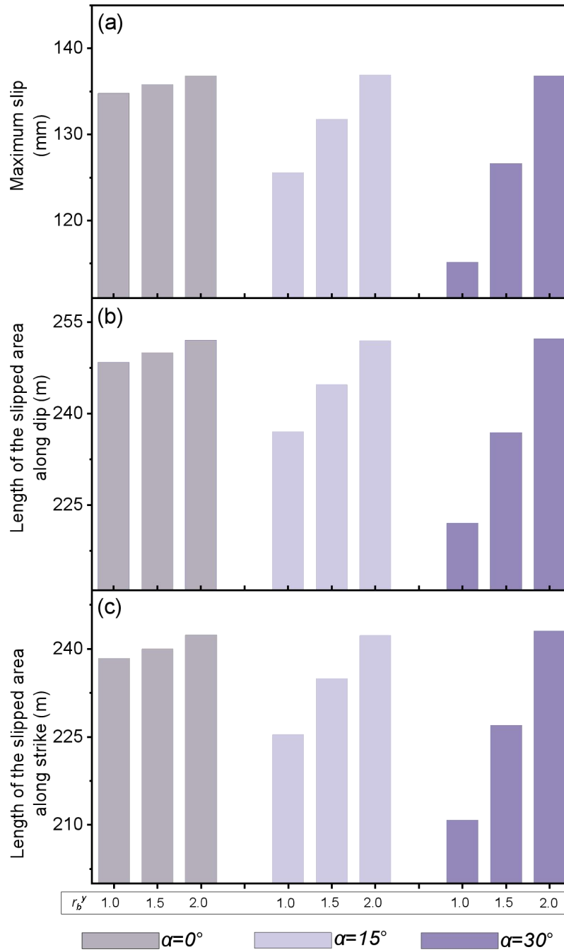
Fig. 3-10 Coseismic slip with far-field stress rotating counterclockwise around the z -axis by 0^\circ , 15^\circ , and 30^\circ , with intermediate far-field stress r_b^y values of 1.0, 1.5, and 2.0, W_m = 200 m, and D_m = -30 m. (a) Maximum slip; (b) Length of the slipped area
