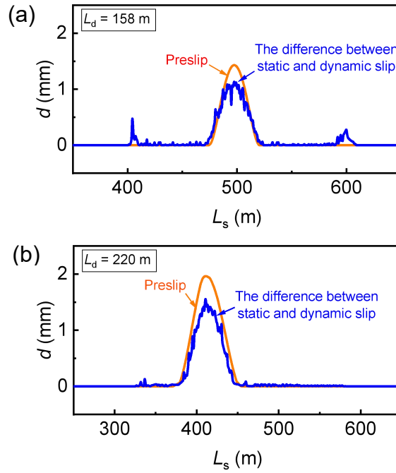
Fig. 4-20 Comparison of preslip with the difference between static and dynamic slip: (a) Model_Cai; (b) Model_Cao.
