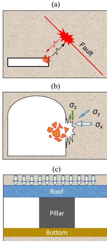
Fig. 1-1 Schematic illustration of rockburst in deep mining. (a) fault-slip rockburst; (b) Strain rockburst; (c) Pillar rockburst. Modified after Cai et al. (2021), Chen et al. (2024), and Ortlepp and Stacey (1994).
