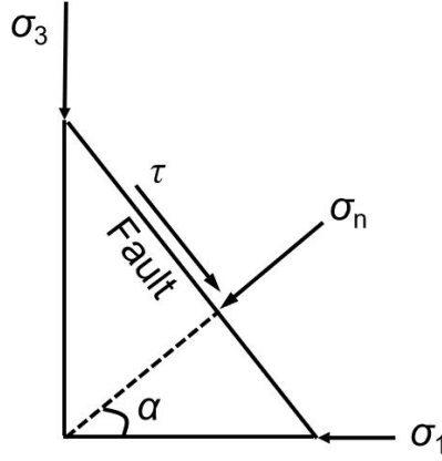
Fig. 4-4 Plane of weakness with outward normal vector oriented at angle \alpha to the direction of \sigma_1 .
