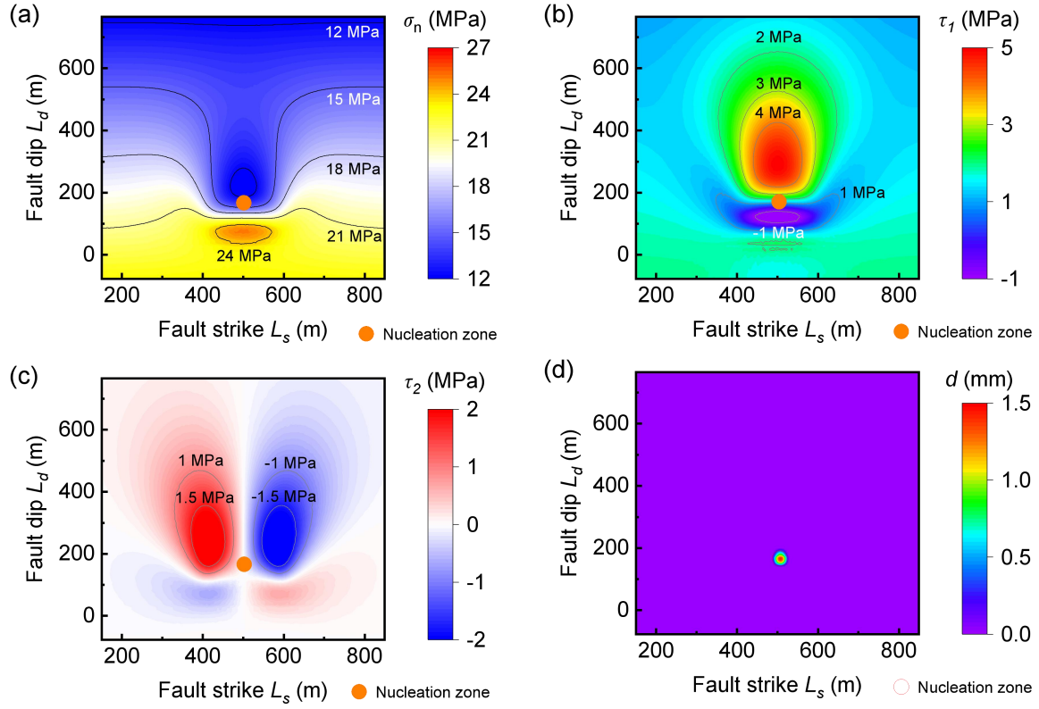
Fig. 4-6 Initial stress distribution for dynamic rupture calculation in Model_Cao, with D_m = 60 m, and \mu_s = 0.375 . (a) \sigma_n distribution, (b) Shear stress, \tau_1 , distribution along dip direction ( L_d ), (c) Shear stress, \tau_2 , distribution along strike direction ( L_s ). (d) Static slip with \mu_s = 0.375 . The orange circular region in the figure represents the designated nucleation zone, calculated based on Eq. 4-6.
