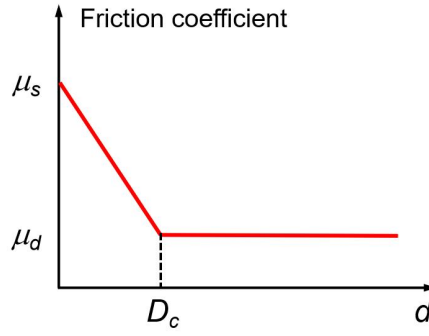
Fig. 4-5 Conceptual diagram of the slip-weakening friction model: \mu_s and \mu_d represent yield and residual friction coefficients, D_c indicates critical slip distance.
