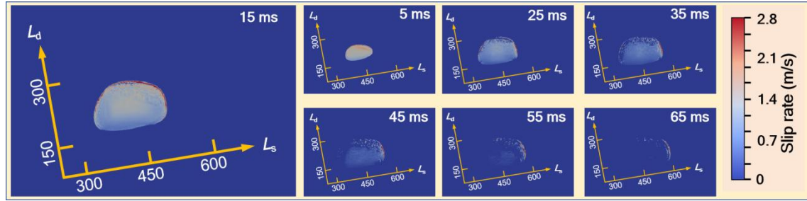
Fig. 4-17 Fault slip rate at 10 ms intervals in Model_Cai.
