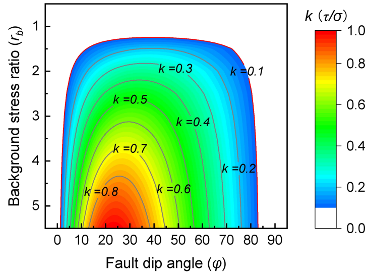
Fig. 5-1 Relationship between fault stress ratio, background stress ratio ( r_b = \sigma_1/\sigma_3 ), and fault dip angle ( \varphi ), under far-field (background stress) conditions. This figure integrates the results from Fig. 2-2 in Chapter 2, presenting a \varphi - r_b plane distribution of k , where both the horizontal axis ( \varphi ) and the vertical axis ( r_b ) are treated as variables. Note that this analysis focuses exclusively on the reverse faulting regime, where r_b > 1.0 .
