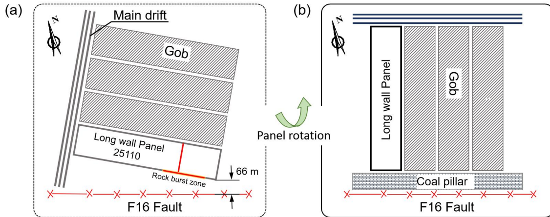
Fig. 3-15 Schematic diagram of direction adjustment layout of the panels. (a) Layout of mining panels and rock burst events at Yuejin Coal Mine; (b) Reconfiguring panel layout: from nearly parallel to perpendicular to the fault strike. The orange and red lines in Longwall panel 25110 in (a) show the rock burst event and the corresponding mining line at the time of the incident, respectively. This figure is drawn based on Li et al. (2014) and Cai et al. (2021).
