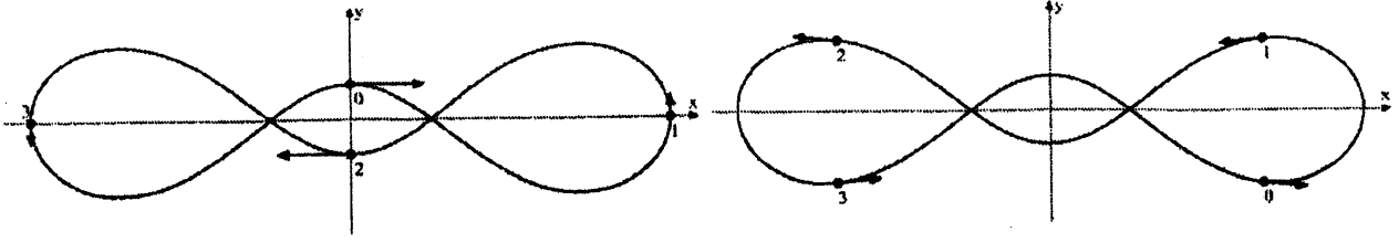
Figure 4: Motion of the Super-Eight \dots \rightarrow \text{Rhomboidal} \rightarrow \text{Collinear} \rightarrow \text{Rectangular} \rightarrow \text{Collinear} \rightarrow \dots
