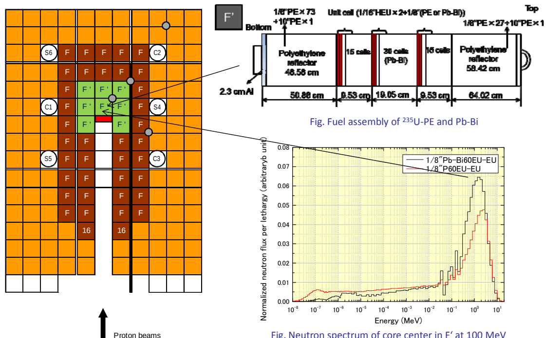
Fig. Core configuration of ^{235}\text{U} and Pb-Bi zoned core
