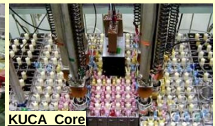
KUCA Core
