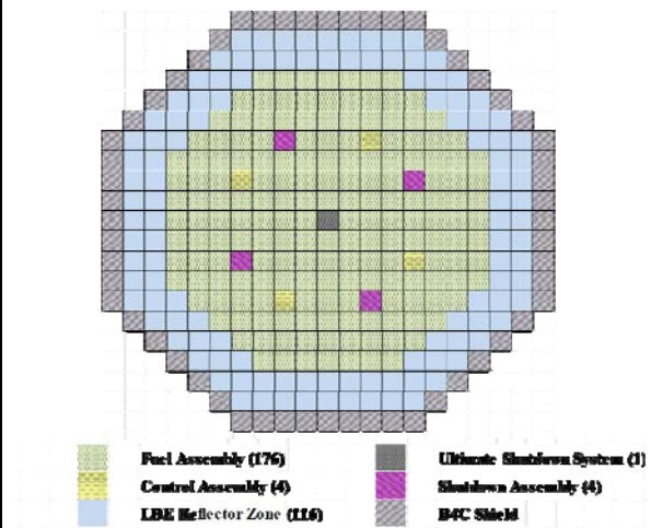
Fig 1. TORIA core model
