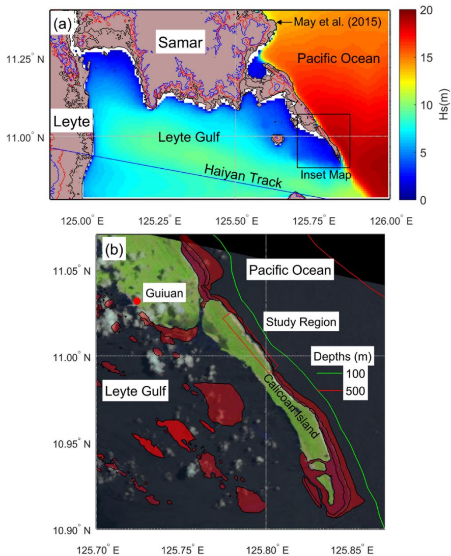
645 Figure 1. Typhoon Haiyan and study region on Calicoan Island. (a) Overview map showing 646 Haiyan Track, (10, 50, 100) meter elevation contours, and hindcast wave heights; (b) Inset map of 647 study region on Calicoan Island, depth contours, and coral reef locations in red. Background 648 image from Landsat May 2, 2014.
