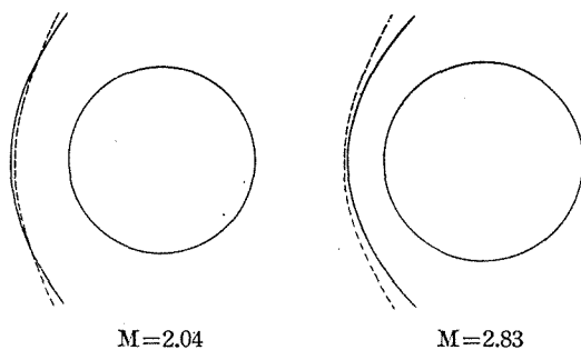
Fig. 3. Case of a circular cylinder.
