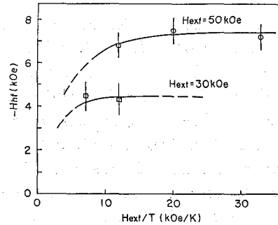
Fig. 6. Hyperfine field of ^{57}\text{Fe} in Tc from Mössbauer experiments as a function of H_{\text{ext}}/T , where the external field H_{\text{ext}}=30 and 50 kOe, and temperature is 1.5 < T < 4.2 K.
