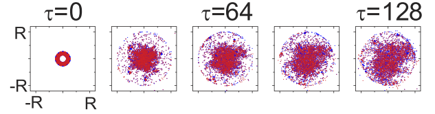
FIG. 5 (color online). Time evolution of the positive temperature system is plotted. The values of the parameters are N = 6920 , n_c = 20 , R_c = 0.2R , r_c = 0.07R , \tau_c = 9.3 , and E = 24.1 (= E_2) . Because the clumps overlap each other, we see only the outline of the clumps (hollow ring) at \tau = 0 .
