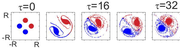
FIG. 4 (color online). Time evolution of the negative temperature system is plotted. The values of the parameters are N = 6724 , n_c = 4 , R_c = 0.5R , r_c = 0.2R , \tau_c = 15.6 , and E = 2.69 \times 10^4 (= E_1) .
